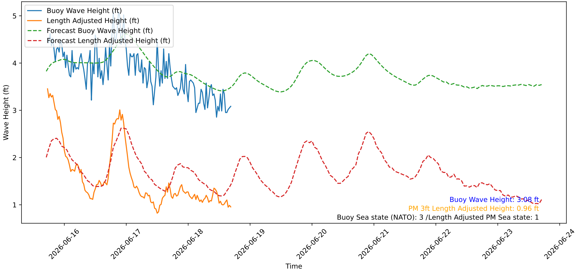
Wave Heights over Time for Green Beach at 2026-06-18 17:21:09
