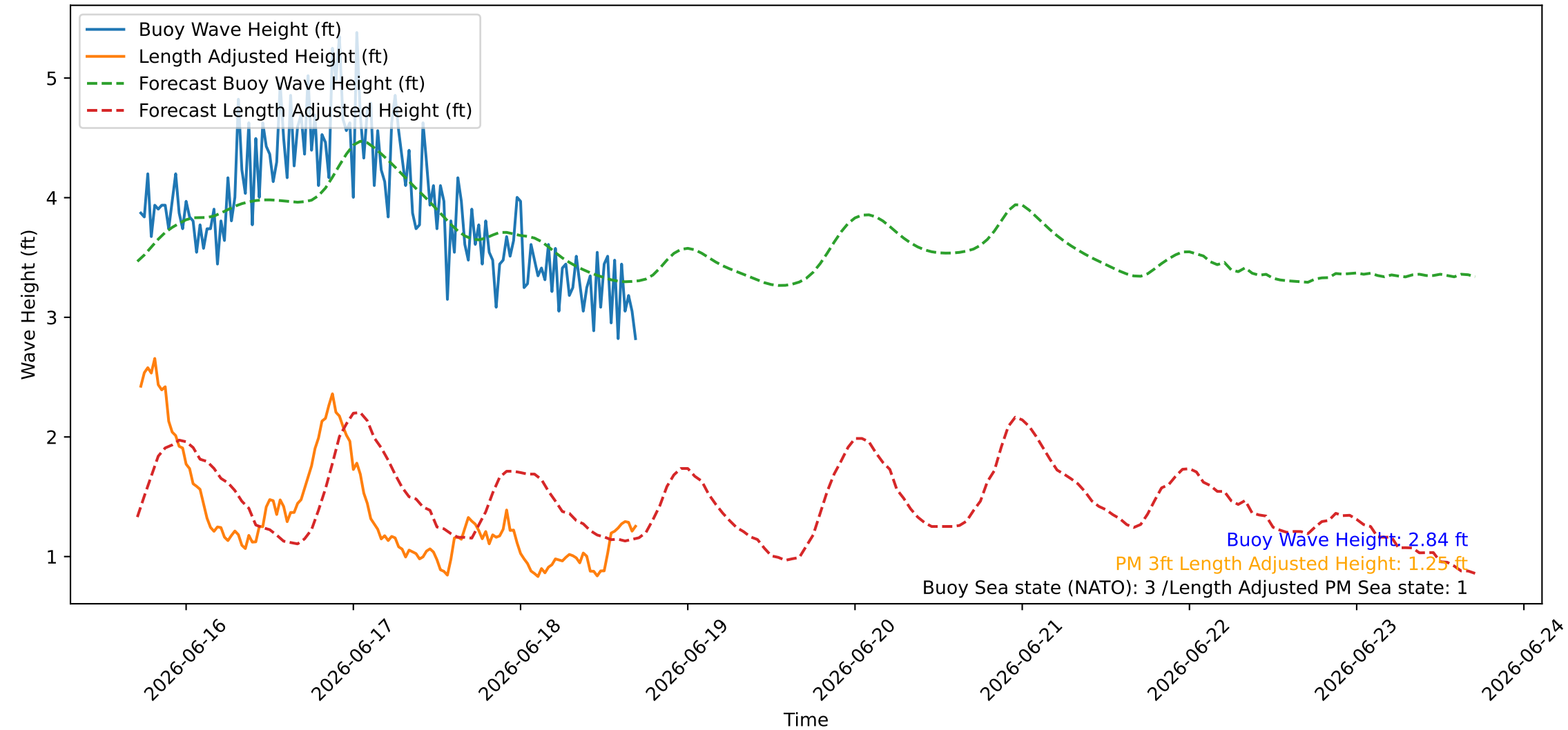
Wave Heights over Time for Red Beach at 2026-06-18 17:20:47
