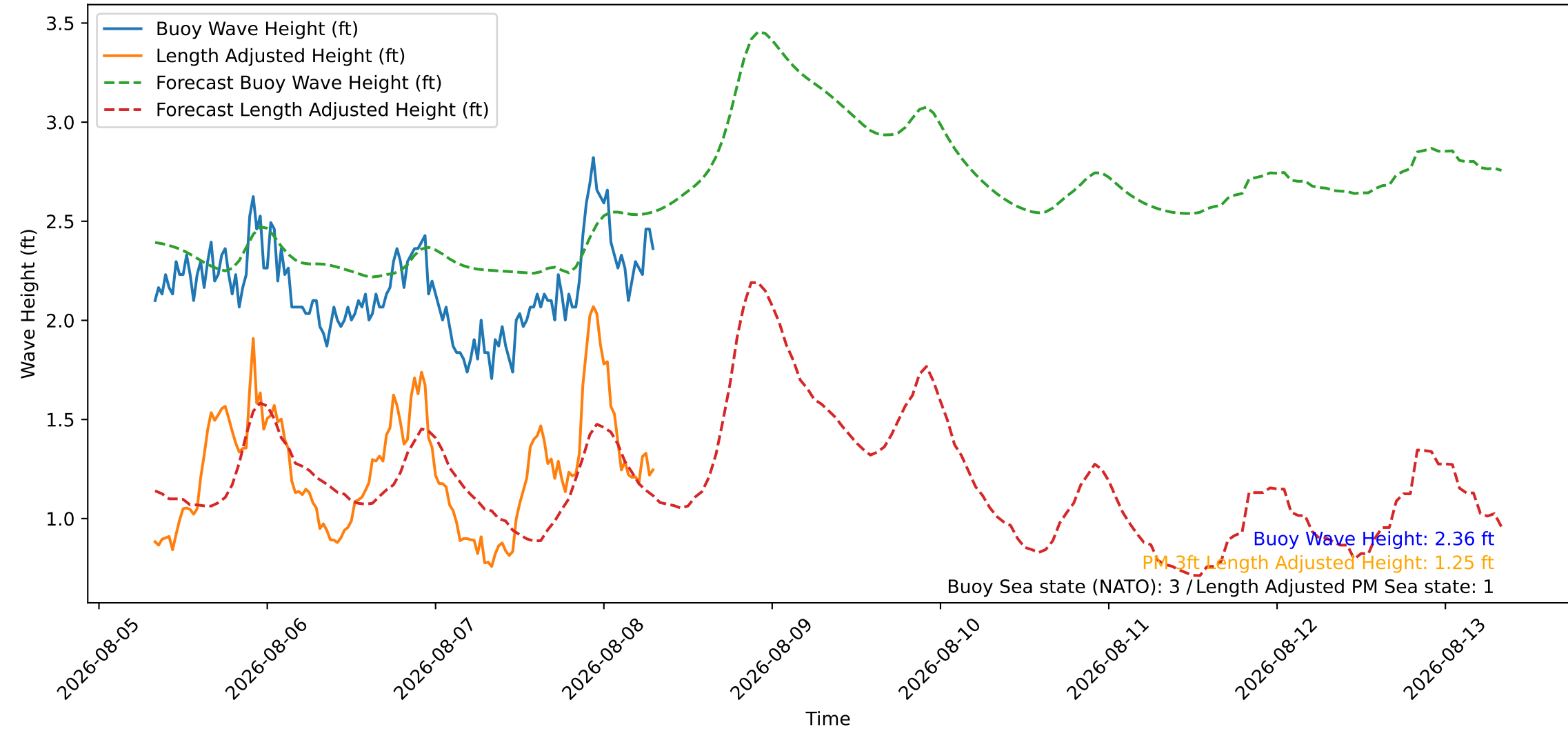
Wave Heights over Time for Green Beach at 2026-08-08 08:01:08
