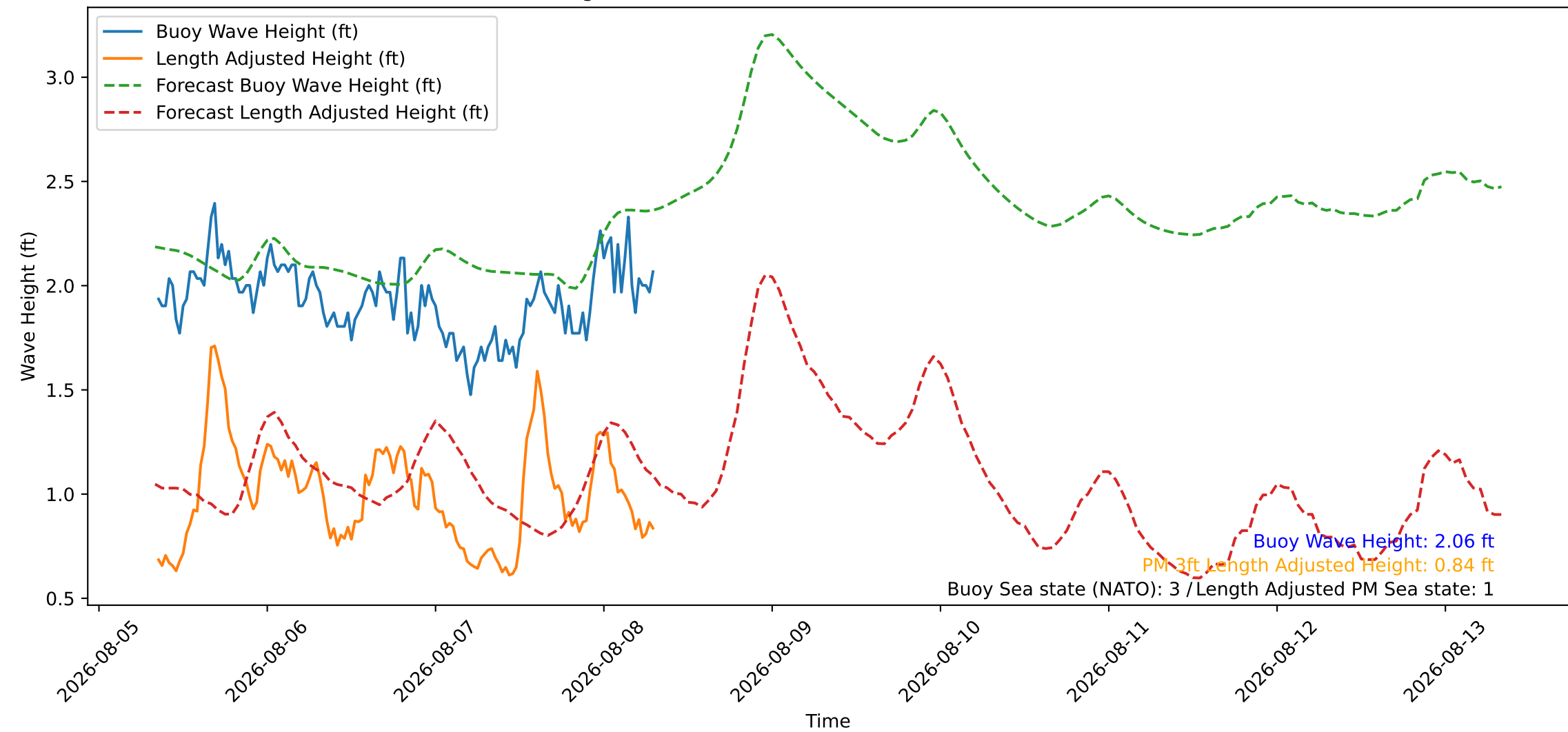
Wave Heights over Time for Red Beach at 2026-08-08 08:00:46
