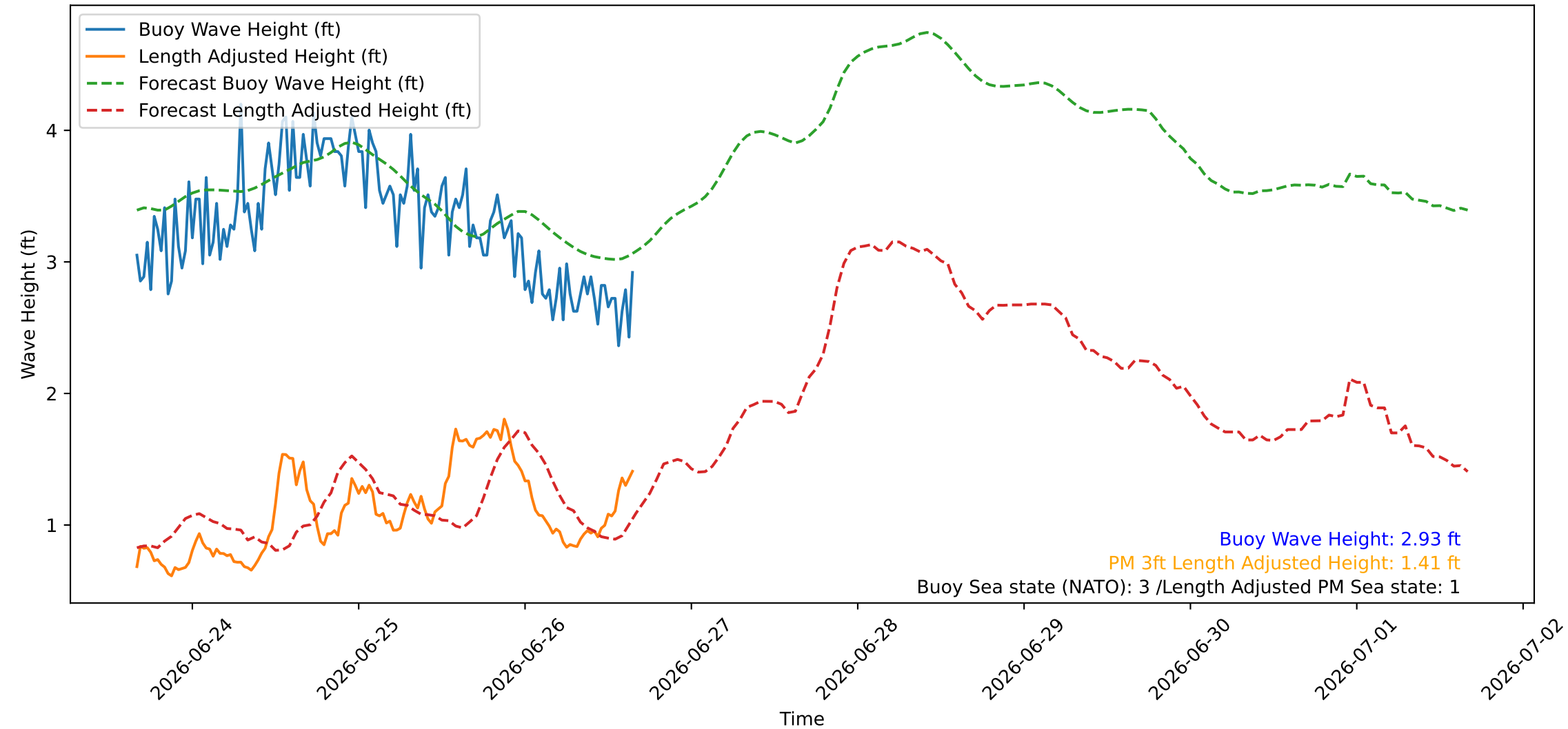
Wave Heights over Time for Green Beach at 2026-06-26 16:11:07
