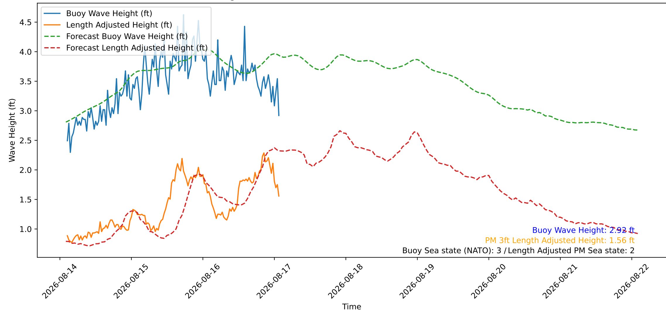
Wave Heights over Time for Oceanside Harbor at 2026-08-17 02:20:27
