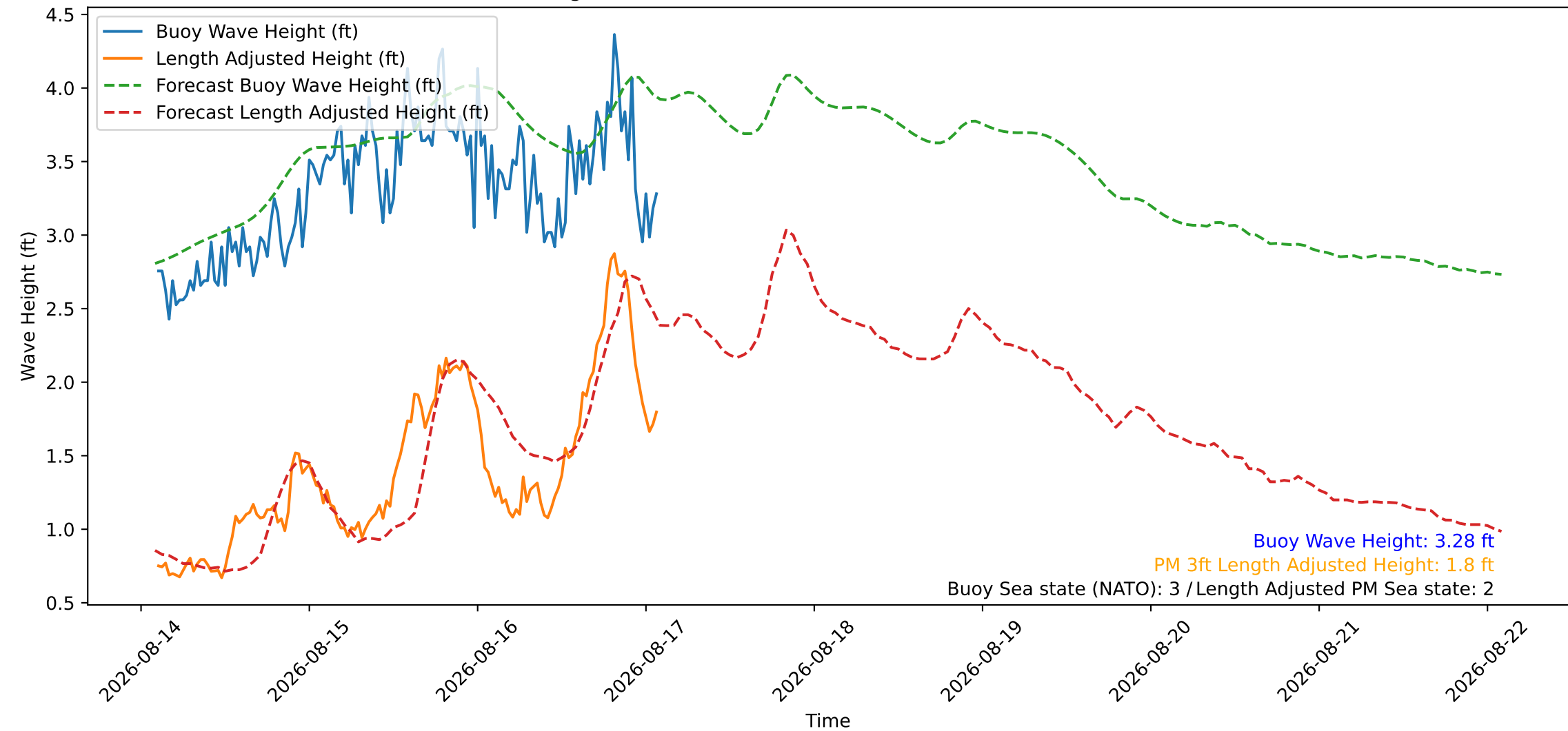
Wave Heights over Time for Green Beach at 2026-08-17 02:21:12
