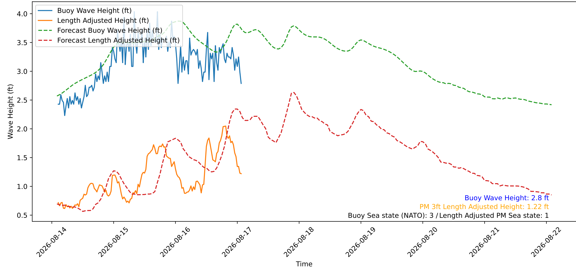
Wave Heights over Time for Red Beach at 2026-08-17 02:20:48
