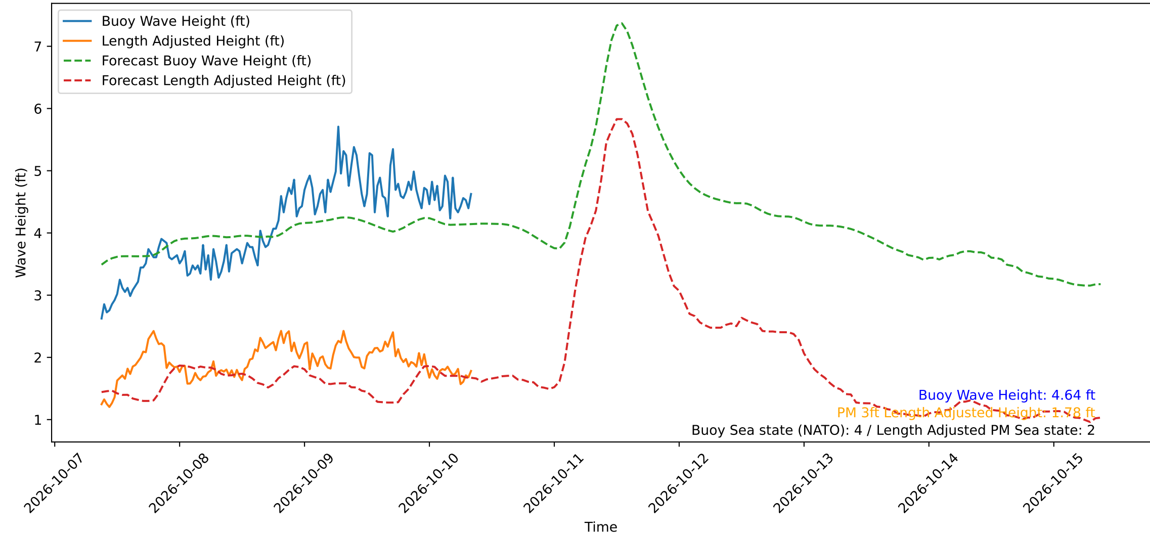
Wave Heights over Time for Red Beach at 2026-10-10 08:50:50
