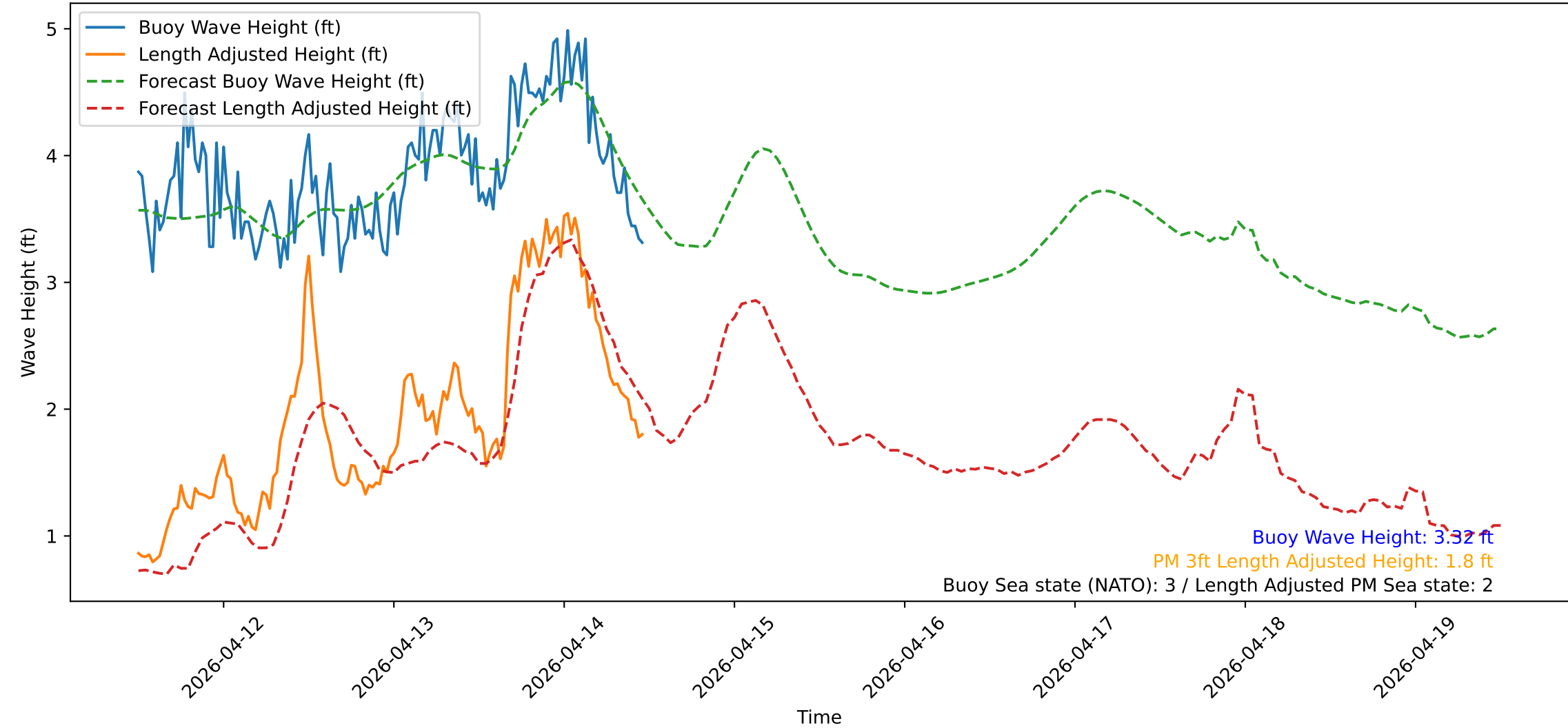
Wave Heights over Time for Green Beach at 2026-04-14 11:51:15
