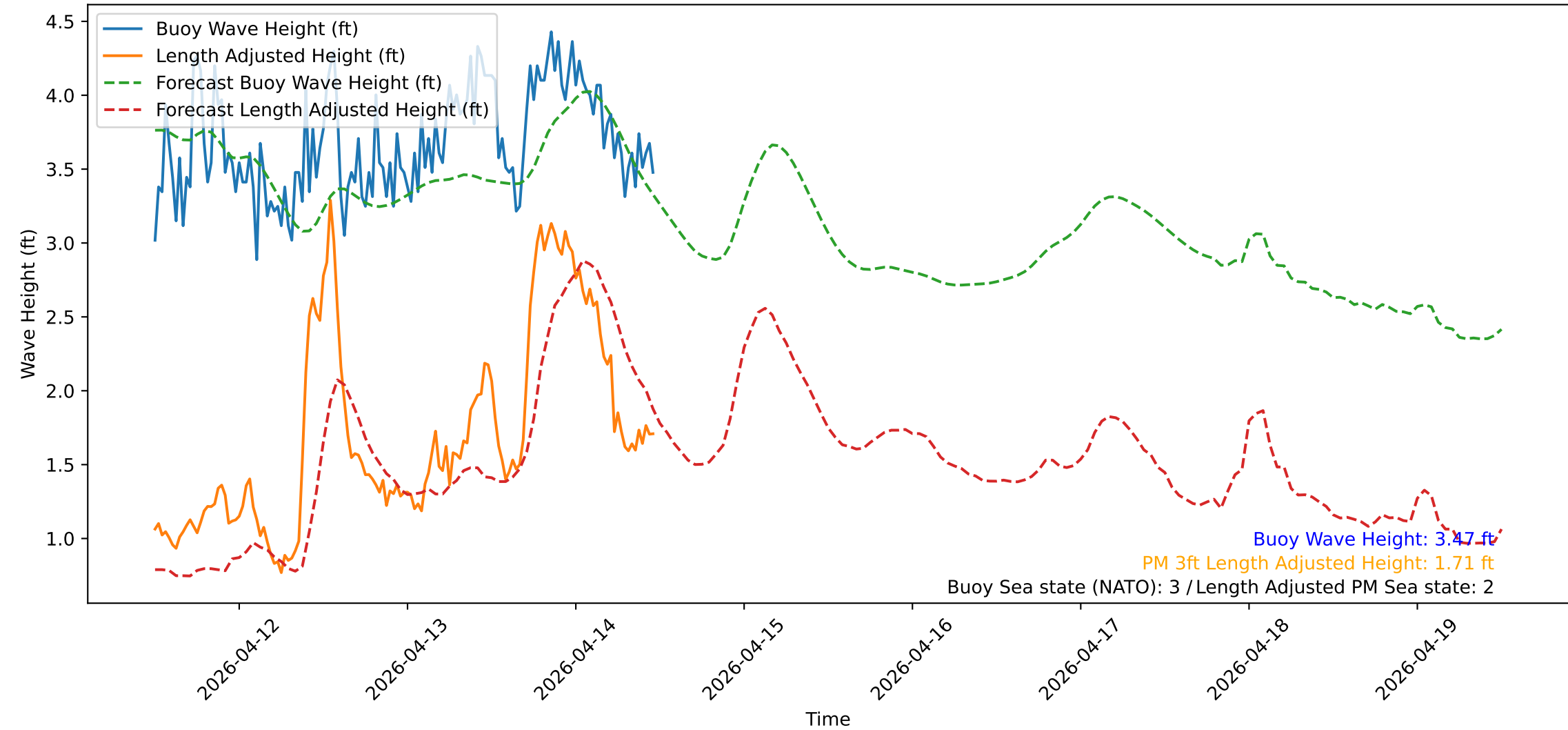
Wave Heights over Time for Red Beach at 2026-04-14 11:50:52
