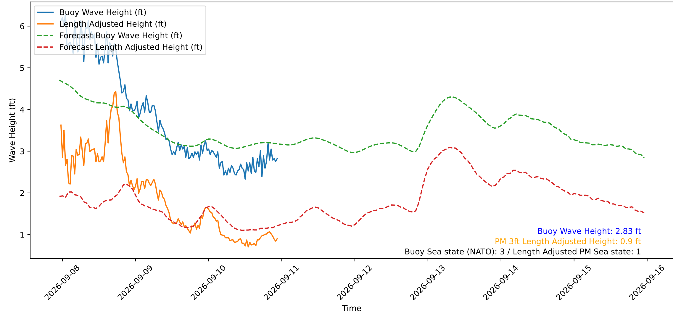
Wave Heights over Time for Red Beach at 2026-09-10 23:10:50
