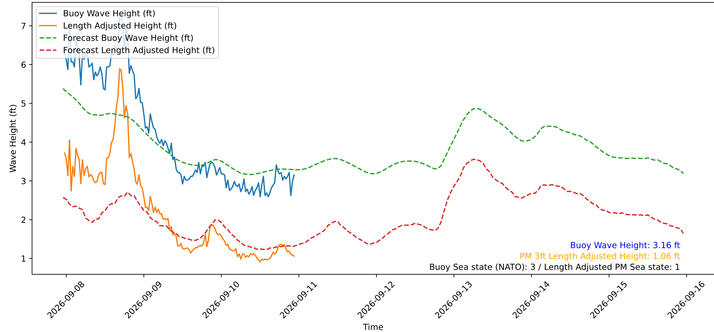
Wave Heights over Time for Green Beach at 2026-09-10 23:11:12
