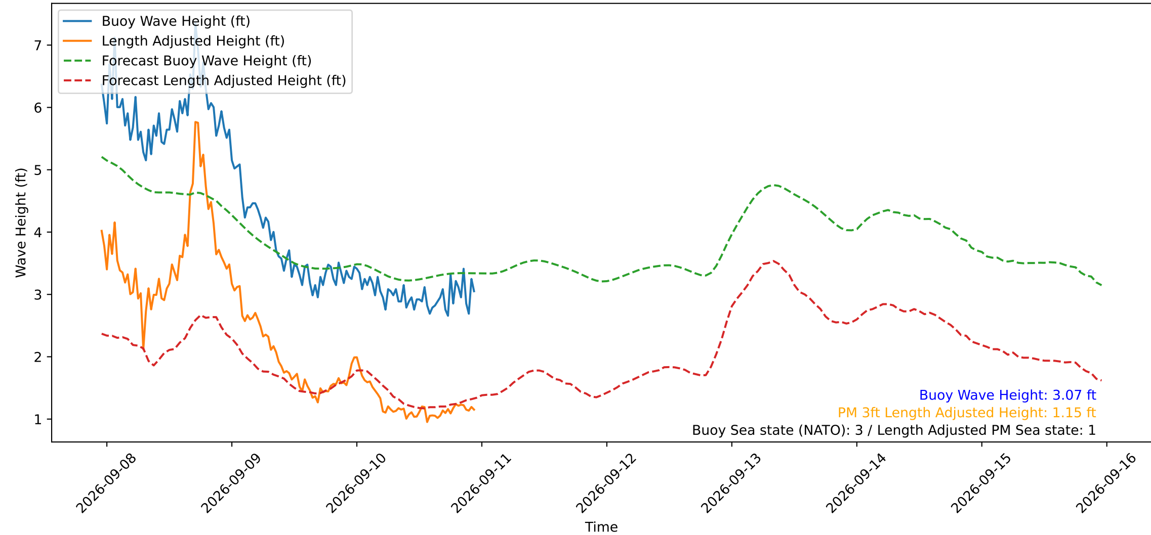
Wave Heights over Time for Oceanside Harbor at 2026-09-10 23:10:30
