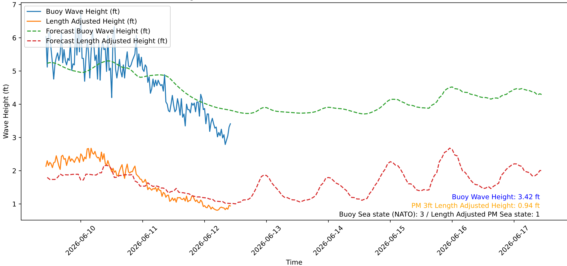
Wave Heights over Time for Oceanside Harbor at 2026-06-12 10:40:27
