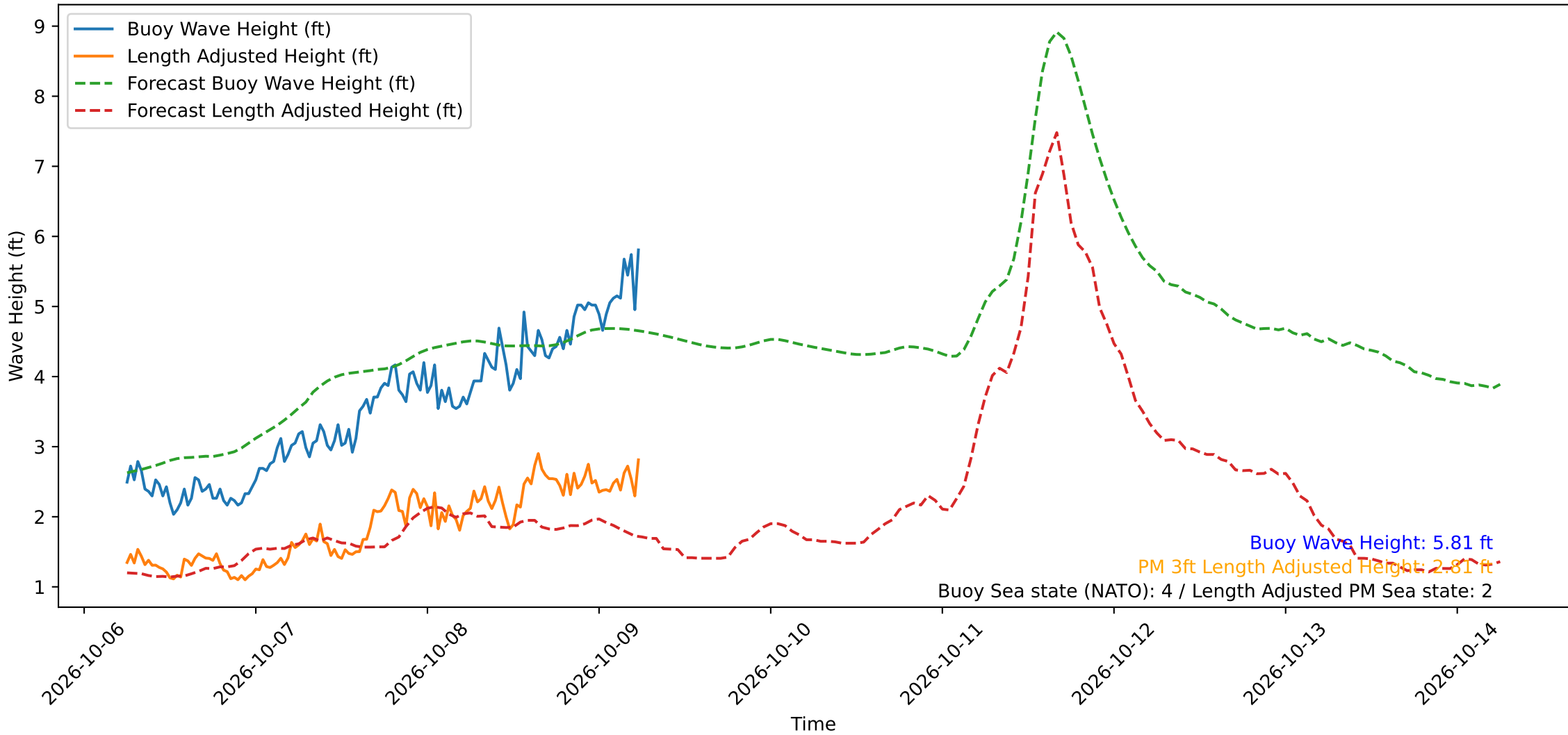
Wave Heights over Time for Oceanside Harbor at 2026-10-09 06:10:29
