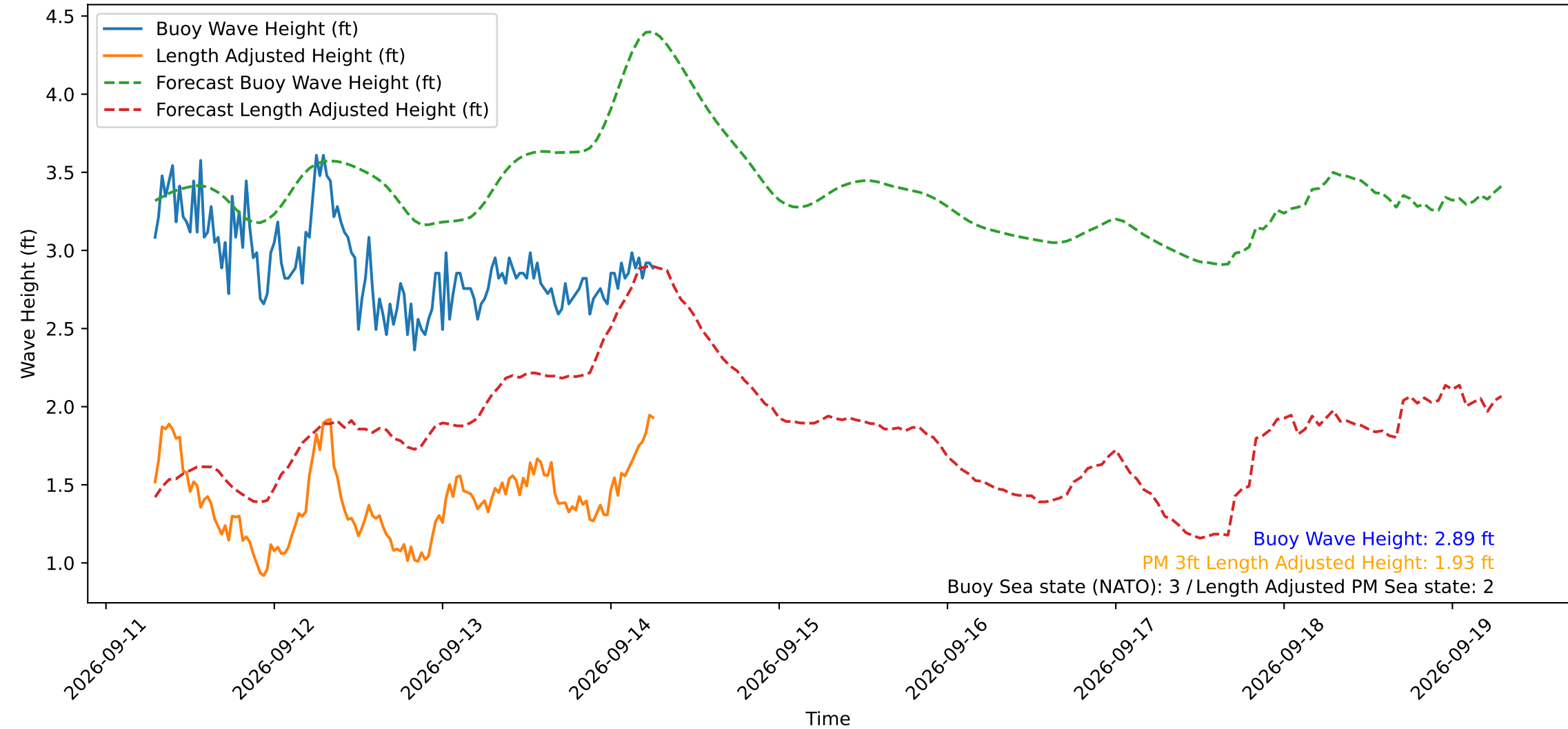
Wave Heights over Time for Green Beach at 2026-09-14 06:51:15
