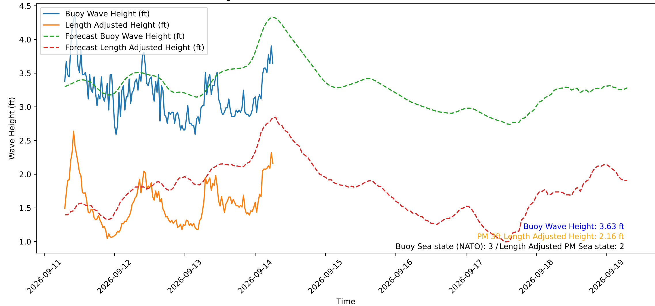
Wave Heights over Time for Oceanside Harbor at 2026-09-14 06:50:29
