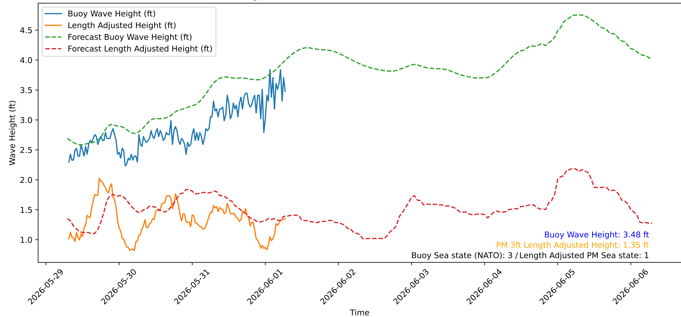
Wave Heights over Time for Red Beach at 2026-06-01 07:10:46
