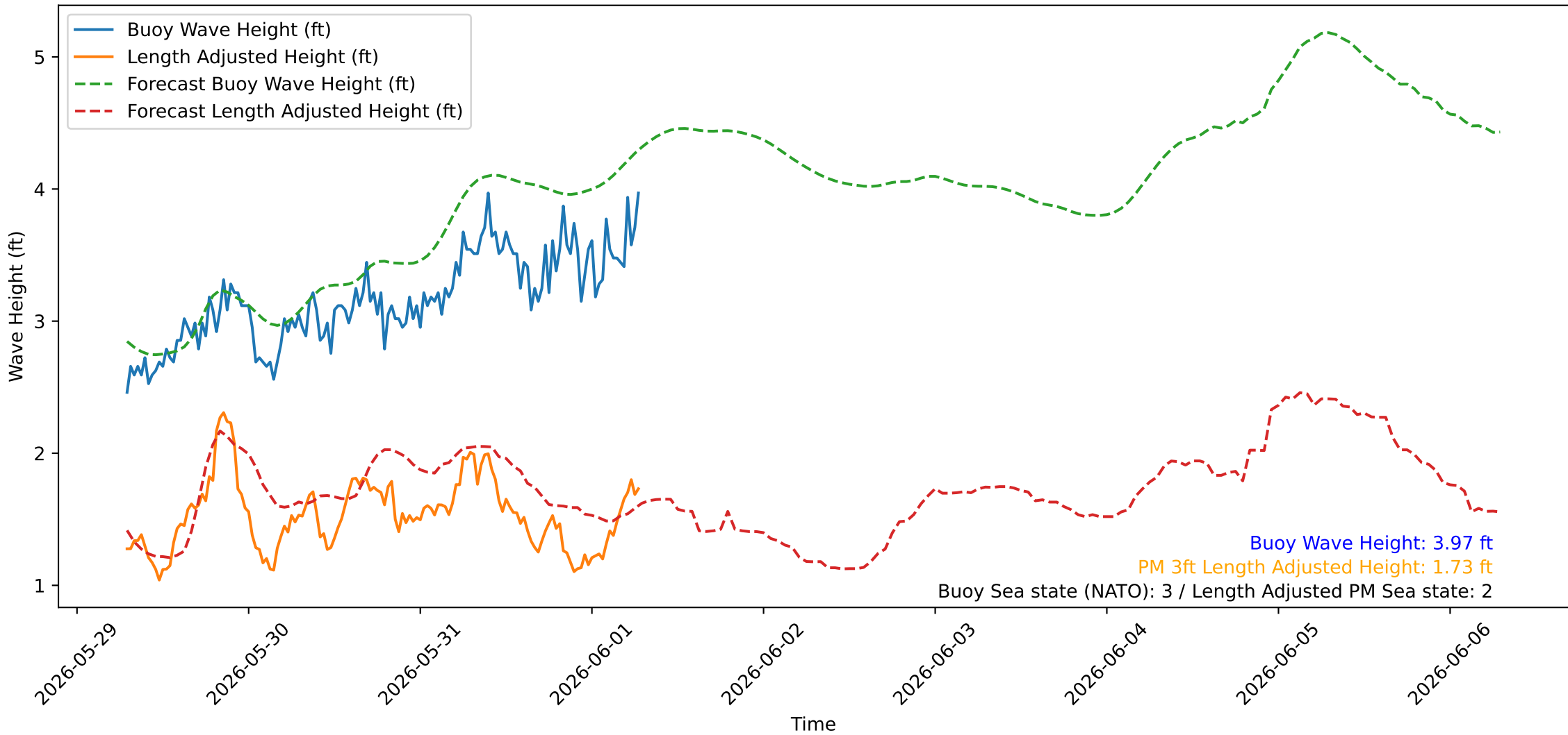
Wave Heights over Time for Green Beach at 2026-06-01 07:11:08
