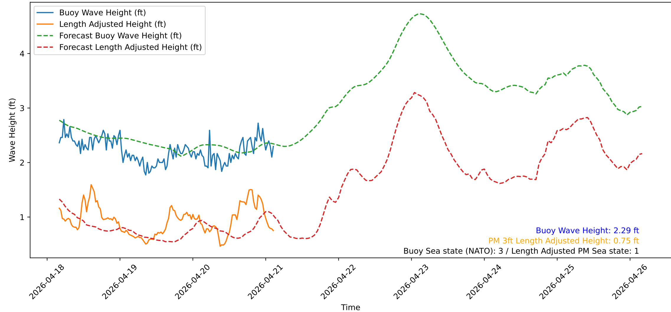
Wave Heights over Time for Red Beach at 2026-04-21 03:40:51
