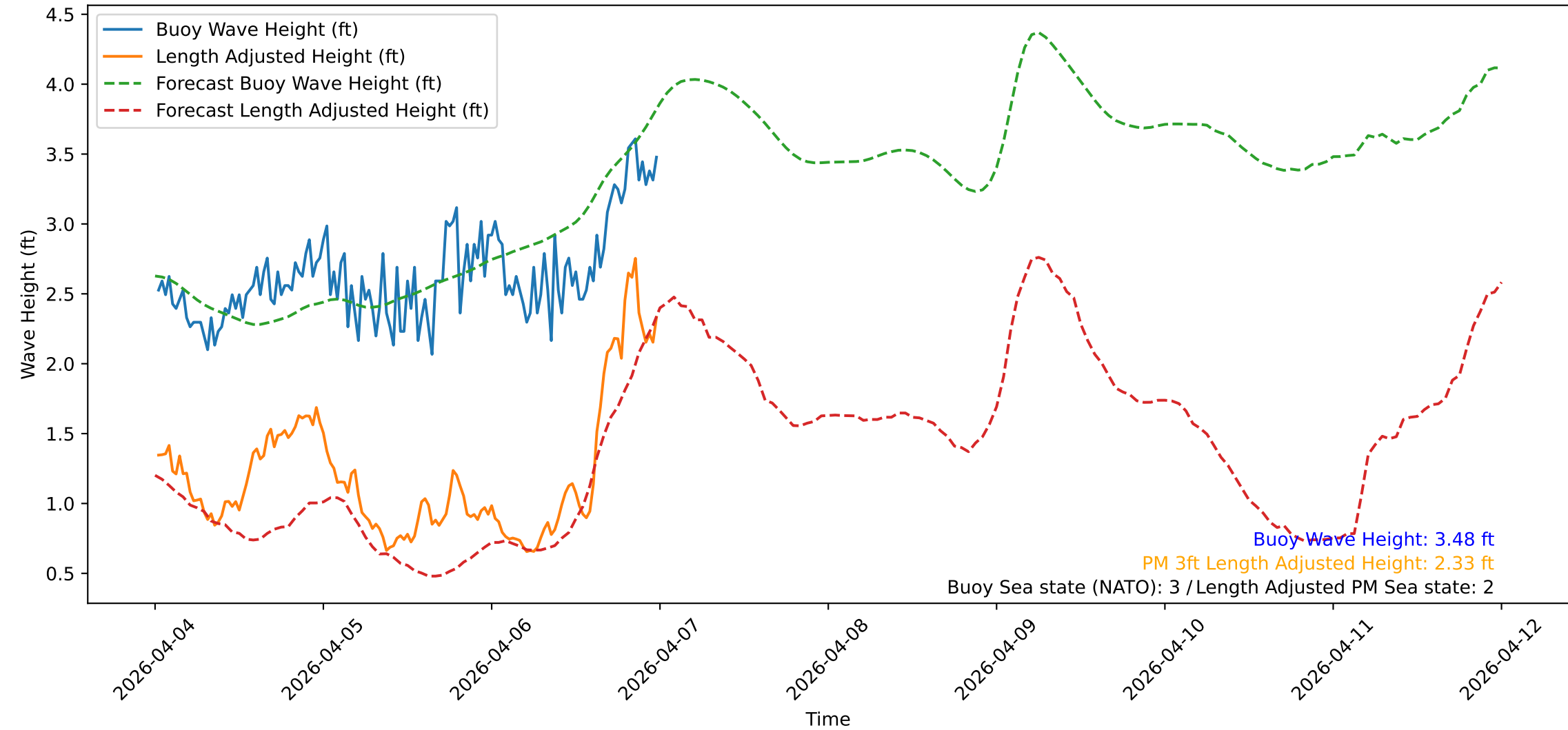
Wave Heights over Time for Oceanside Harbor at 2026-04-07 00:20:31
