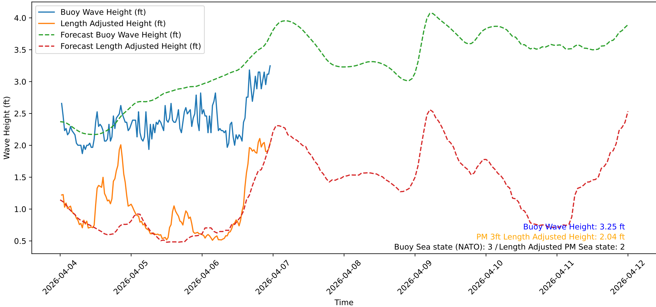
Wave Heights over Time for Red Beach at 2026-04-07 00:20:47
