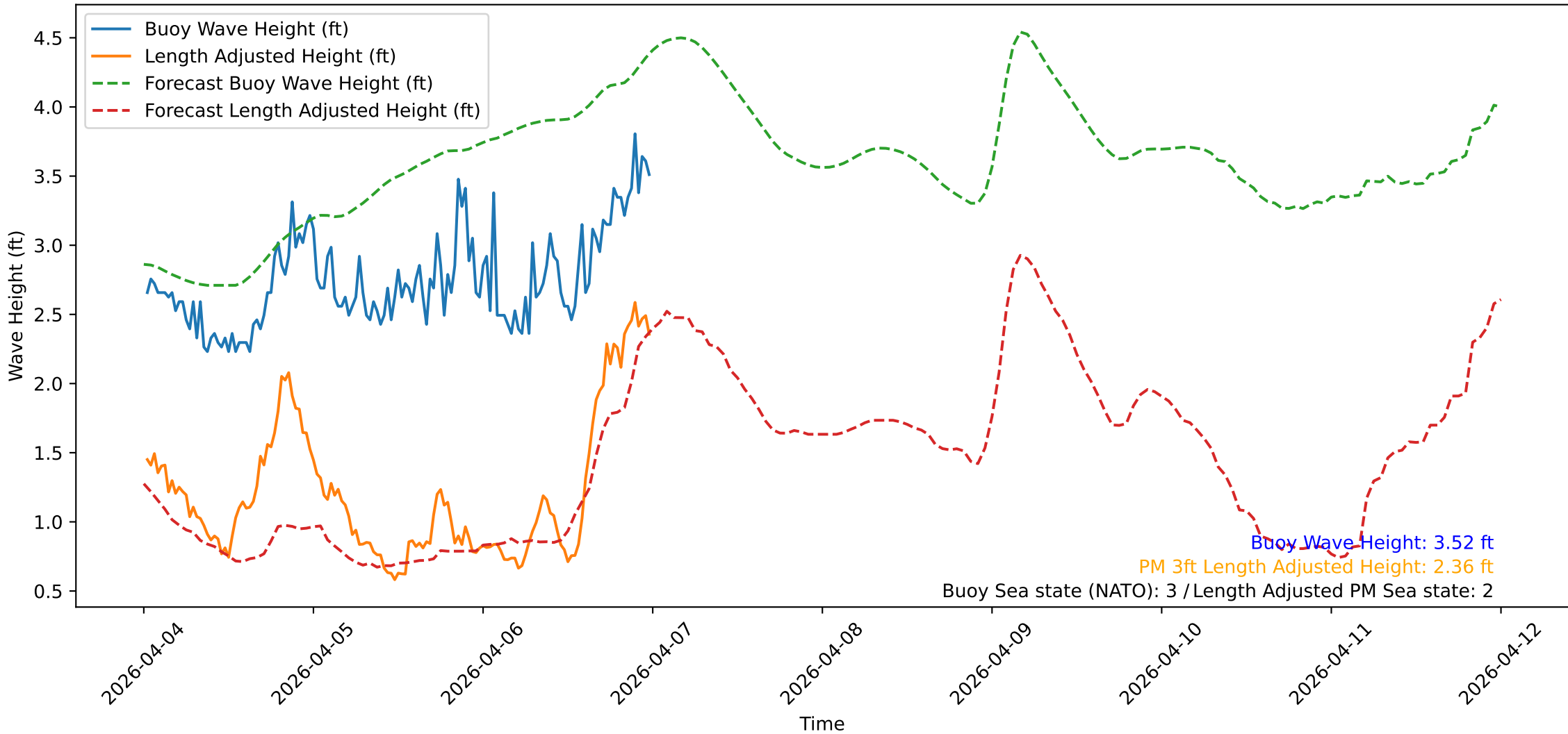
Wave Heights over Time for Green Beach at 2026-04-07 00:21:09
