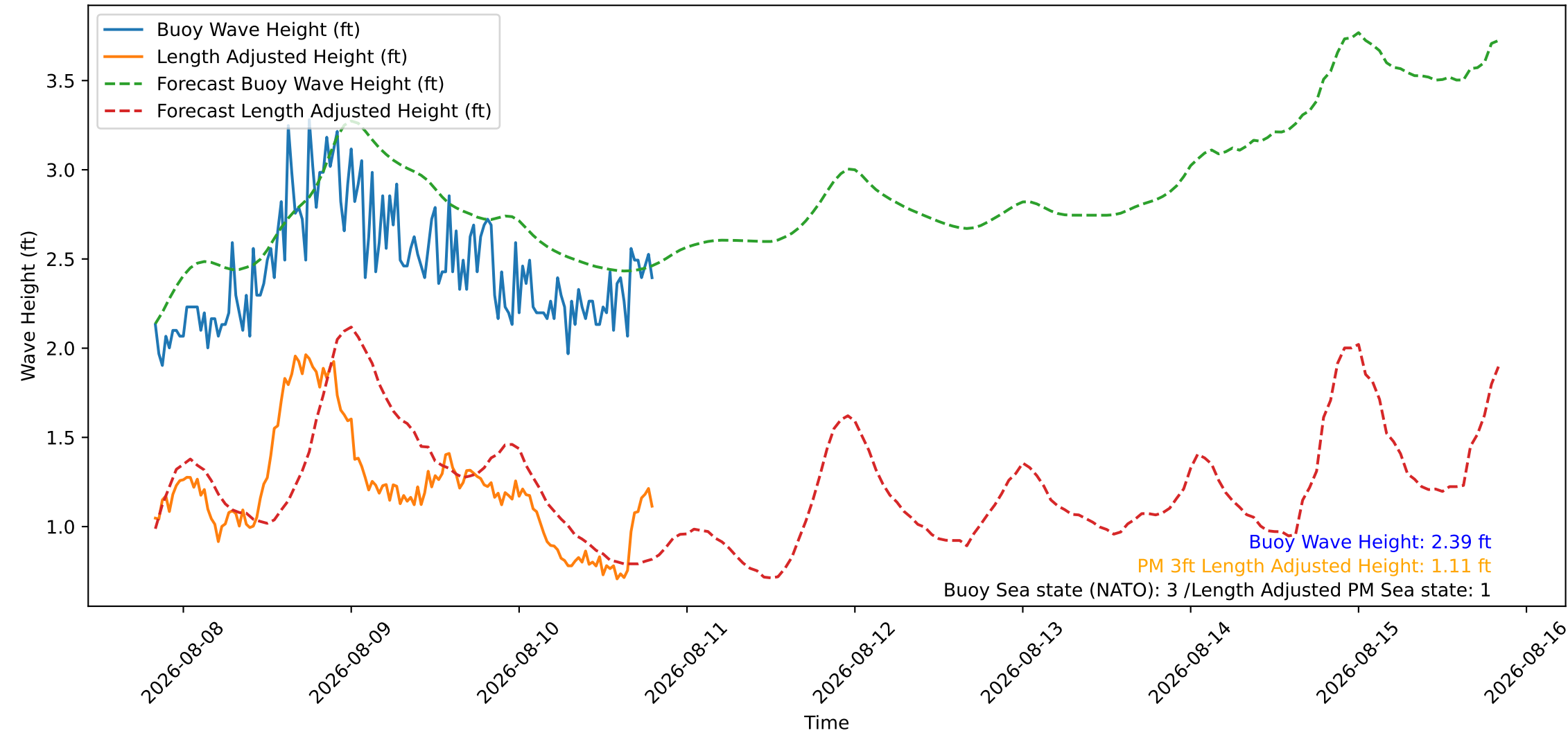
Wave Heights over Time for Oceanside Harbor at 2026-08-10 19:50:26
