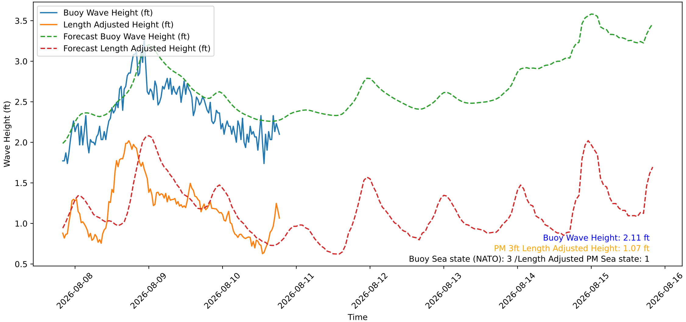
Wave Heights over Time for Red Beach at 2026-08-10 19:50:47
