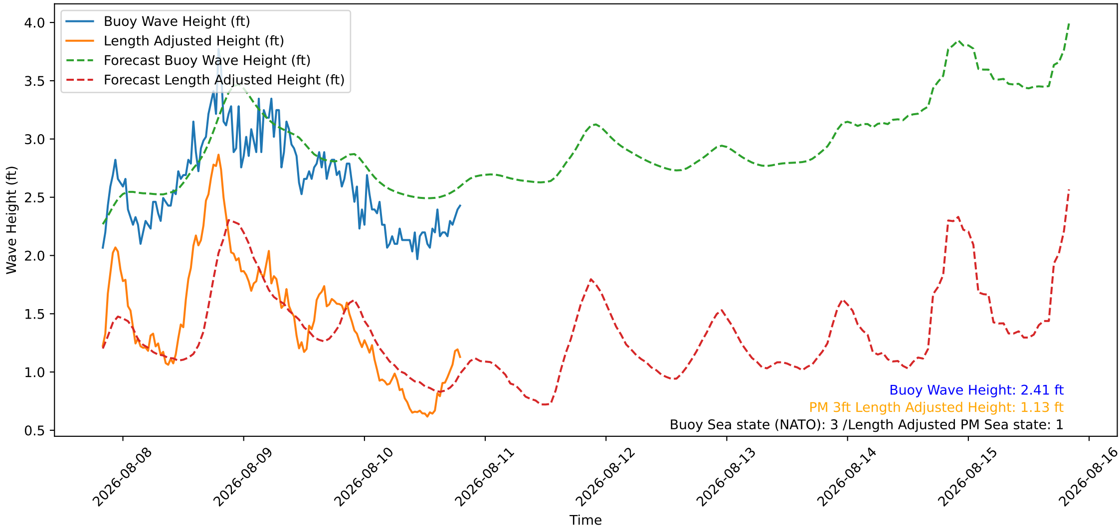
Wave Heights over Time for Green Beach at 2026-08-10 19:51:09
