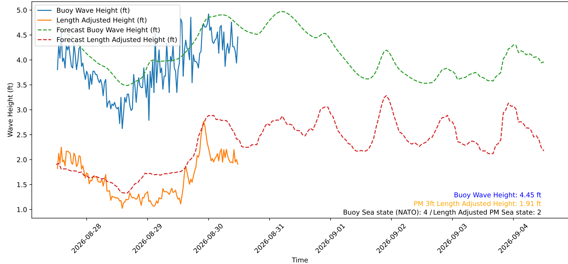
Wave Heights over Time for Green Beach at 2026-08-30 12:11:11
