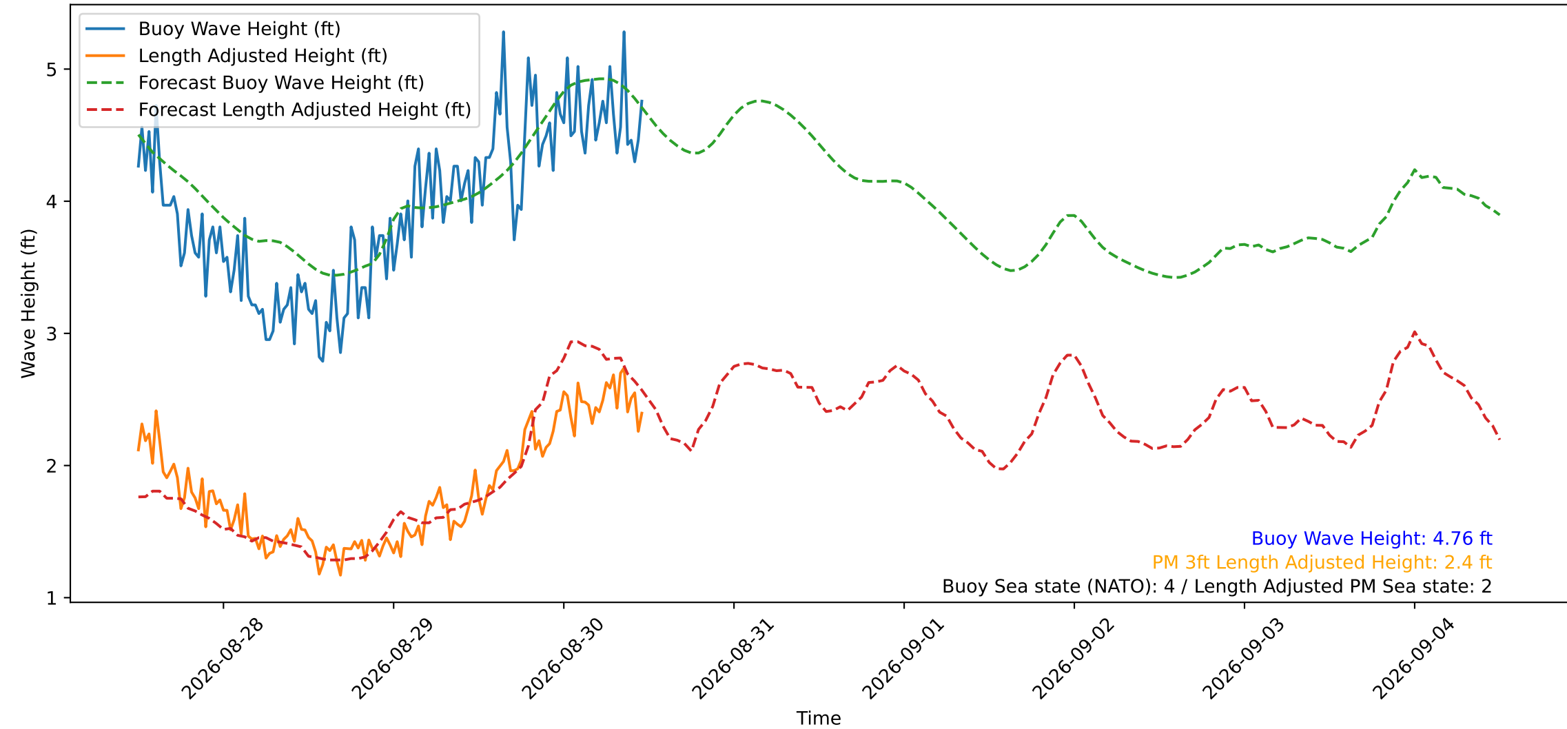
Wave Heights over Time for Oceanside Harbor at 2026-08-30 12:10:29
