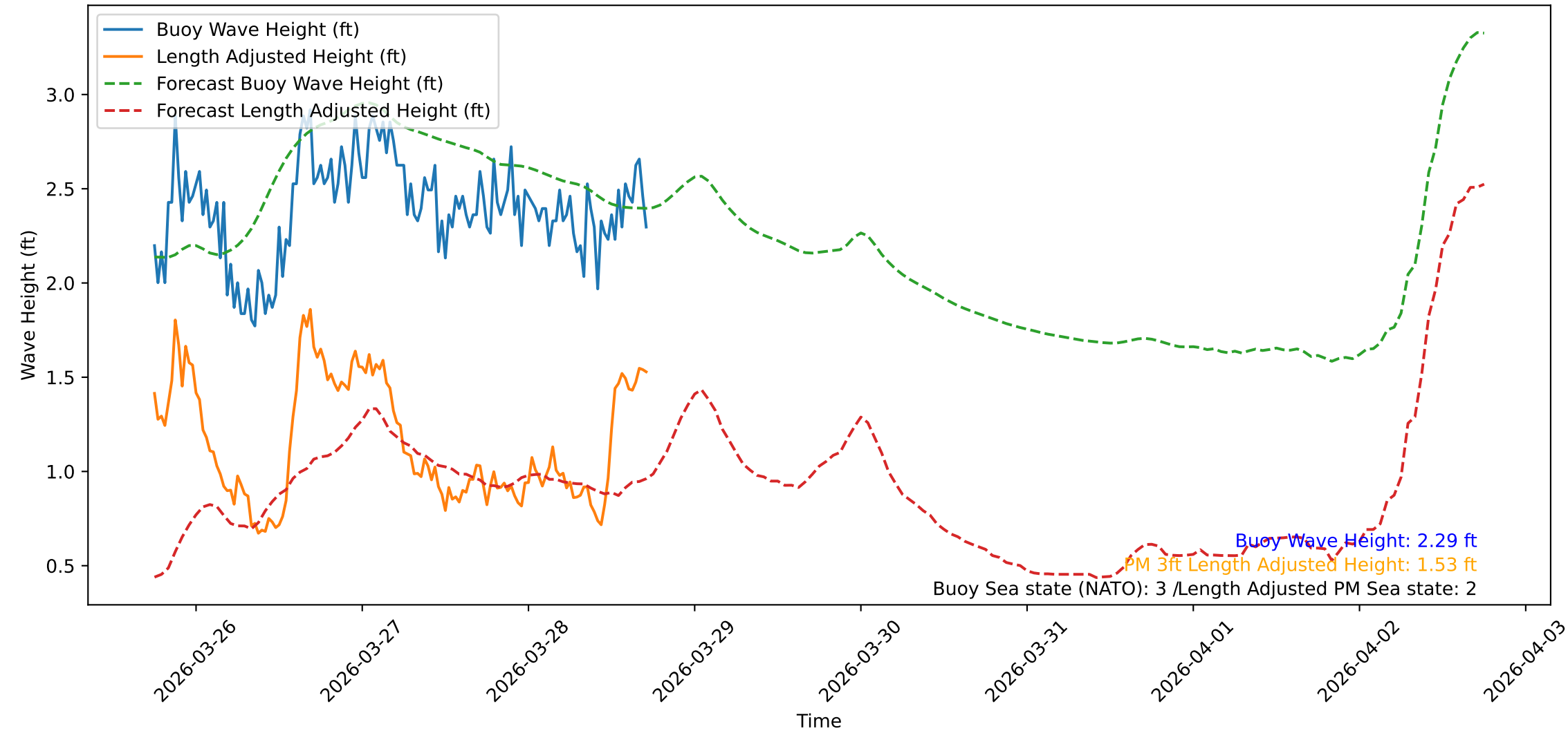
Wave Heights over Time for Oceanside Harbor at 2026-03-28 17:50:32
