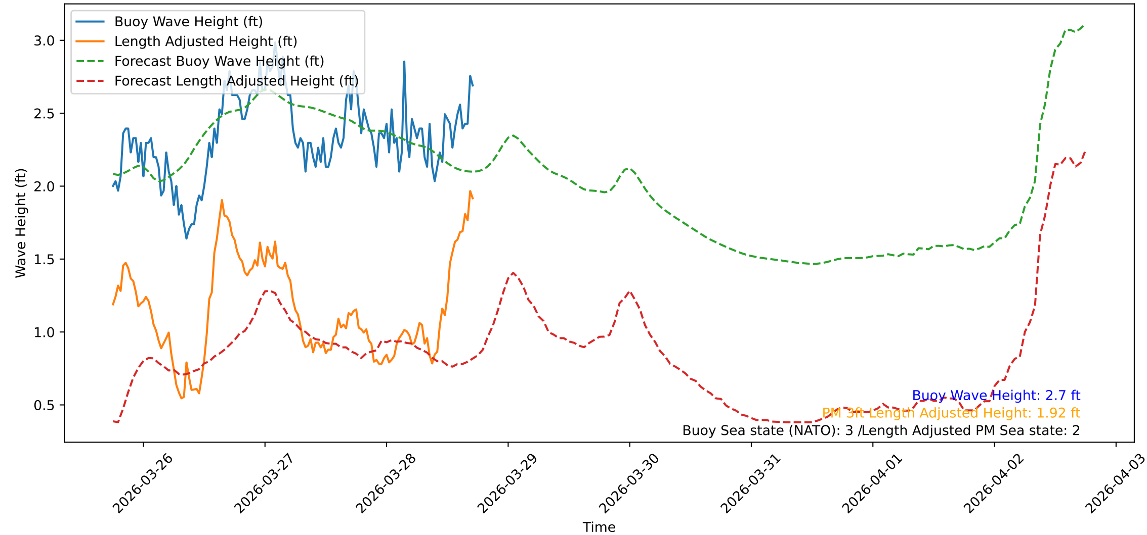
Wave Heights over Time for Red Beach at 2026-03-28 17:50:48
