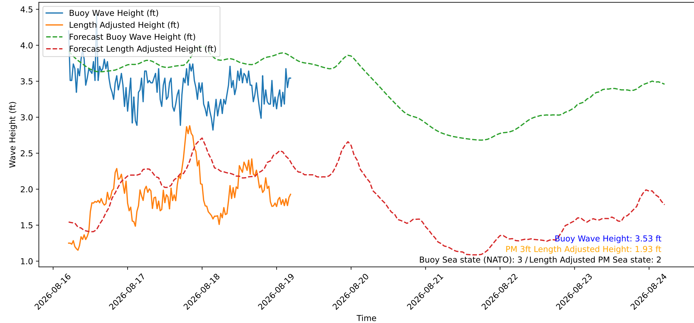
Wave Heights over Time for Oceanside Harbor at 2026-08-19 05:00:26
