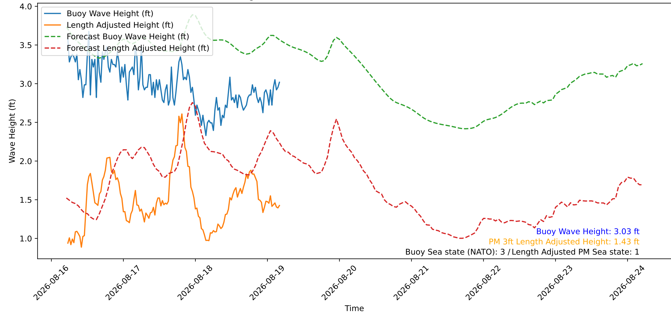
Wave Heights over Time for Red Beach at 2026-08-19 05:00:46
