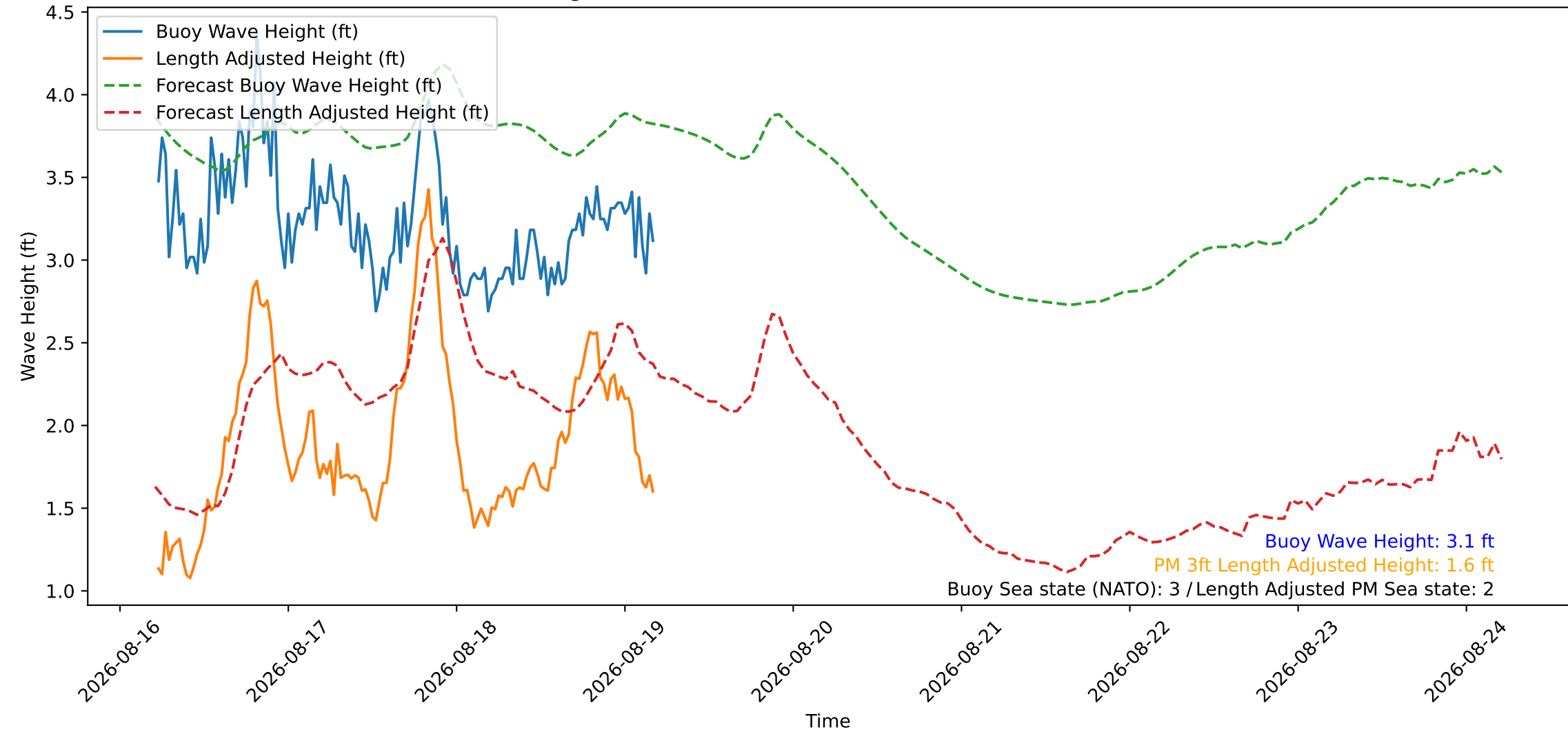
Wave Heights over Time for Green Beach at 2026-08-19 05:01:08
