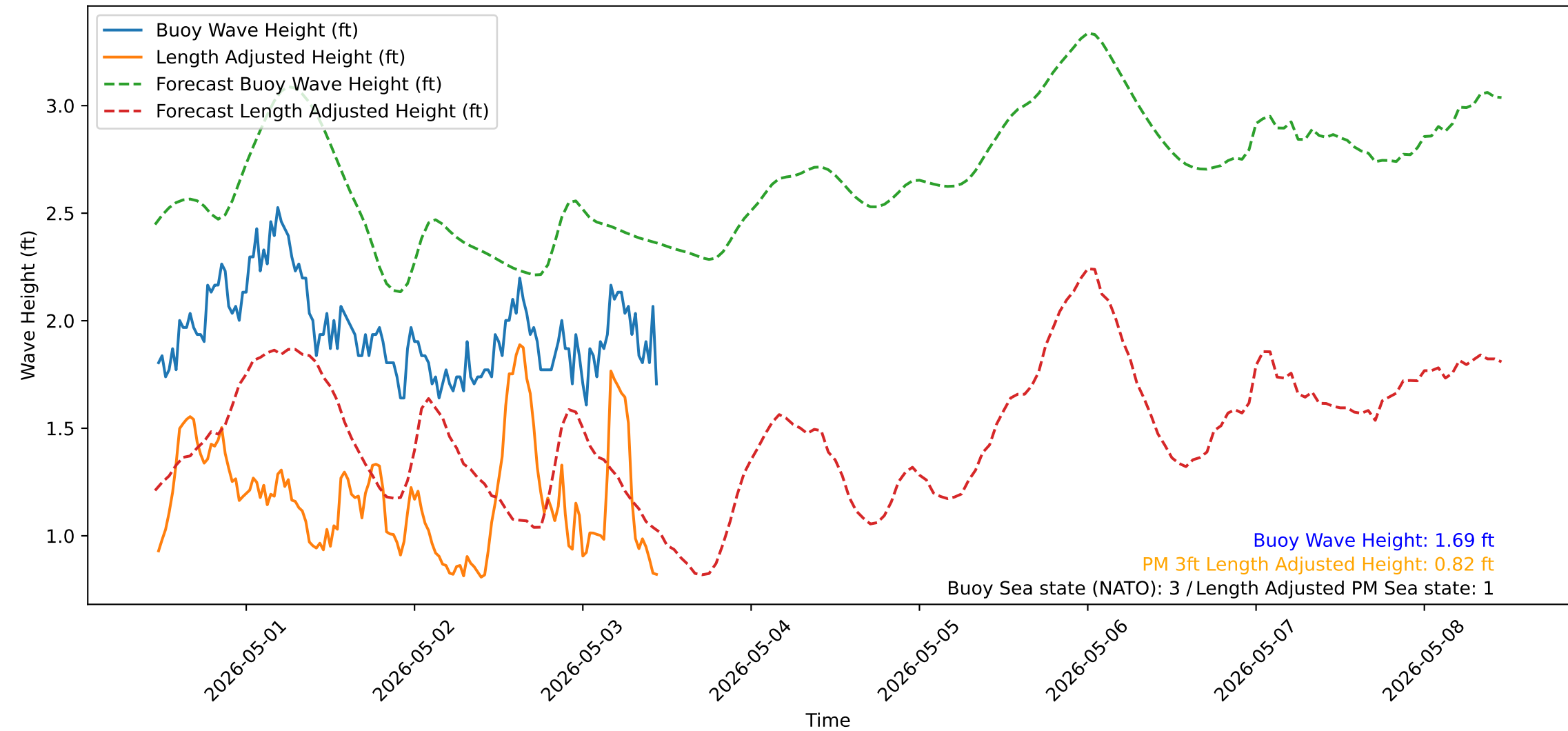
Wave Heights over Time for Red Beach at 2026-05-03 11:20:51
