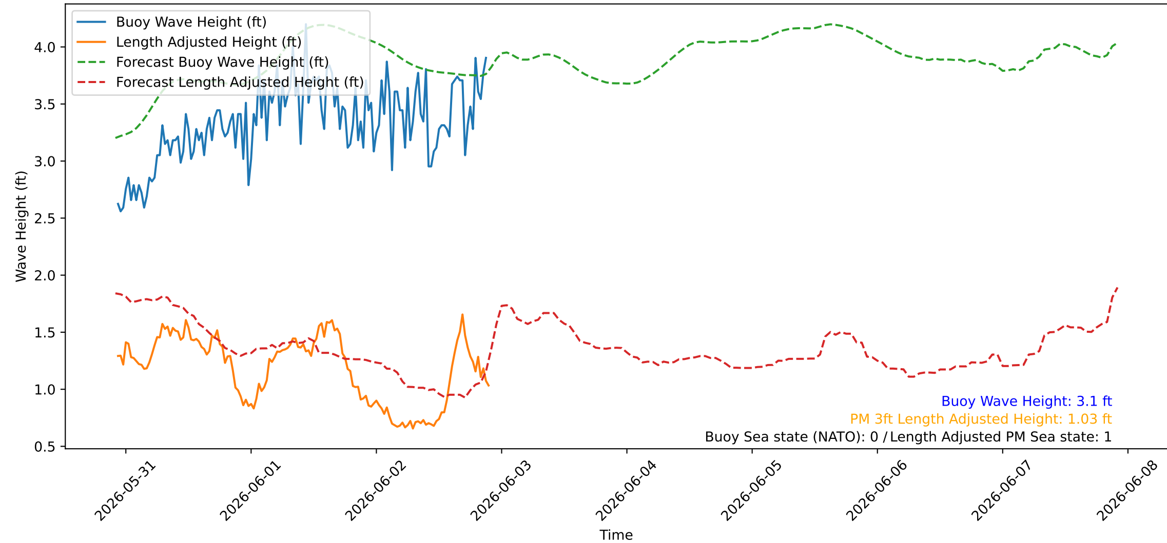
Wave Heights over Time for Red Beach at 2026-06-02 22:10:47
