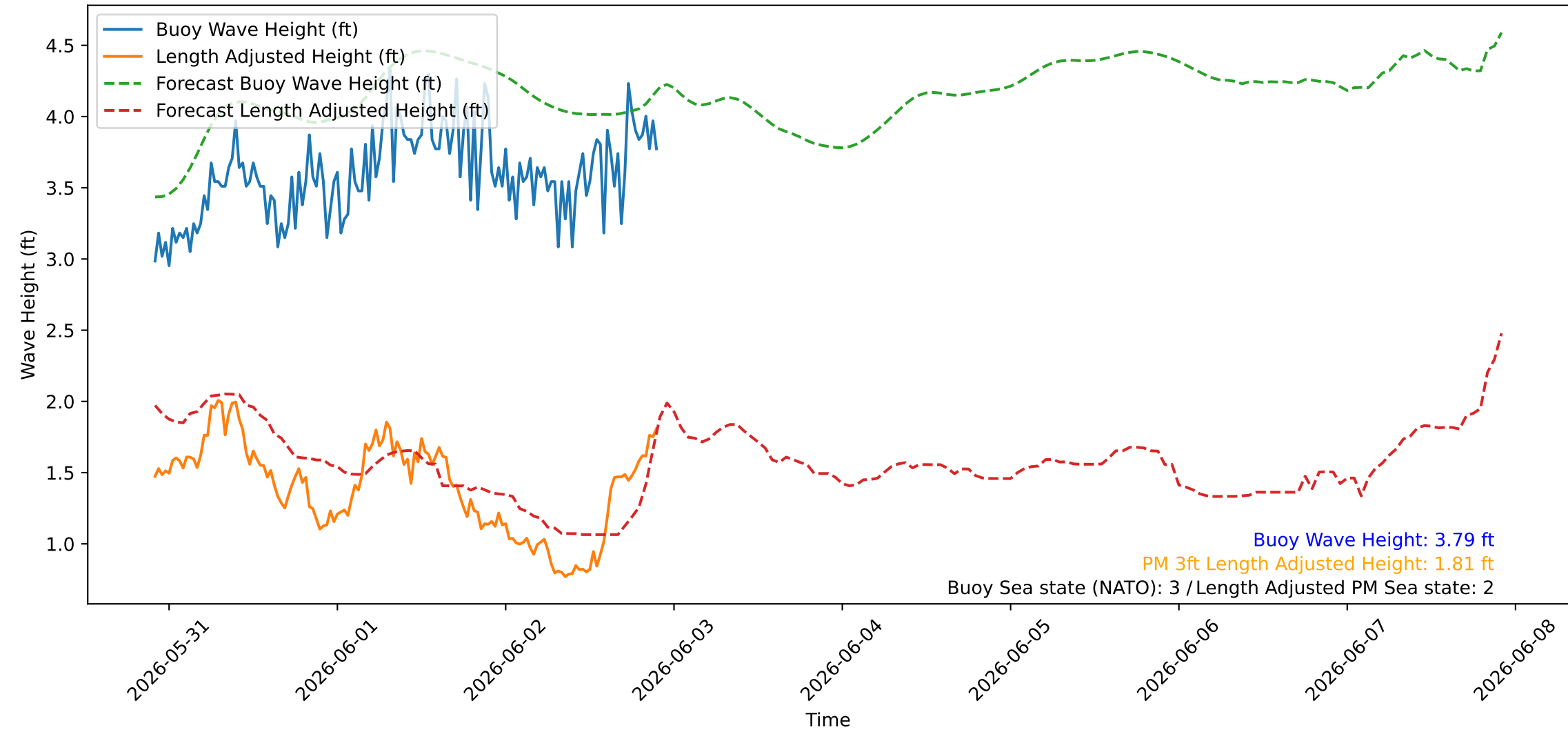
Wave Heights over Time for Green Beach at 2026-06-02 22:11:09
