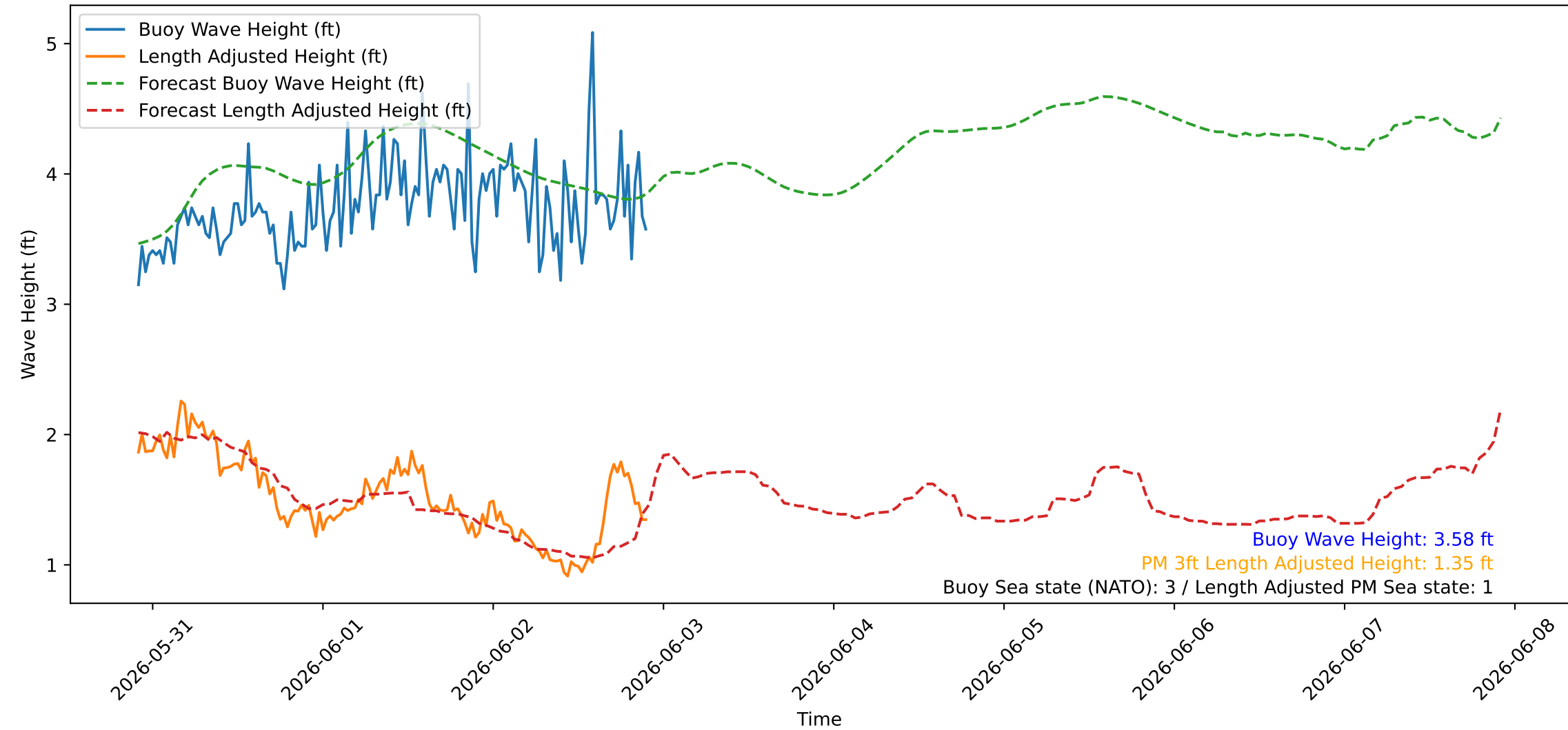
Wave Heights over Time for Oceanside Harbor at 2026-06-02 22:10:25
