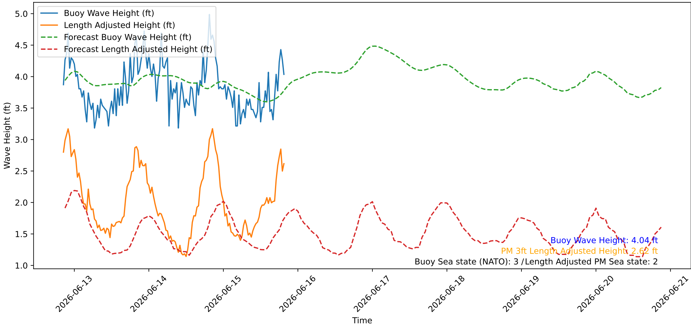
Wave Heights over Time for Oceanside Harbor at 2026-06-15 20:30:26
