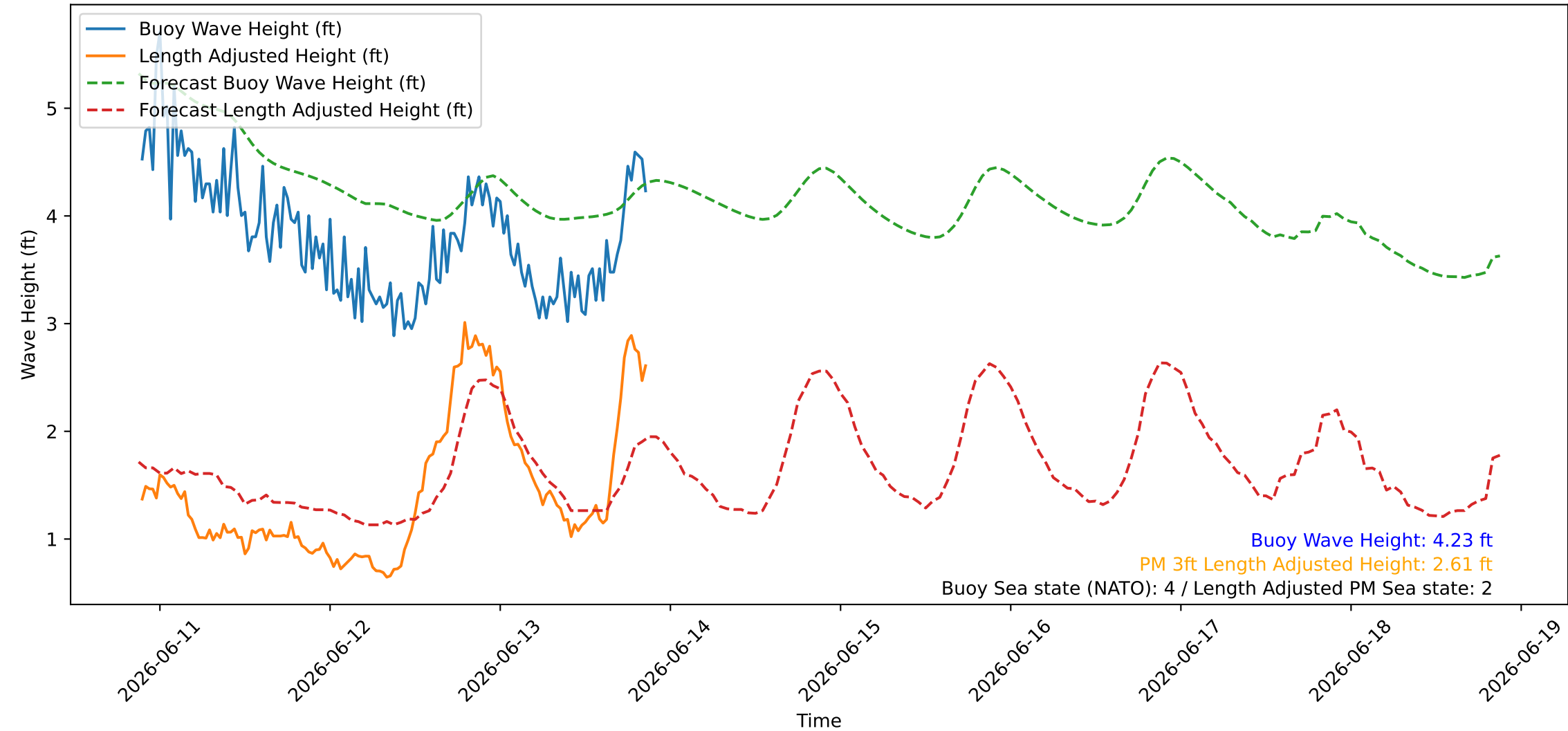
Wave Heights over Time for Green Beach at 2026-06-13 21:21:10
