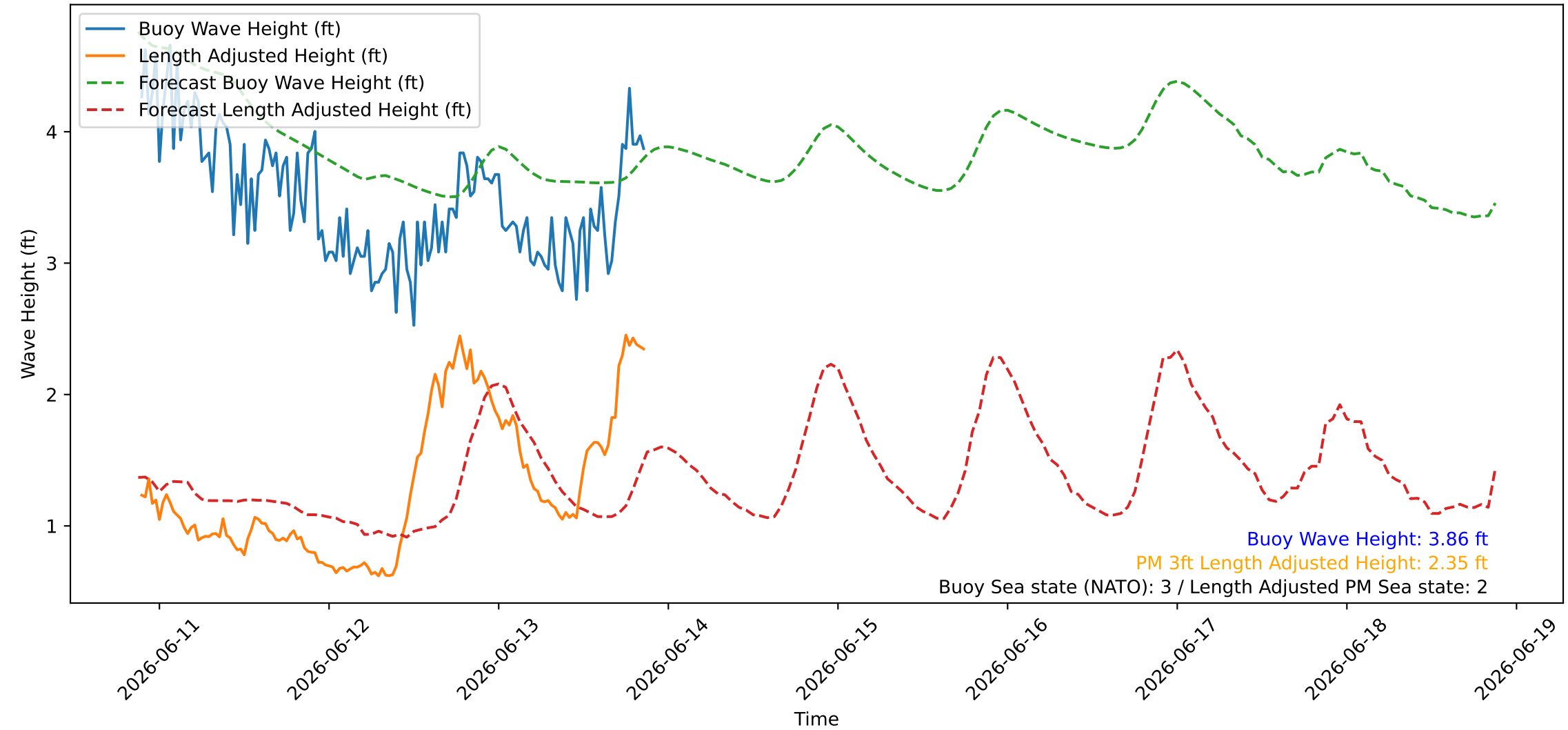
Wave Heights over Time for Red Beach at 2026-06-13 21:20:48
