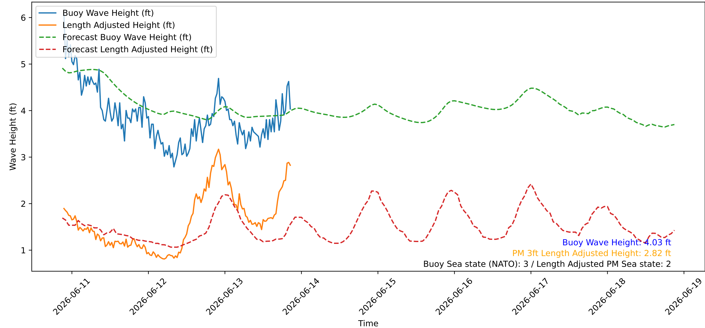
Wave Heights over Time for Oceanside Harbor at 2026-06-13 21:20:27
