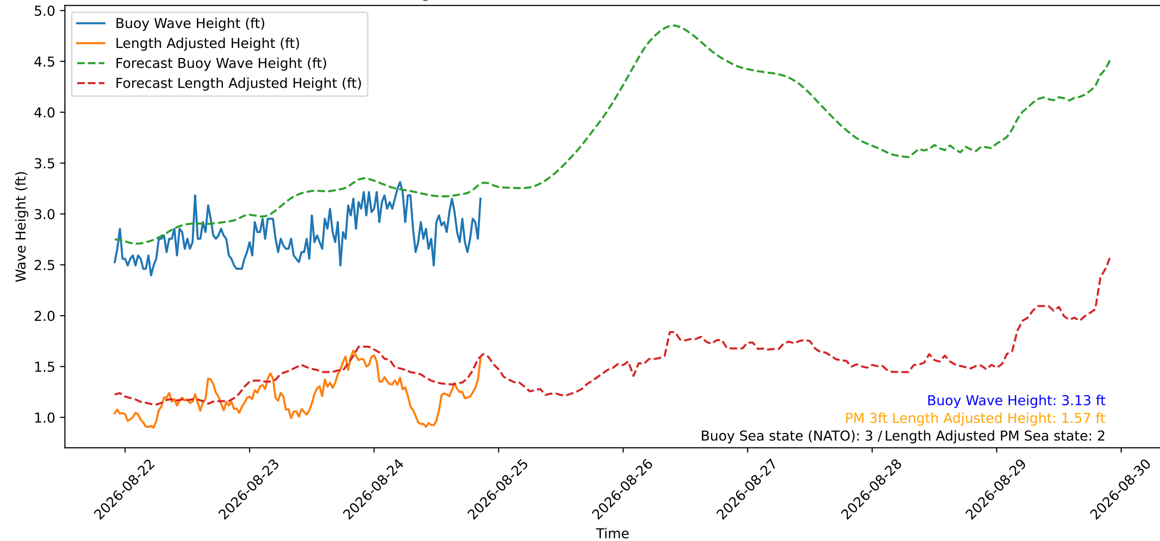
Wave Heights over Time for Green Beach at 2026-08-24 21:31:15
