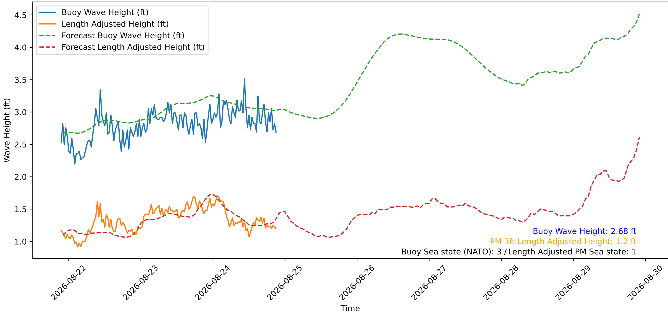
Wave Heights over Time for Oceanside Harbor at 2026-08-24 21:30:32
