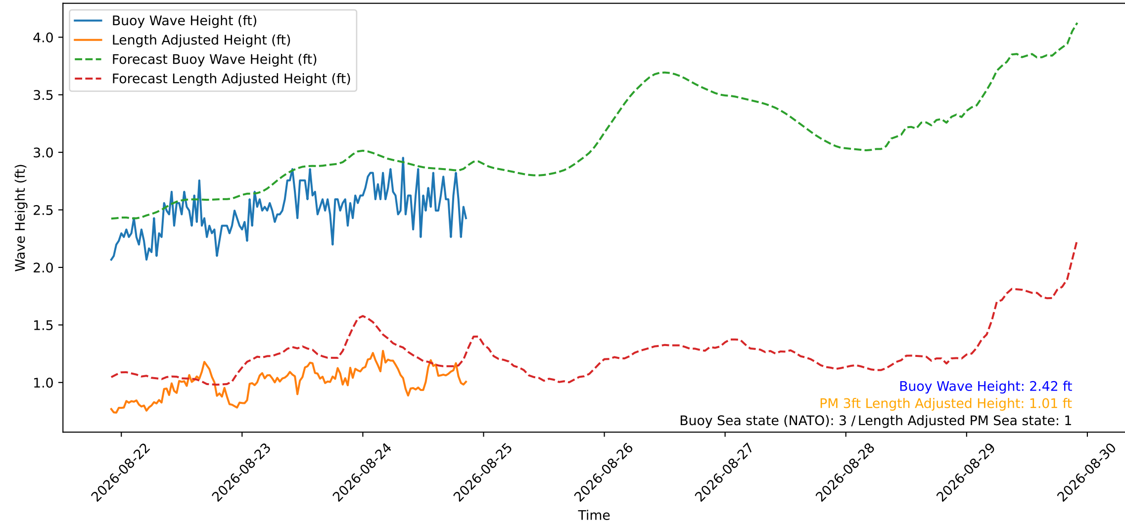
Wave Heights over Time for Red Beach at 2026-08-24 21:30:52
