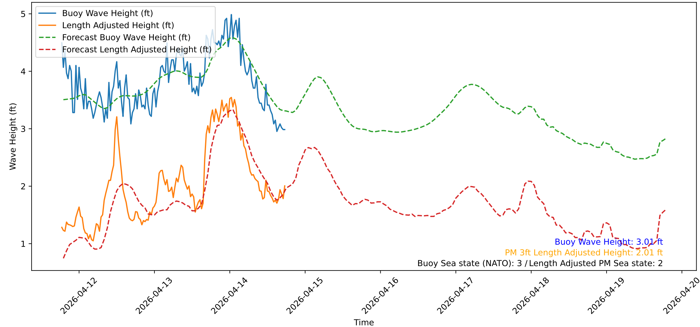
Wave Heights over Time for Green Beach at 2026-04-14 18:31:13
