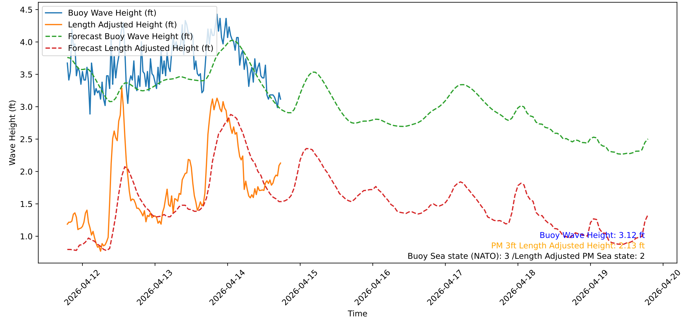
Wave Heights over Time for Red Beach at 2026-04-14 18:30:51
