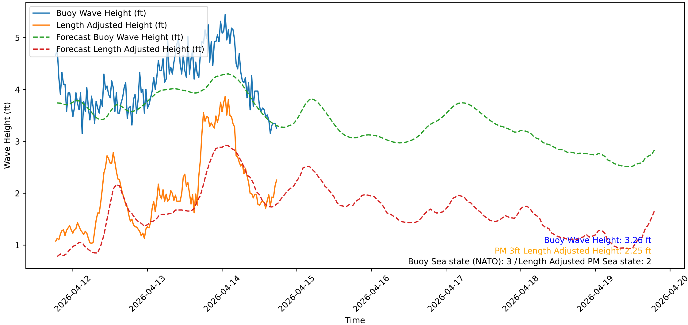
Wave Heights over Time for Oceanside Harbor at 2026-04-14 18:30:31
