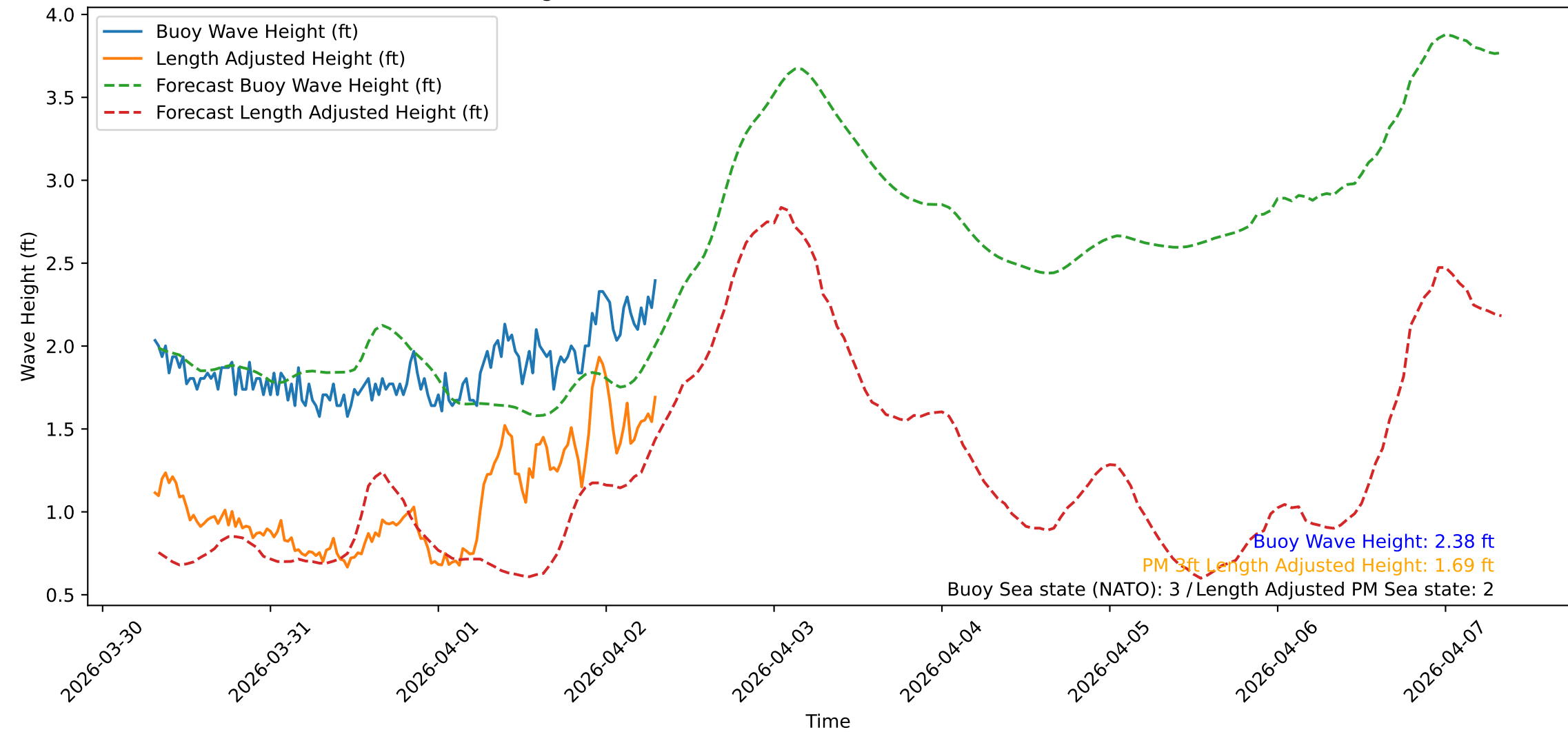
Wave Heights over Time for Oceanside Harbor at 2026-04-02 07:30:32
