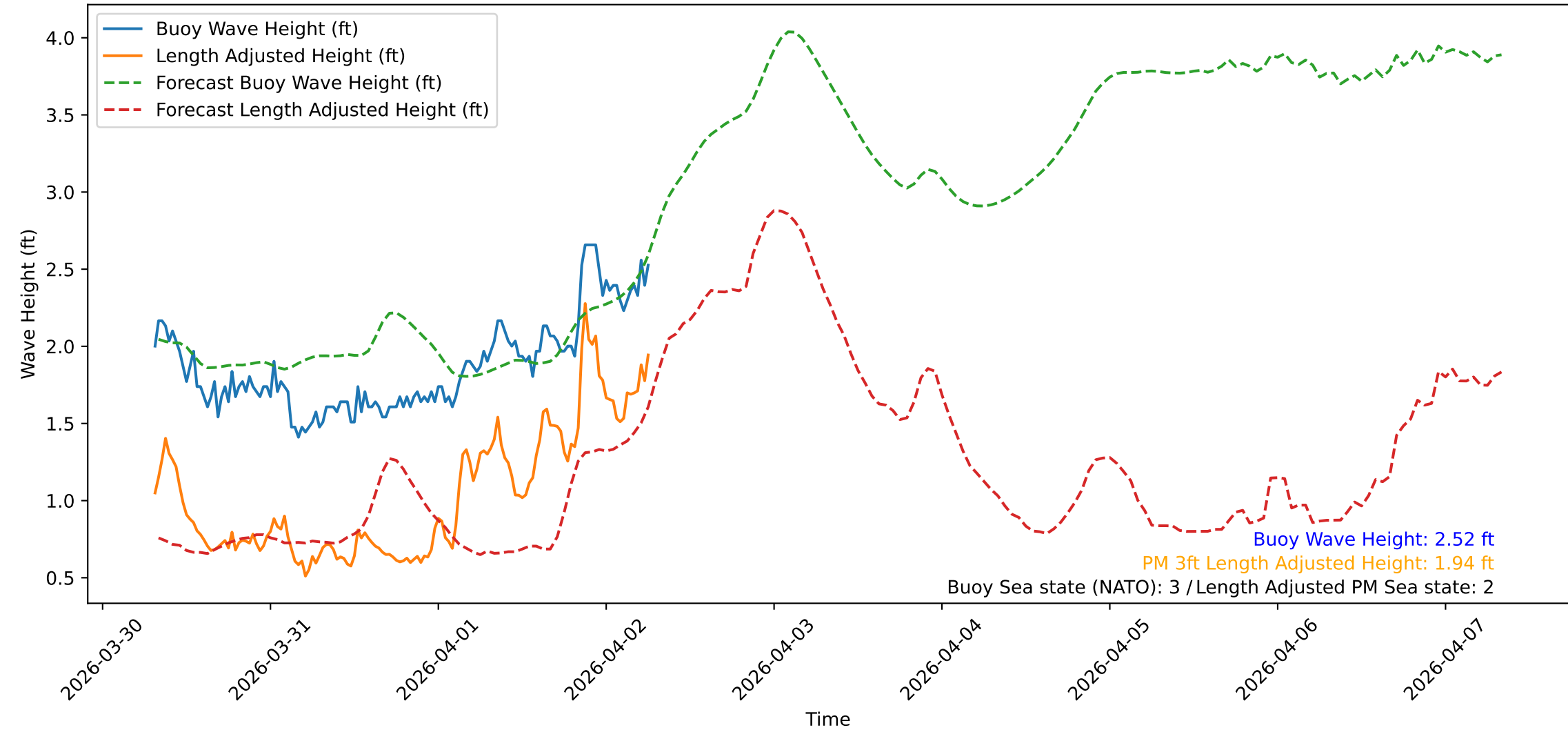
Wave Heights over Time for Green Beach at 2026-04-02 07:31:11
