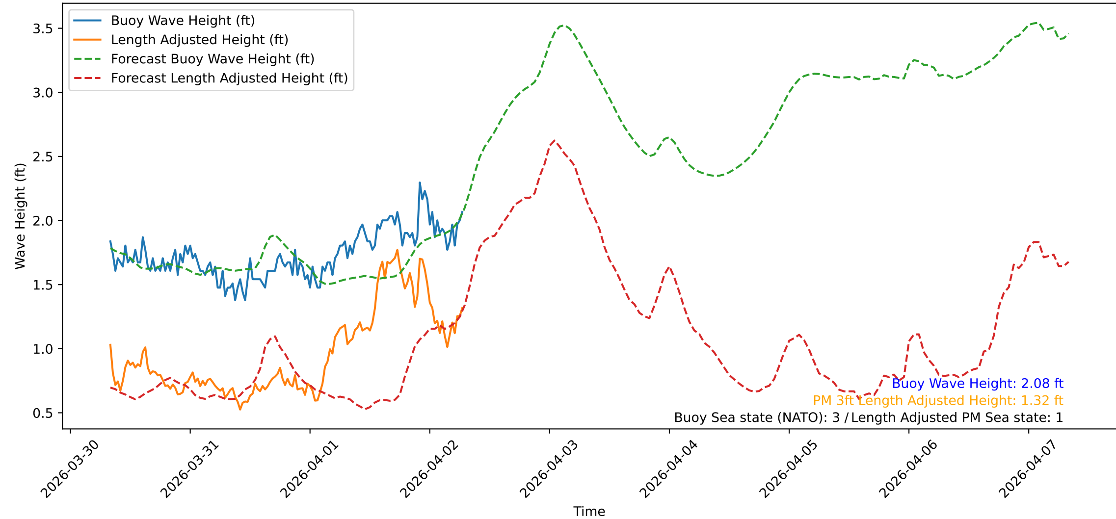
Wave Heights over Time for Red Beach at 2026-04-02 07:30:48
