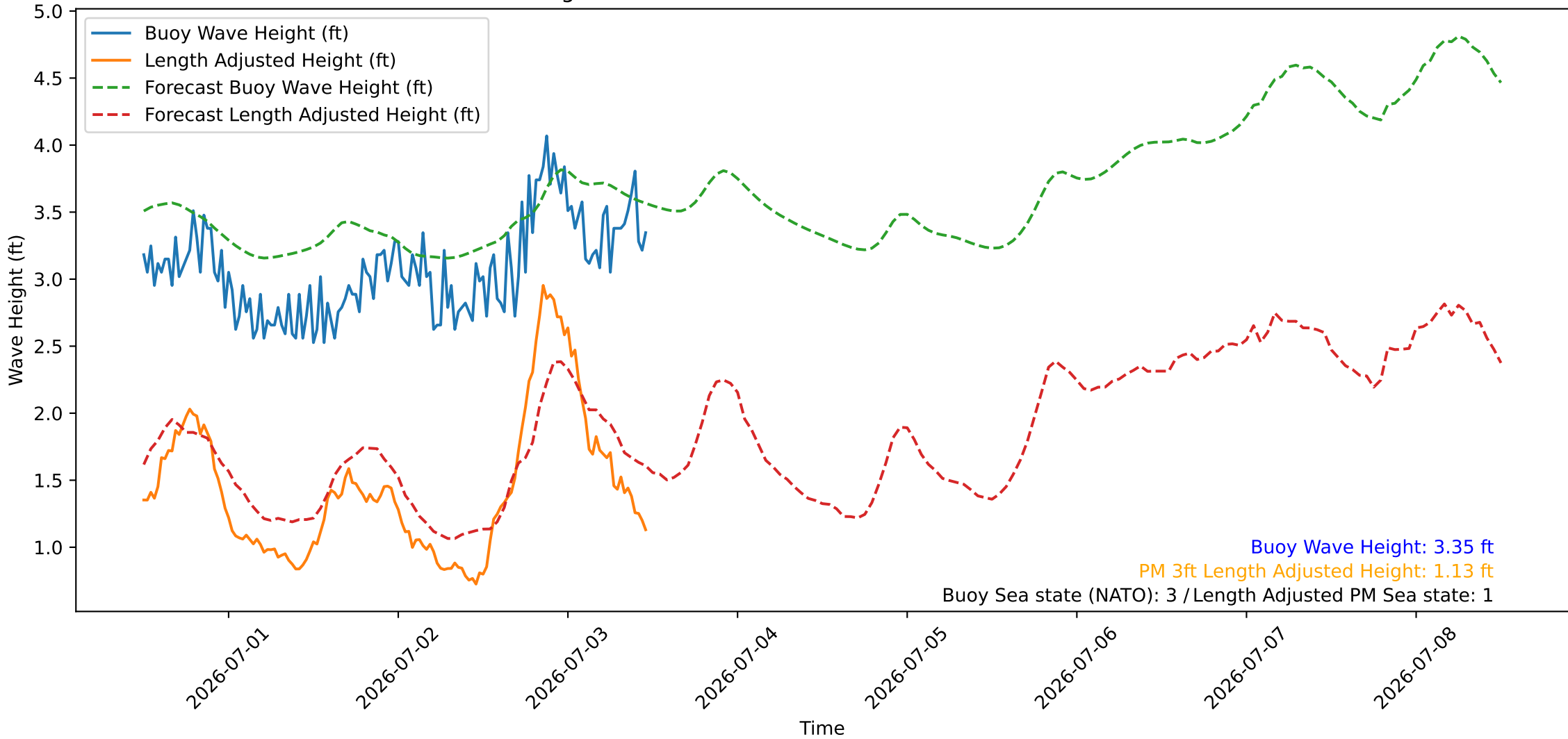
Wave Heights over Time for Green Beach at 2026-07-03 11:51:09
