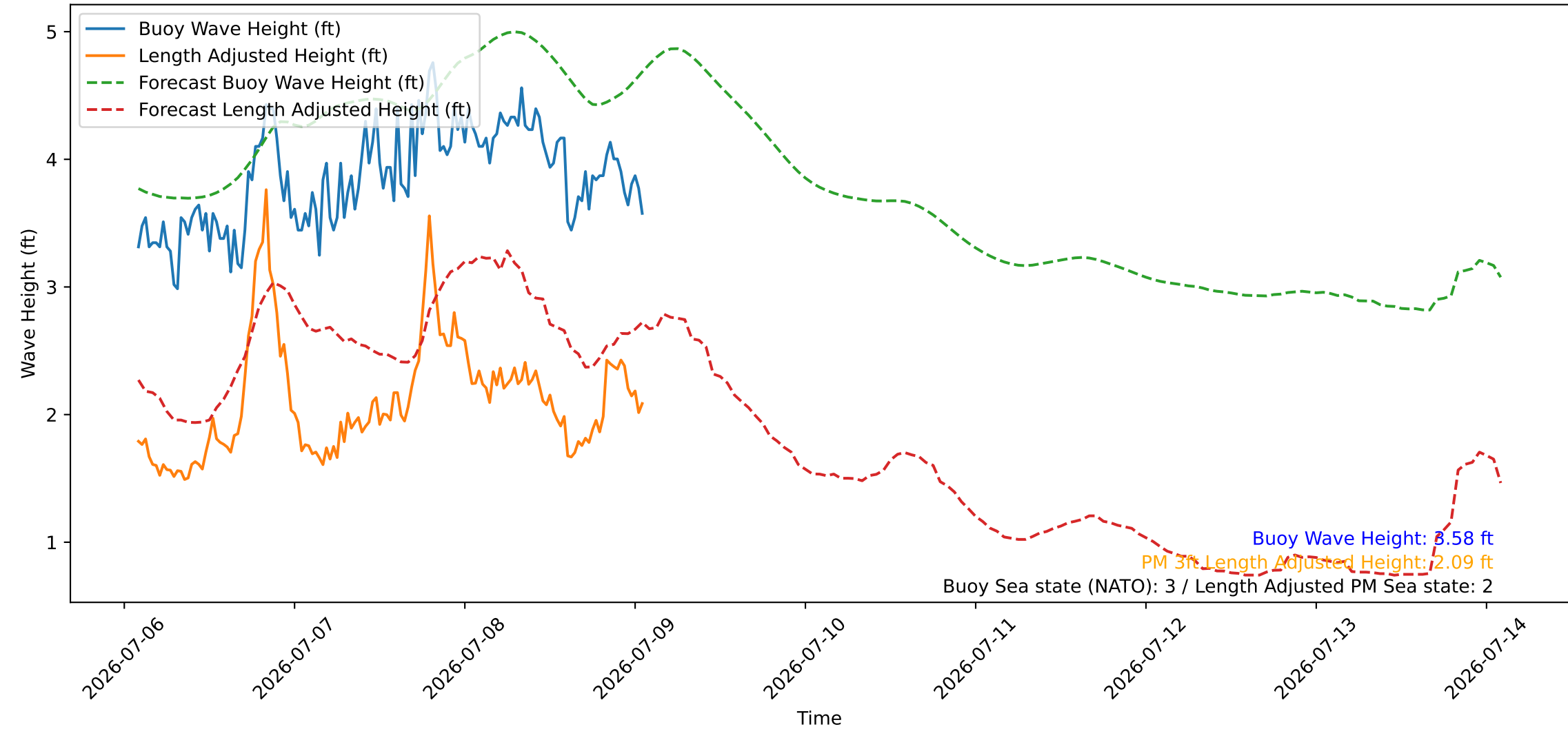
Wave Heights over Time for Green Beach at 2026-07-09 02:01:08
