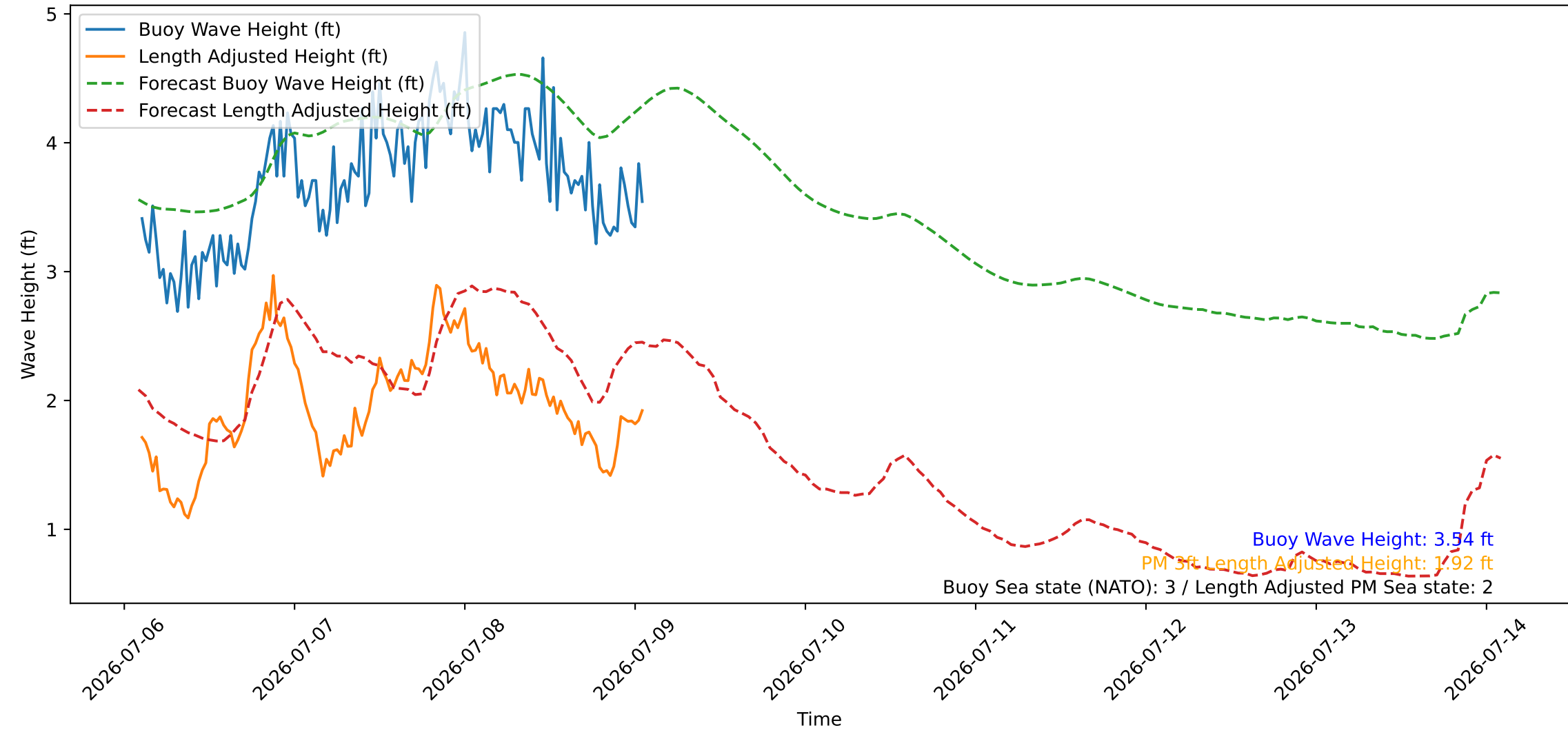
Wave Heights over Time for Red Beach at 2026-07-09 02:00:46
