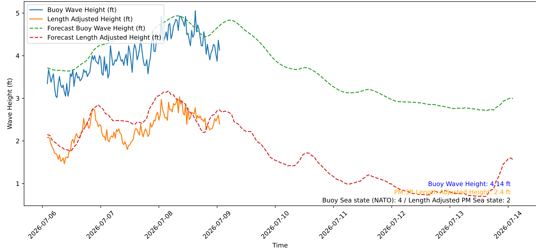
Wave Heights over Time for Oceanside Harbor at 2026-07-09 02:00:26
