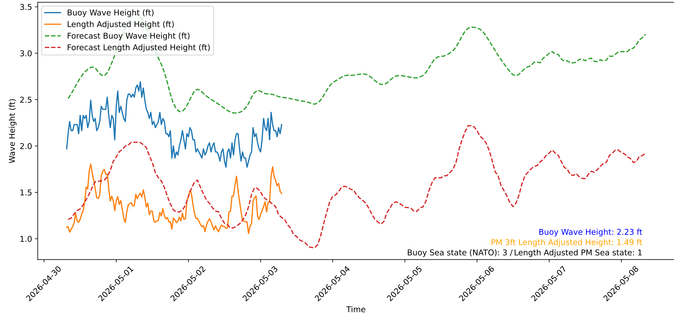
Wave Heights over Time for Oceanside Harbor at 2026-05-03 07:30:31
