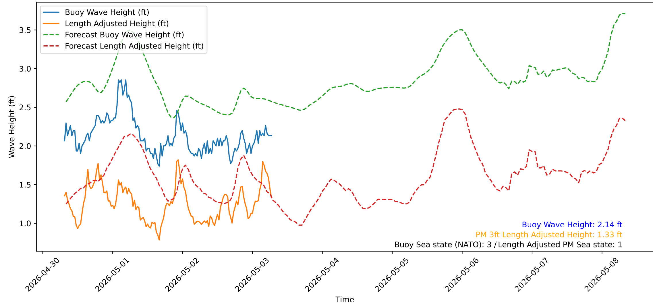
Wave Heights over Time for Green Beach at 2026-05-03 07:31:13
