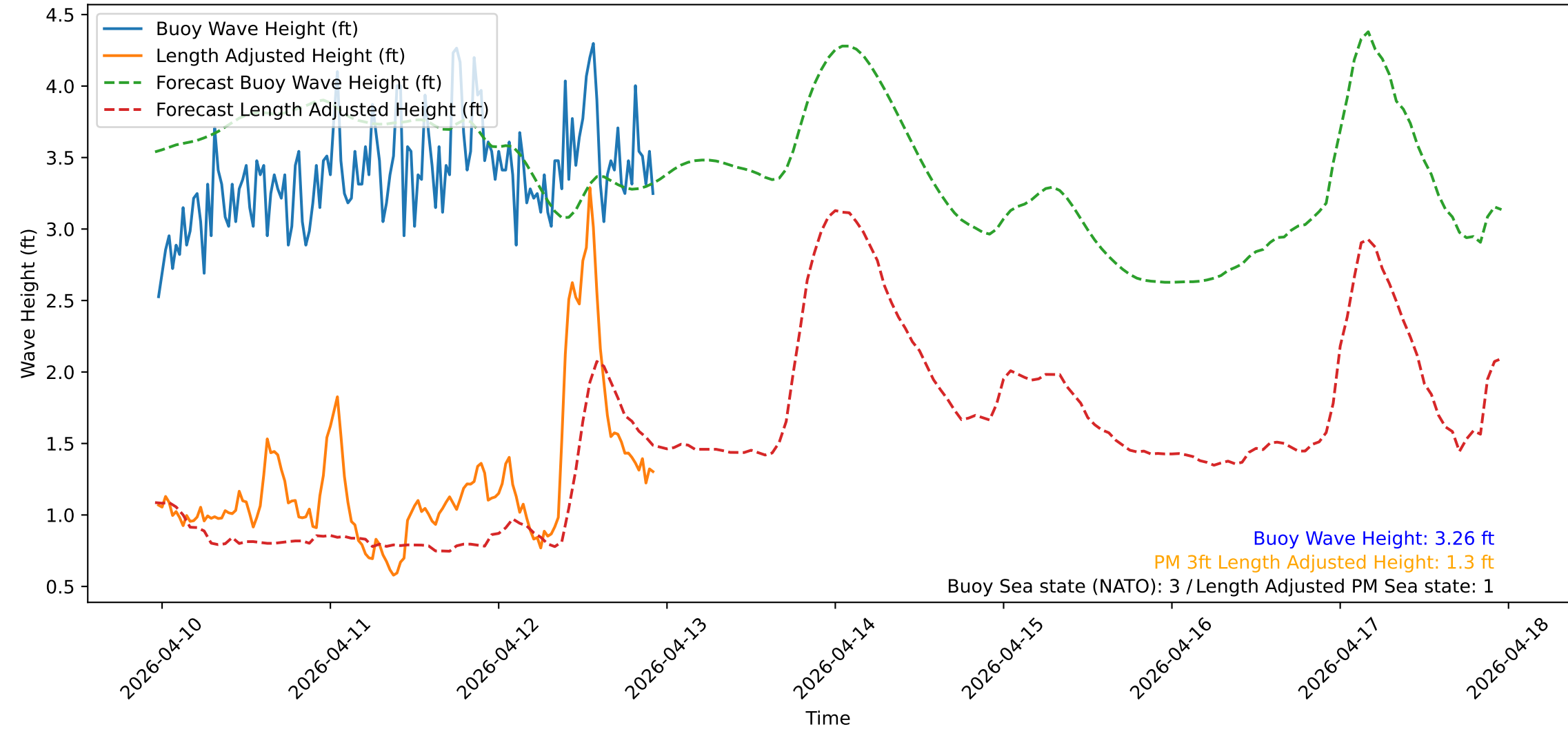
Wave Heights over Time for Red Beach at 2026-04-12 23:00:50
