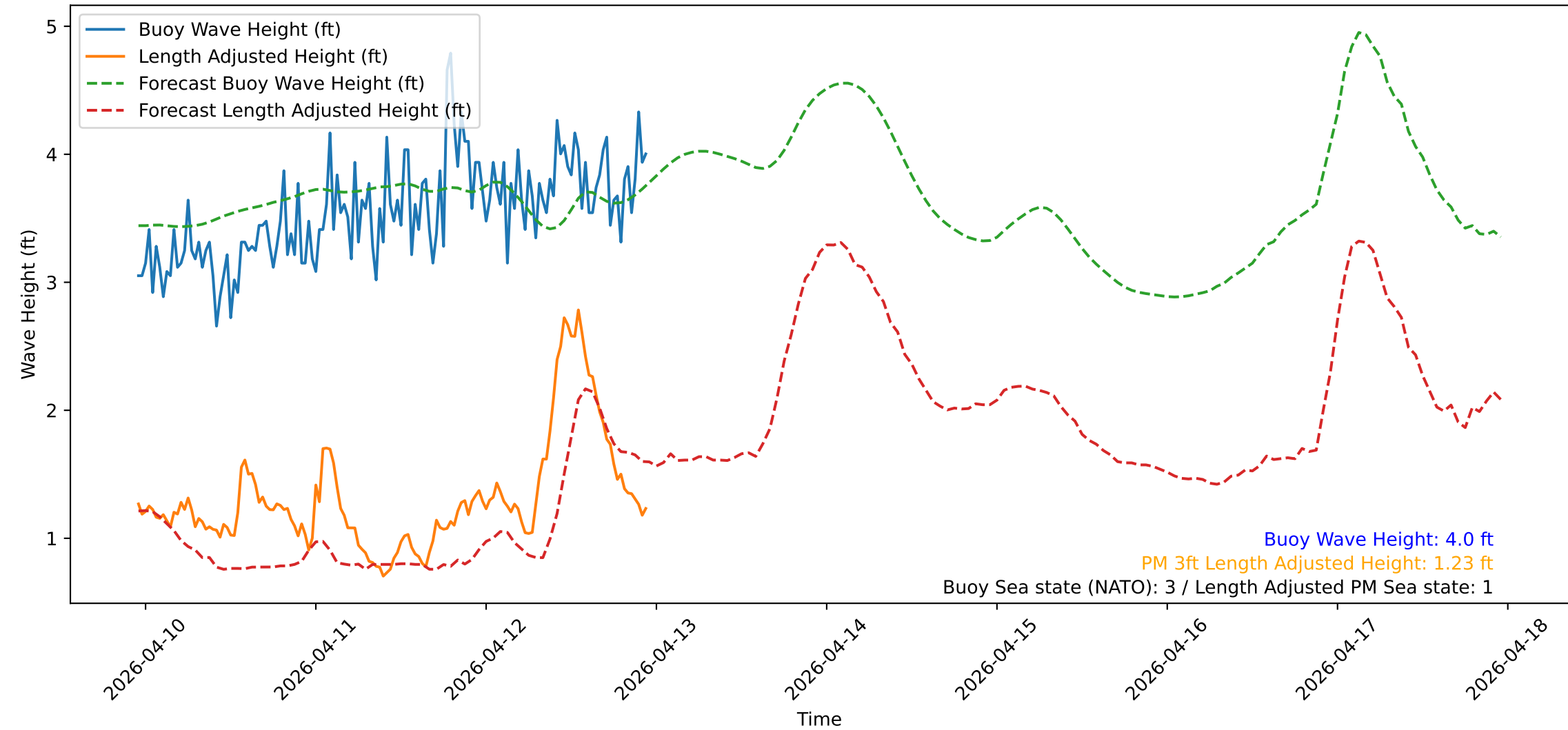
Wave Heights over Time for Oceanside Harbor at 2026-04-12 23:00:31
