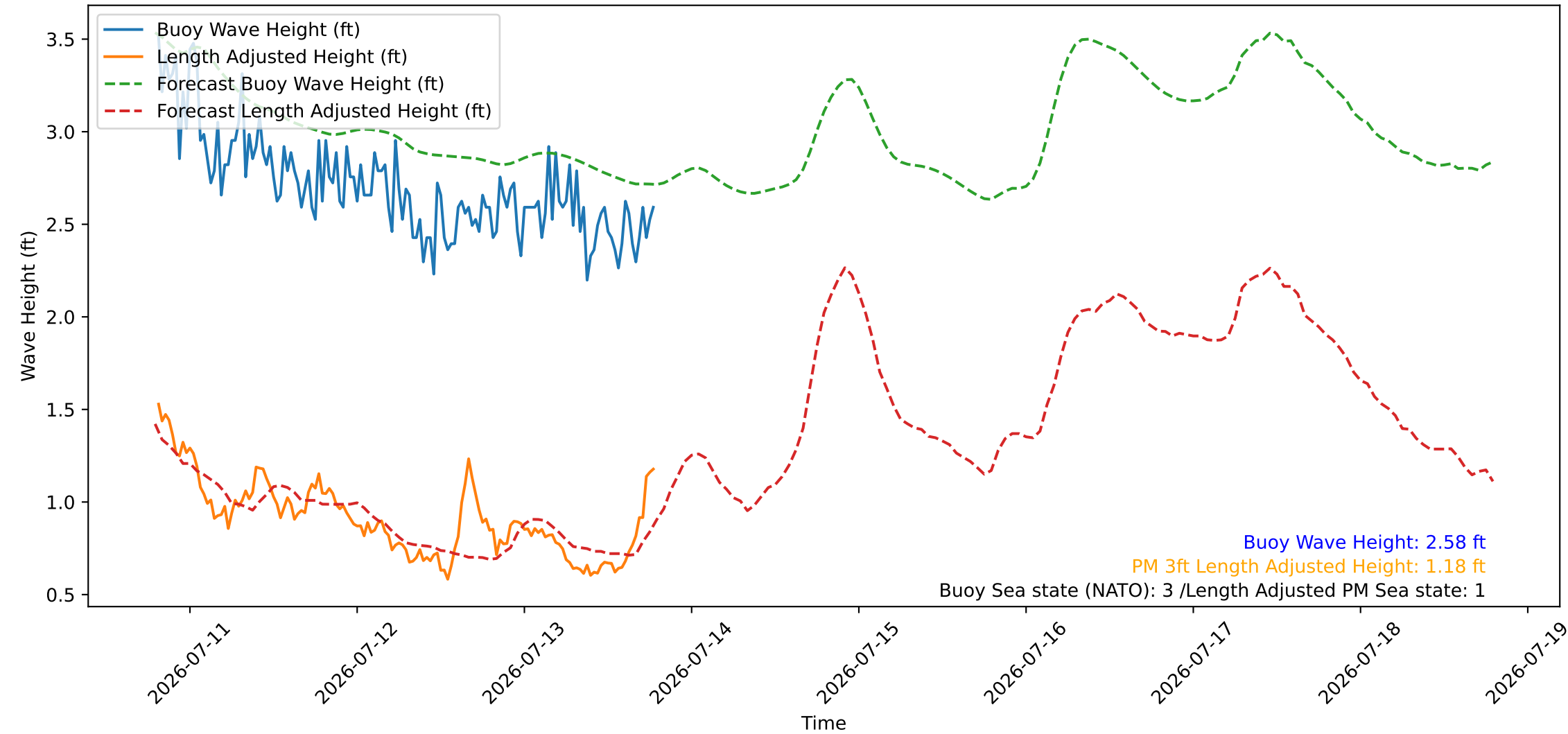
Wave Heights over Time for Green Beach at 2026-07-13 19:21:11
