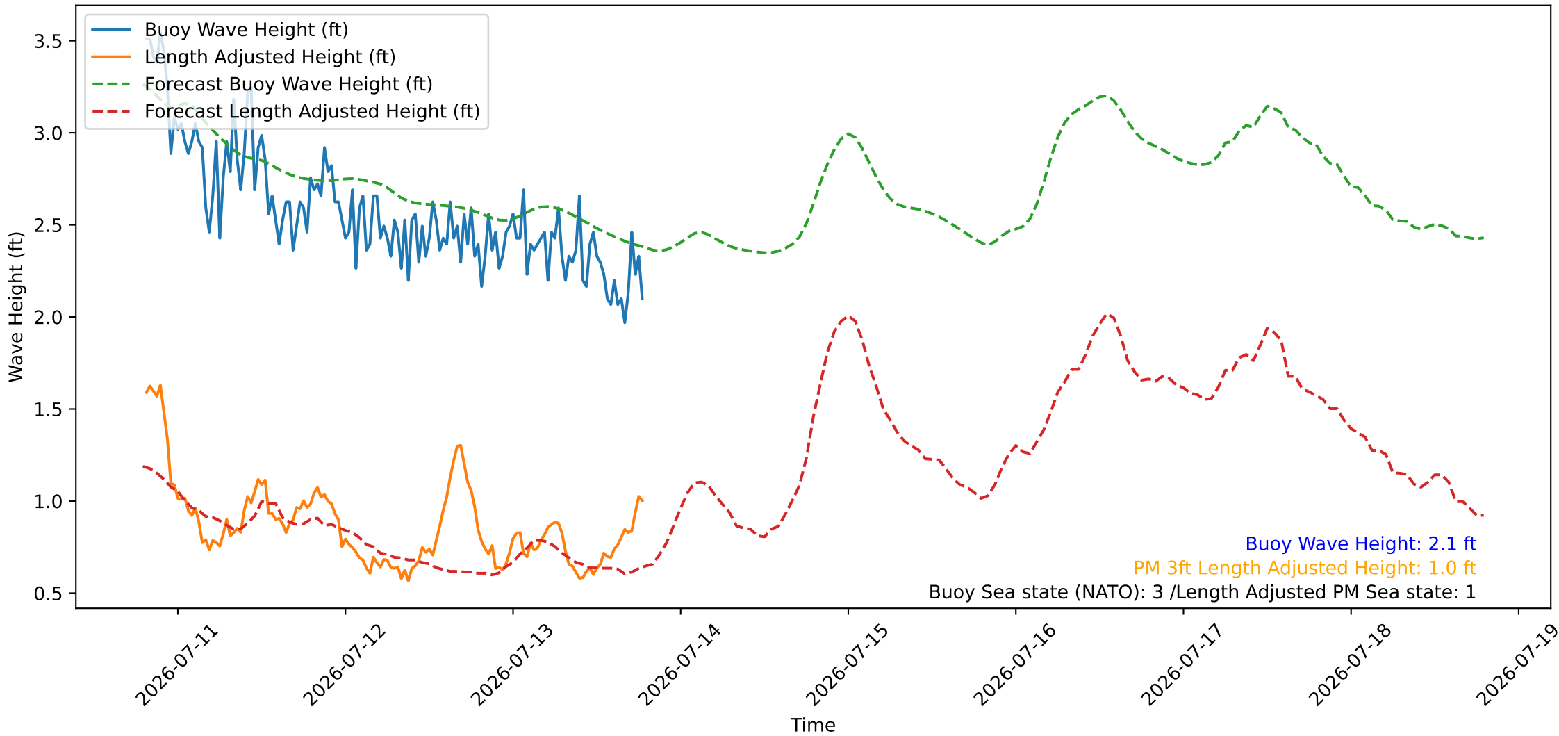
Wave Heights over Time for Red Beach at 2026-07-13 19:20:48
