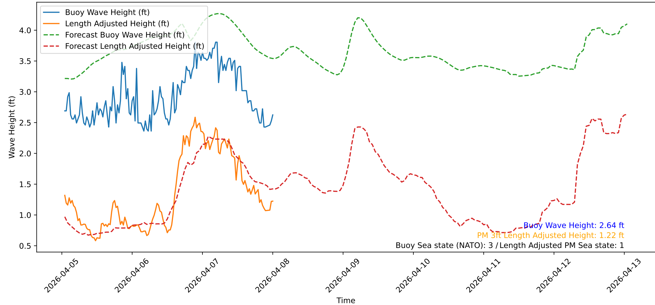
Wave Heights over Time for Green Beach at 2026-04-08 00:51:09
