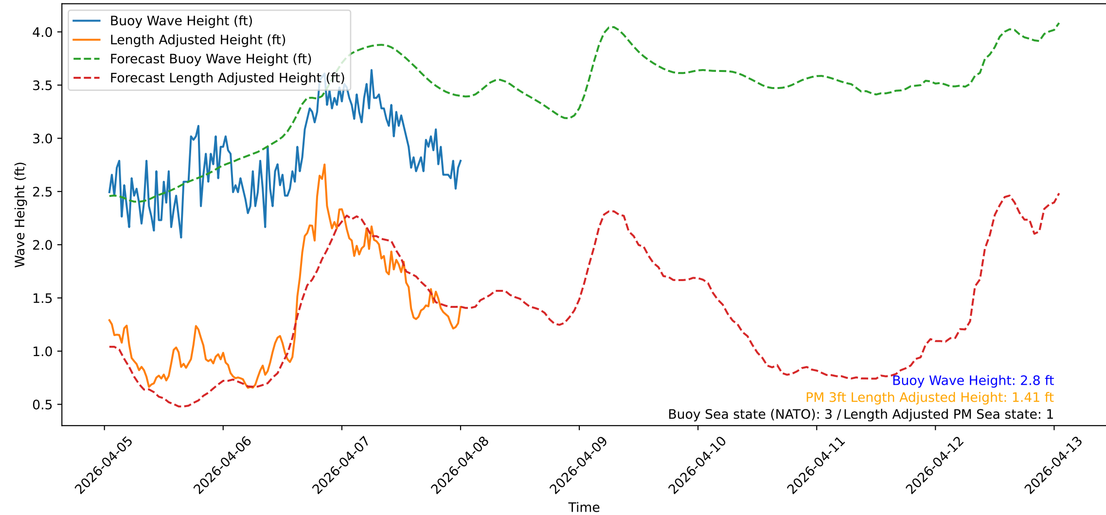
Wave Heights over Time for Oceanside Harbor at 2026-04-08 00:50:31
