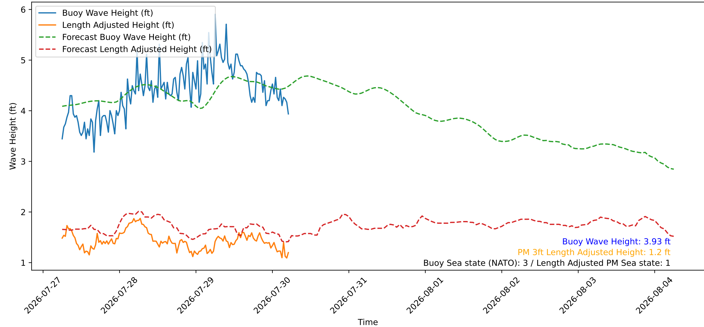
Wave Heights over Time for Oceanside Harbor at 2026-07-30 06:00:26
