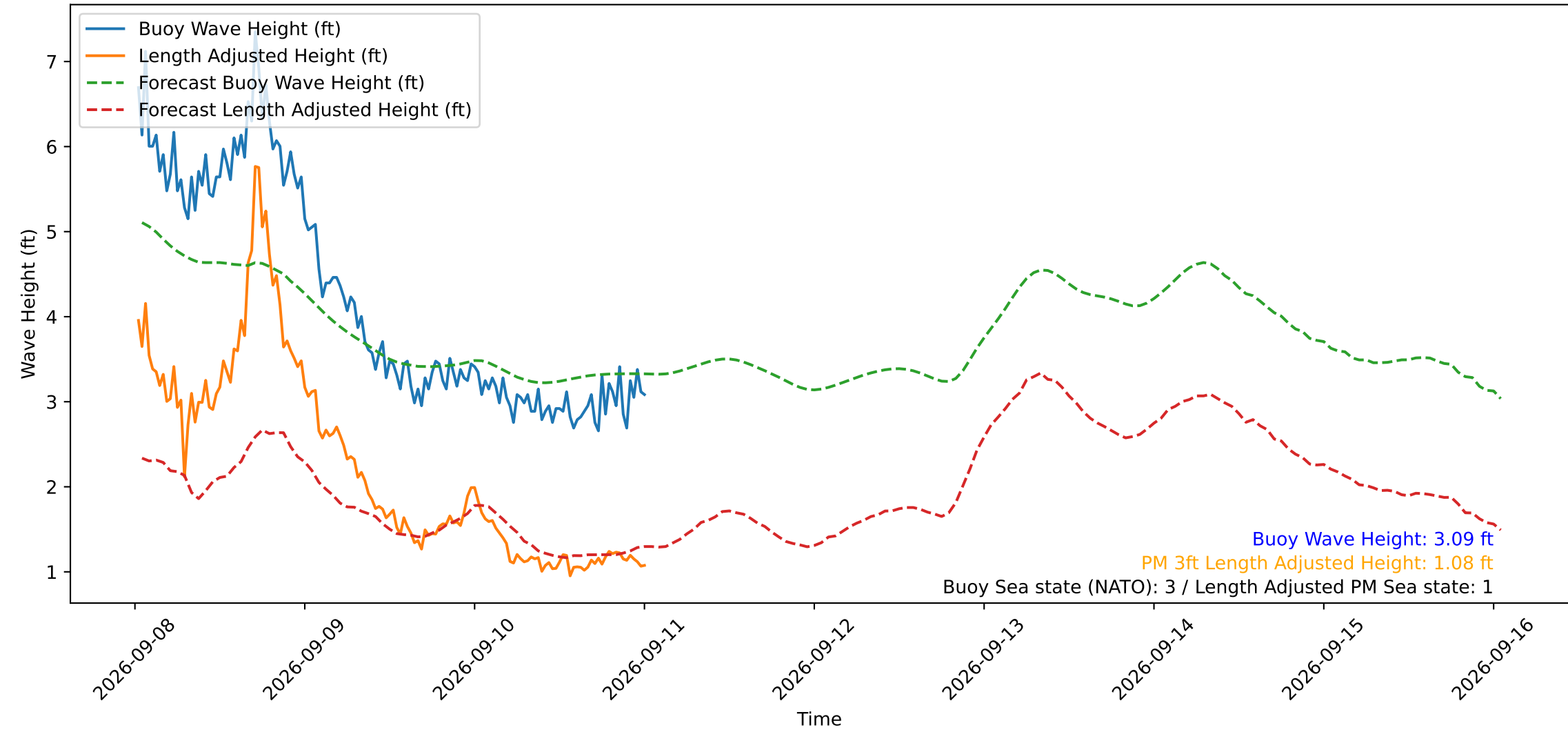
Wave Heights over Time for Oceanside Harbor at 2026-09-11 00:40:30
