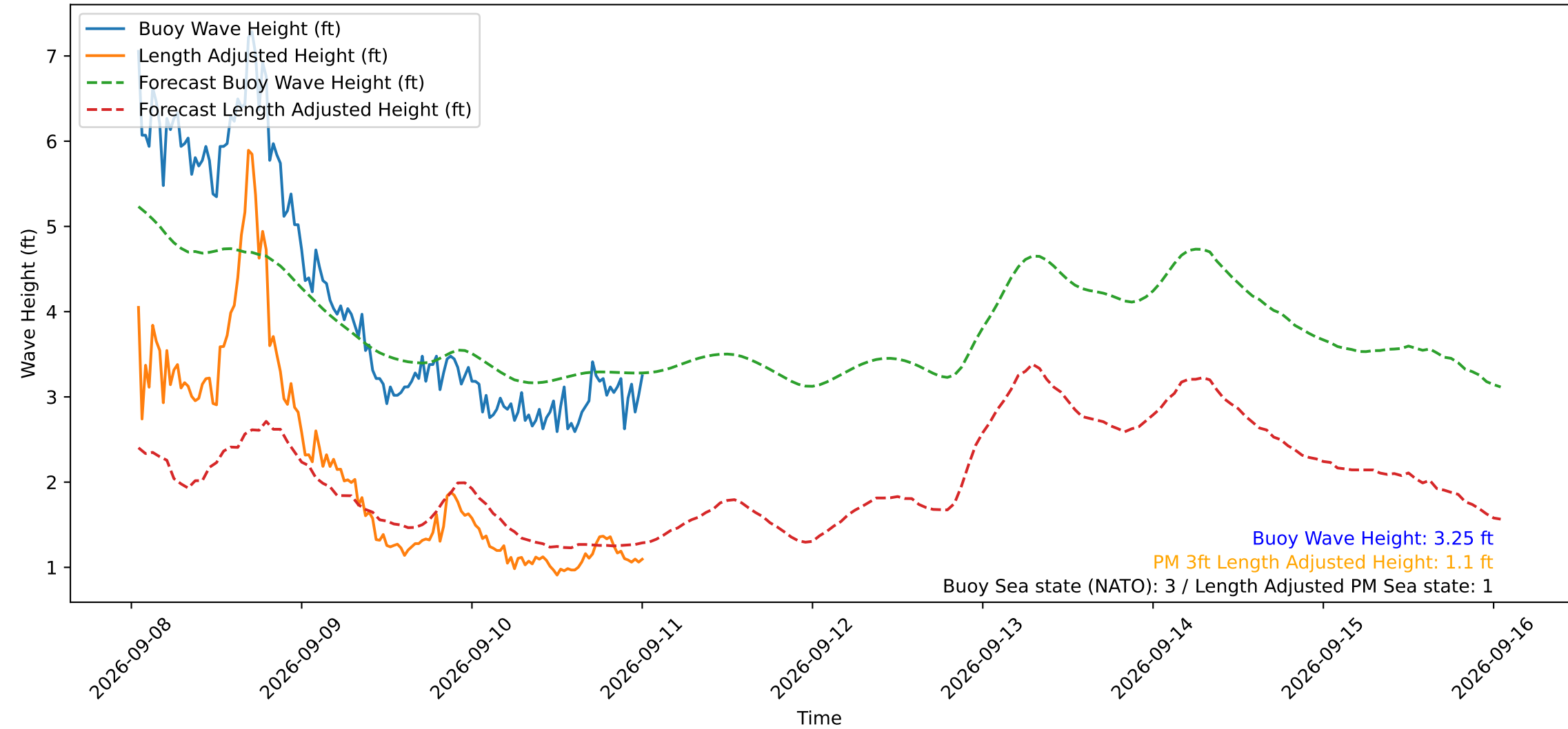
Wave Heights over Time for Green Beach at 2026-09-11 00:41:12
