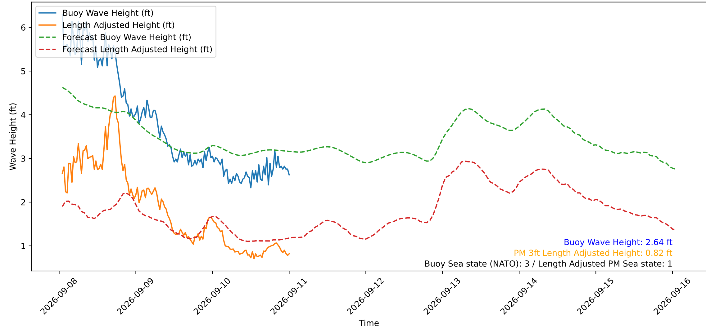
Wave Heights over Time for Red Beach at 2026-09-11 00:40:49
