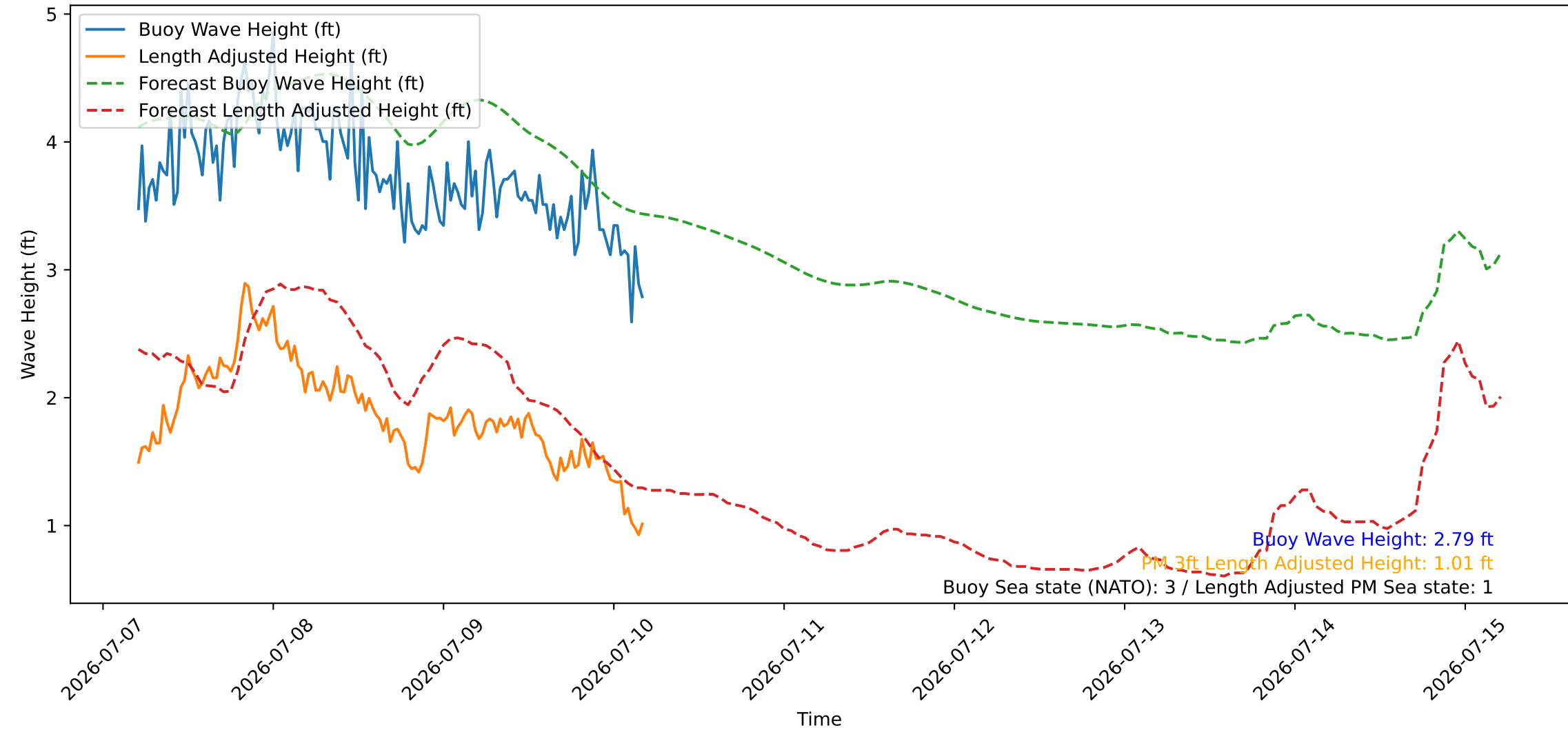
Wave Heights over Time for Red Beach at 2026-07-10 04:40:45
