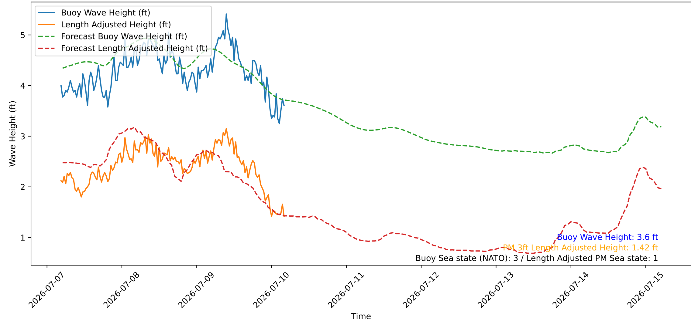
Wave Heights over Time for Oceanside Harbor at 2026-07-10 04:40:25
