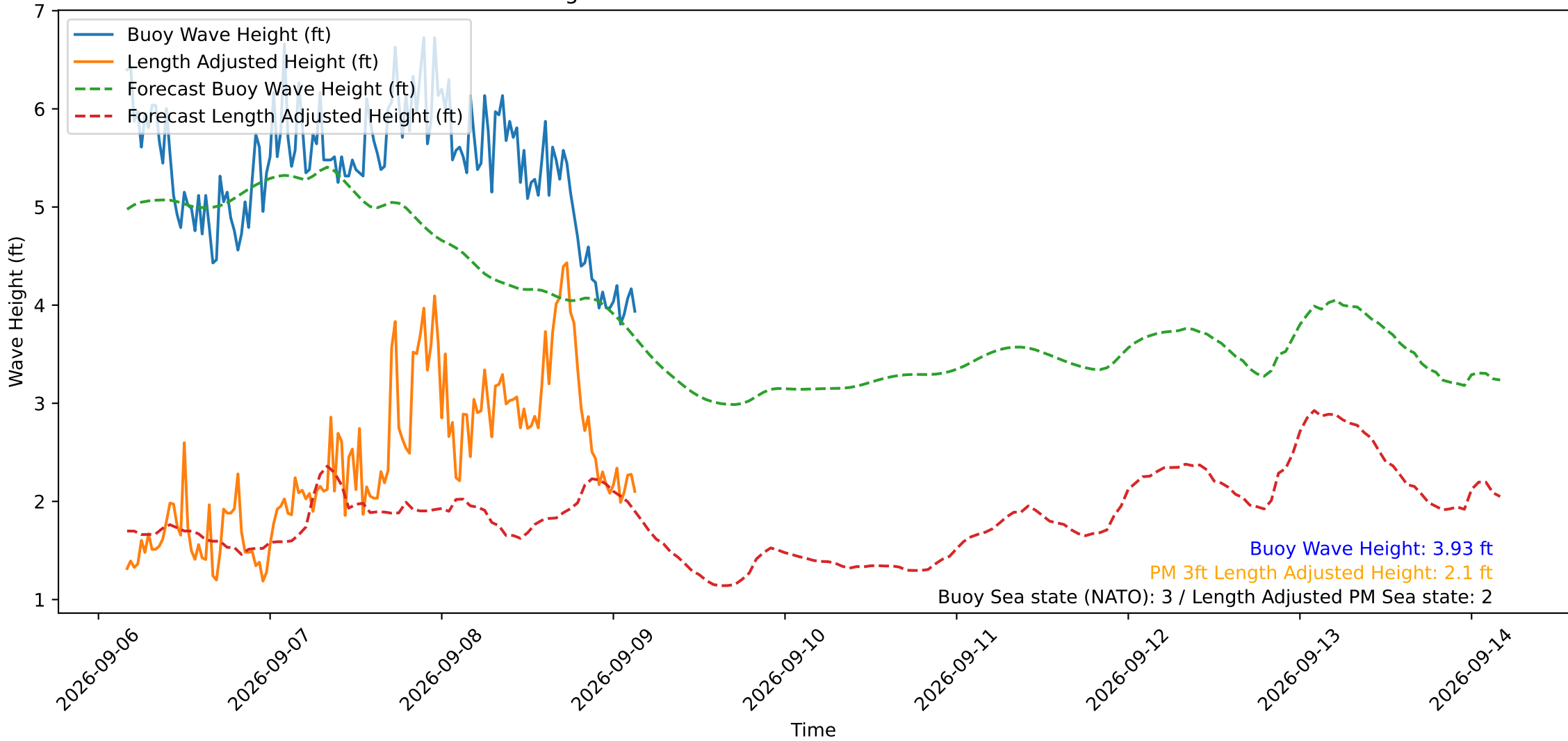
Wave Heights over Time for Red Beach at 2026-09-09 03:40:49
