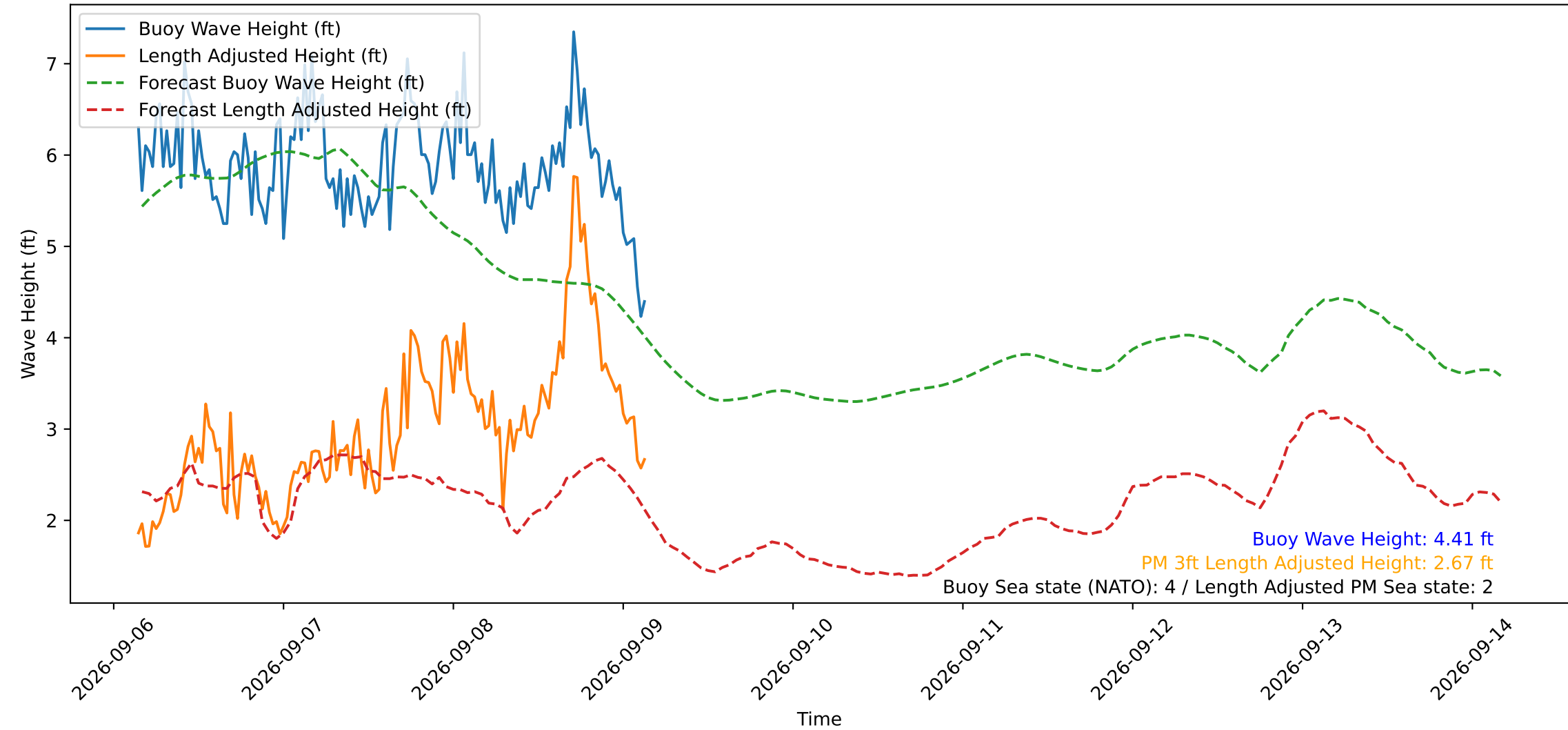
Wave Heights over Time for Oceanside Harbor at 2026-09-09 03:40:29
