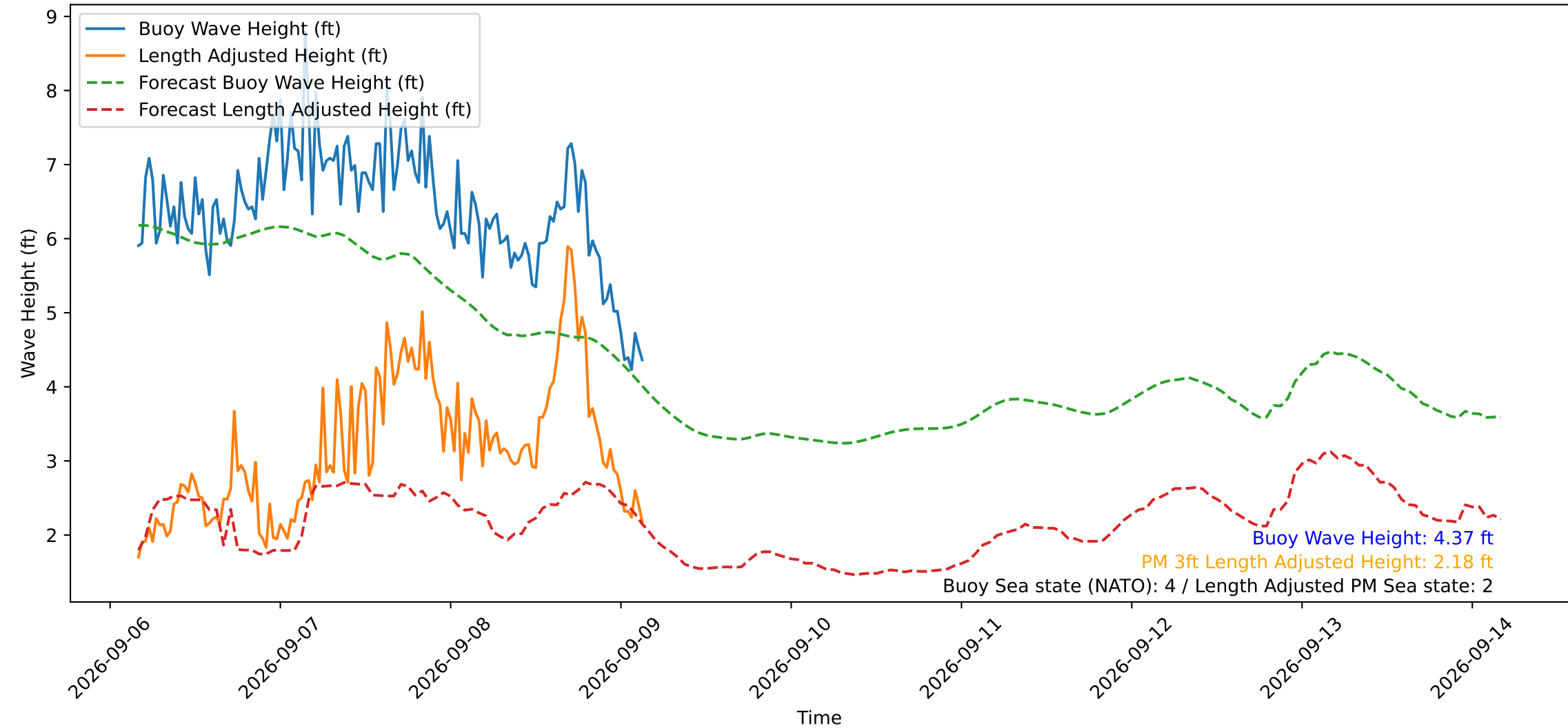
Wave Heights over Time for Green Beach at 2026-09-09 03:41:12
