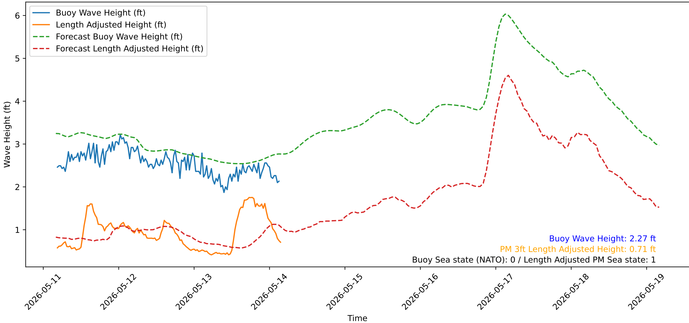
Wave Heights over Time for Red Beach at 2026-05-14 04:20:52
