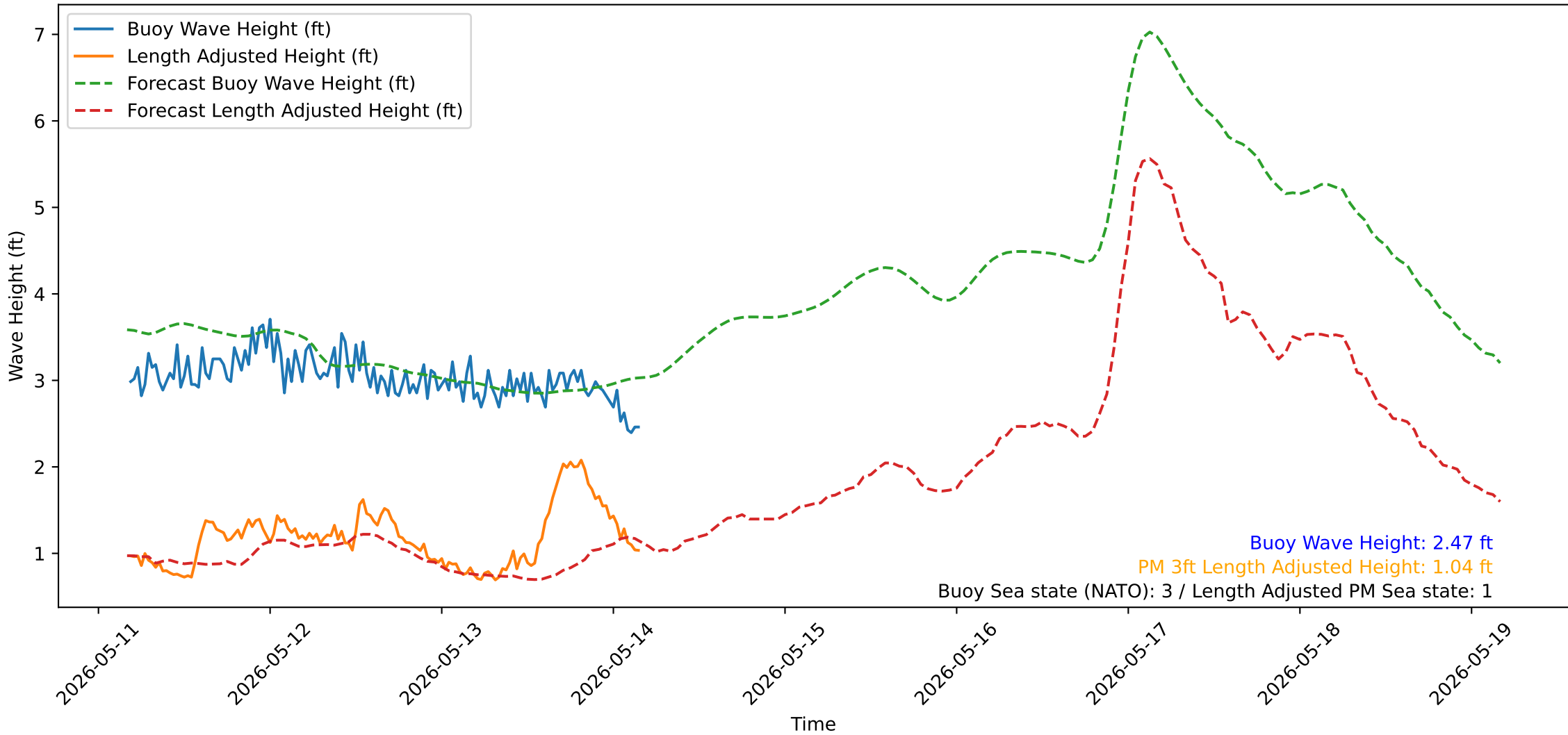
Wave Heights over Time for Oceanside Harbor at 2026-05-14 04:20:32
