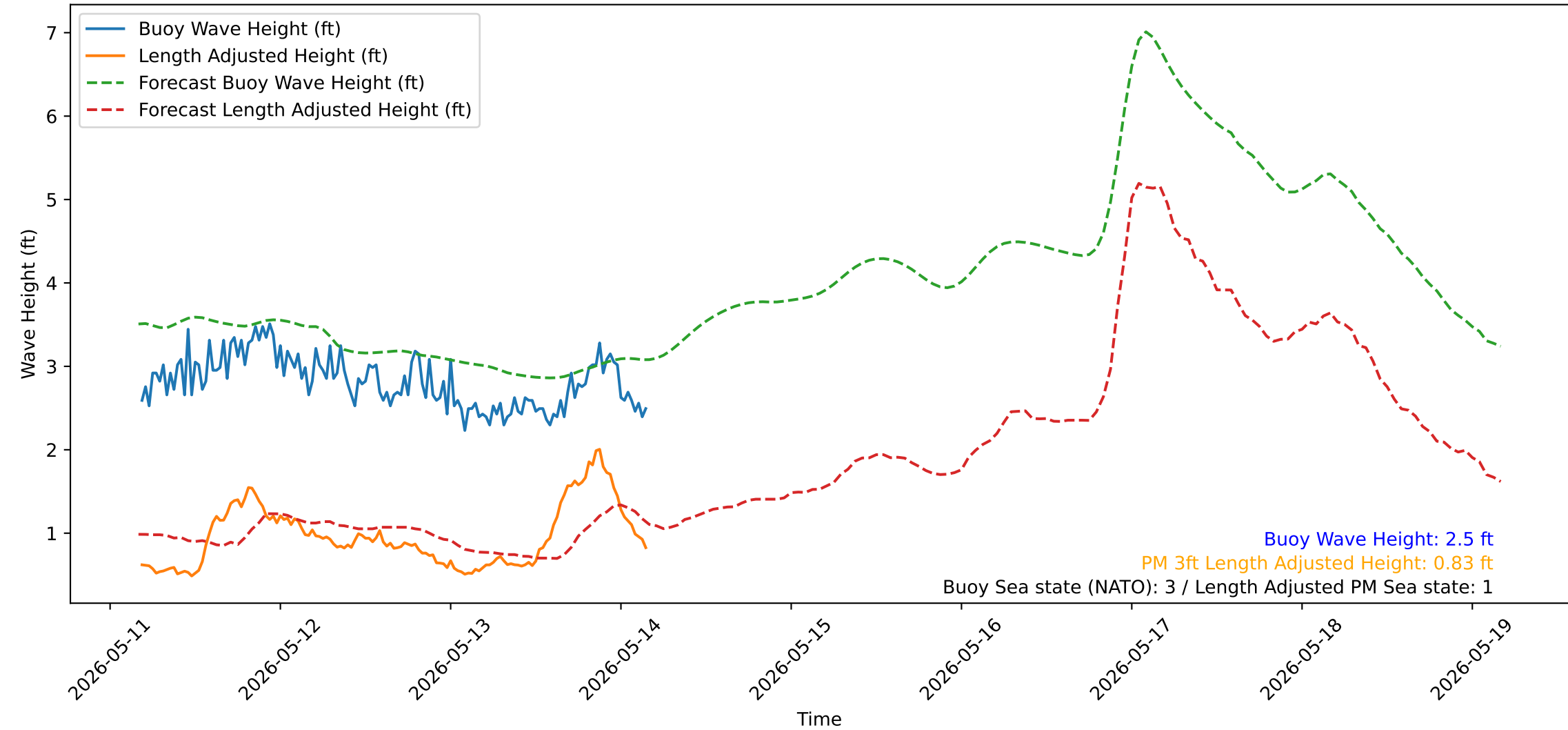
Wave Heights over Time for Green Beach at 2026-05-14 04:21:15
