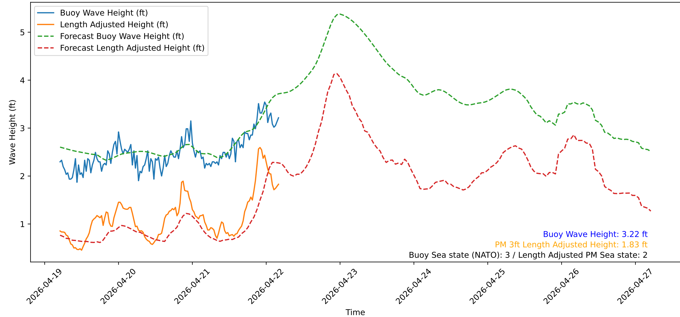
Wave Heights over Time for Green Beach at 2026-04-22 05:01:12
