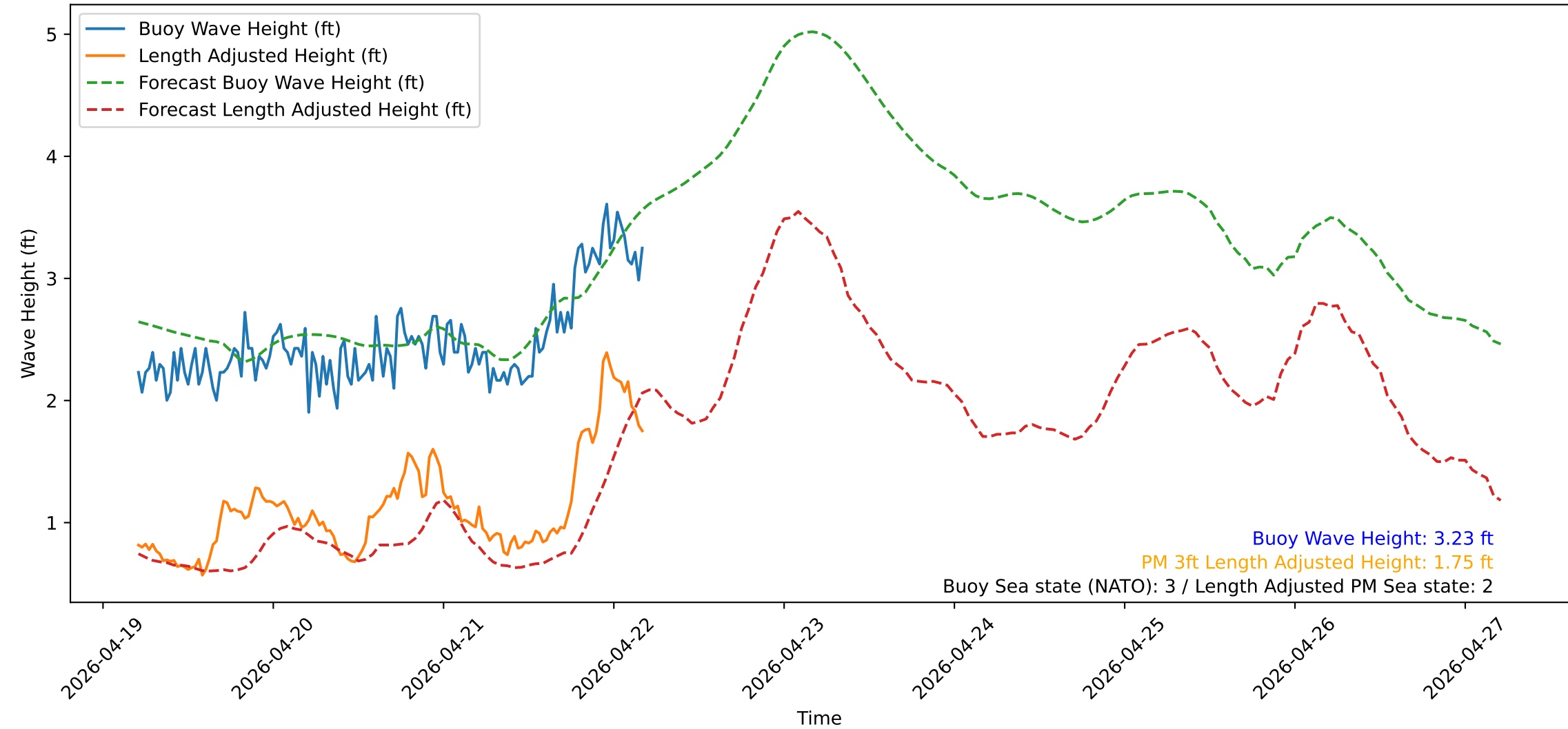
Wave Heights over Time for Oceanside Harbor at 2026-04-22 05:00:31
