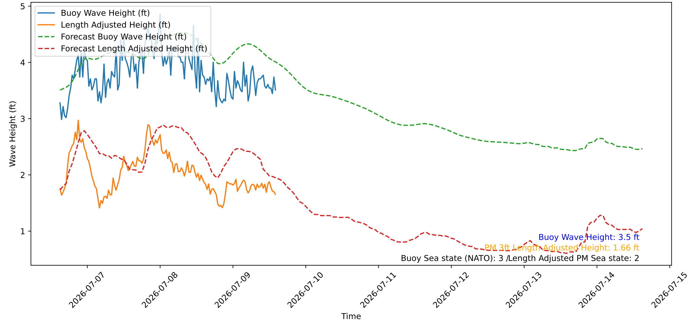
Wave Heights over Time for Red Beach at 2026-07-09 14:40:46
