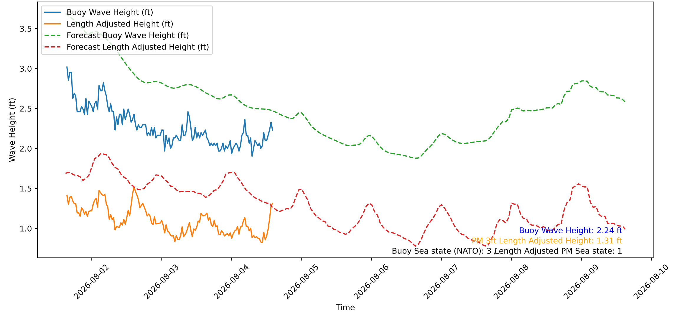
Wave Heights over Time for Red Beach at 2026-08-04 15:10:46
