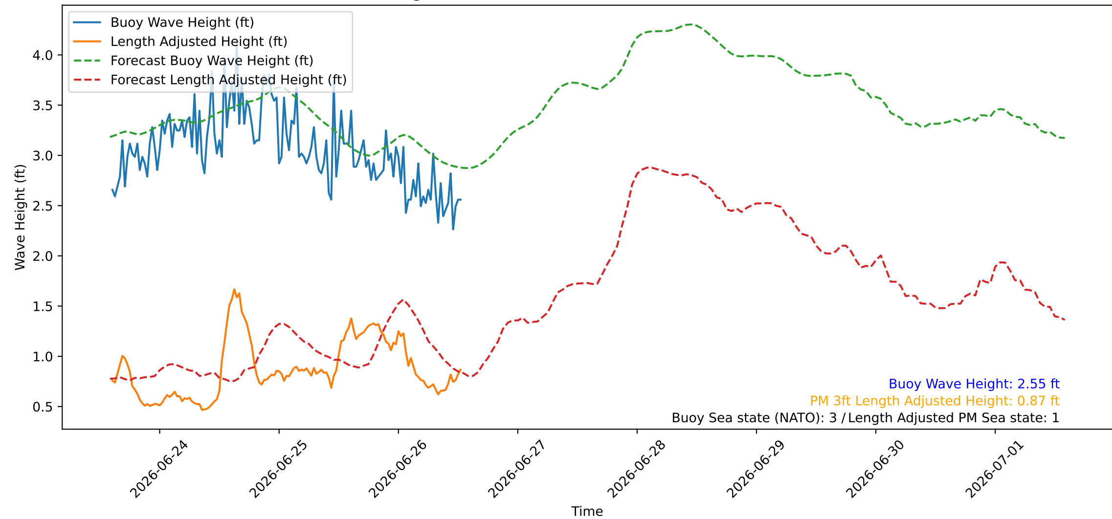
Wave Heights over Time for Red Beach at 2026-06-26 14:00:45
