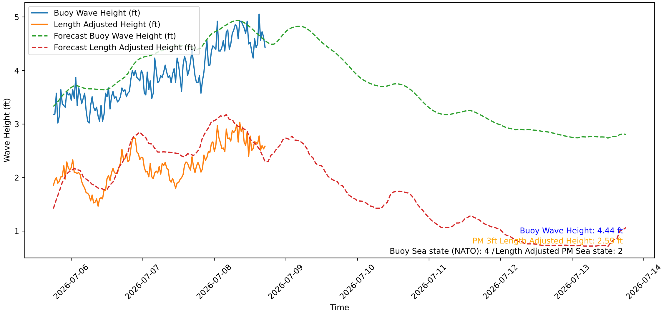
Wave Heights over Time for Oceanside Harbor at 2026-07-08 17:50:27
