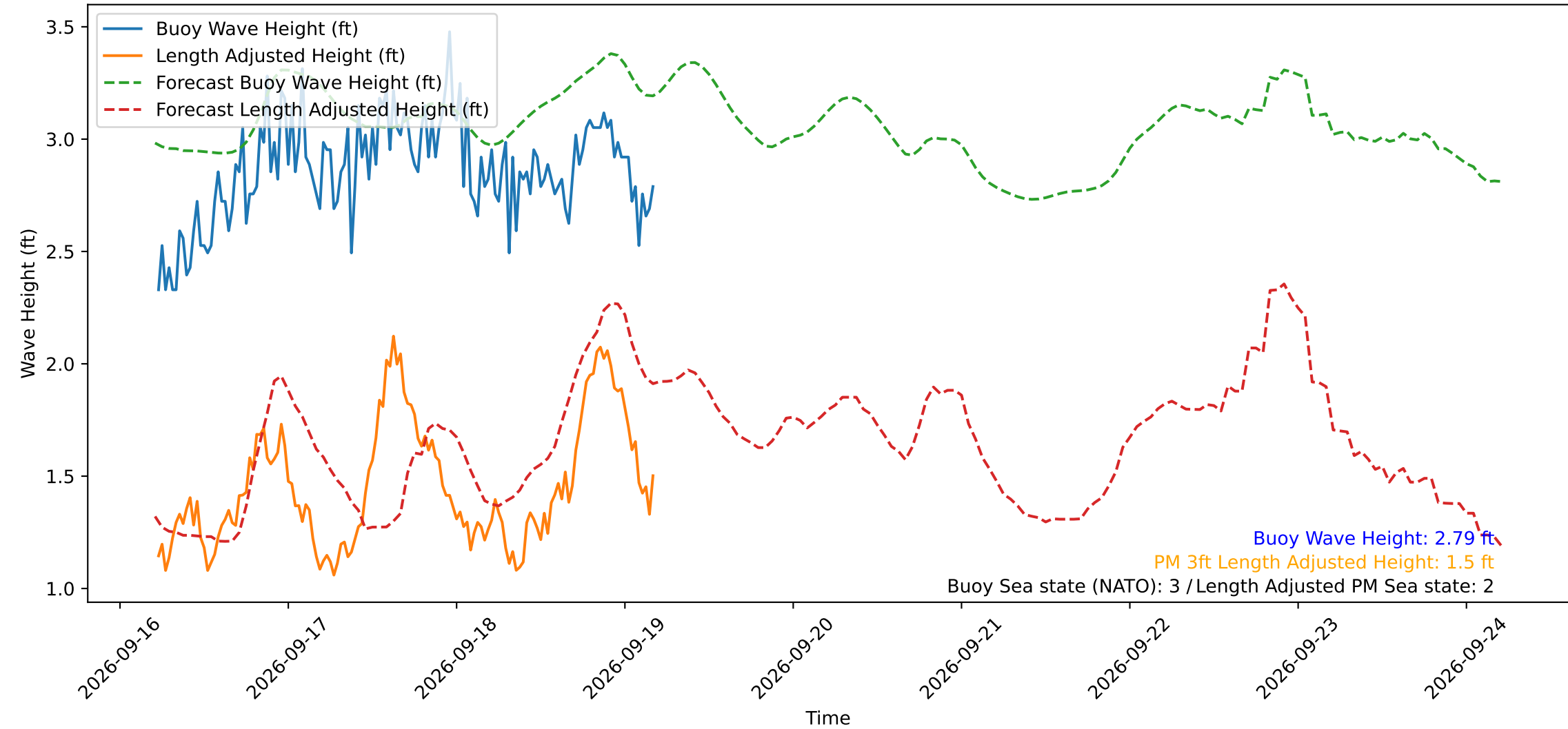
Wave Heights over Time for Green Beach at 2026-09-19 05:01:11
