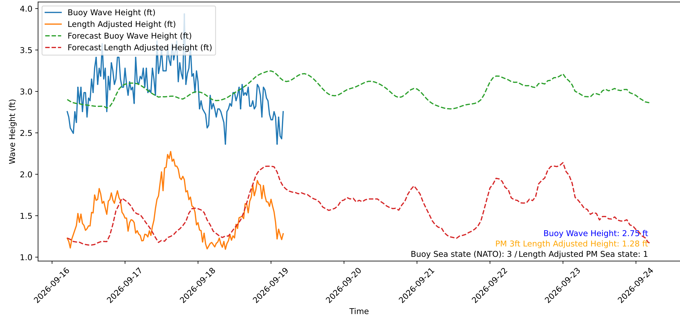
Wave Heights over Time for Oceanside Harbor at 2026-09-19 05:00:29
