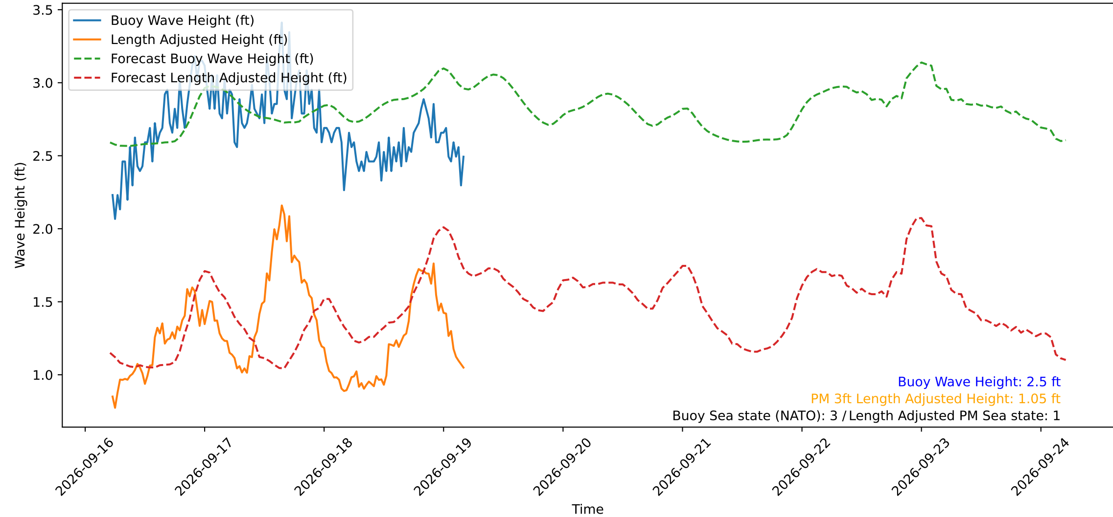
Wave Heights over Time for Red Beach at 2026-09-19 05:00:49
