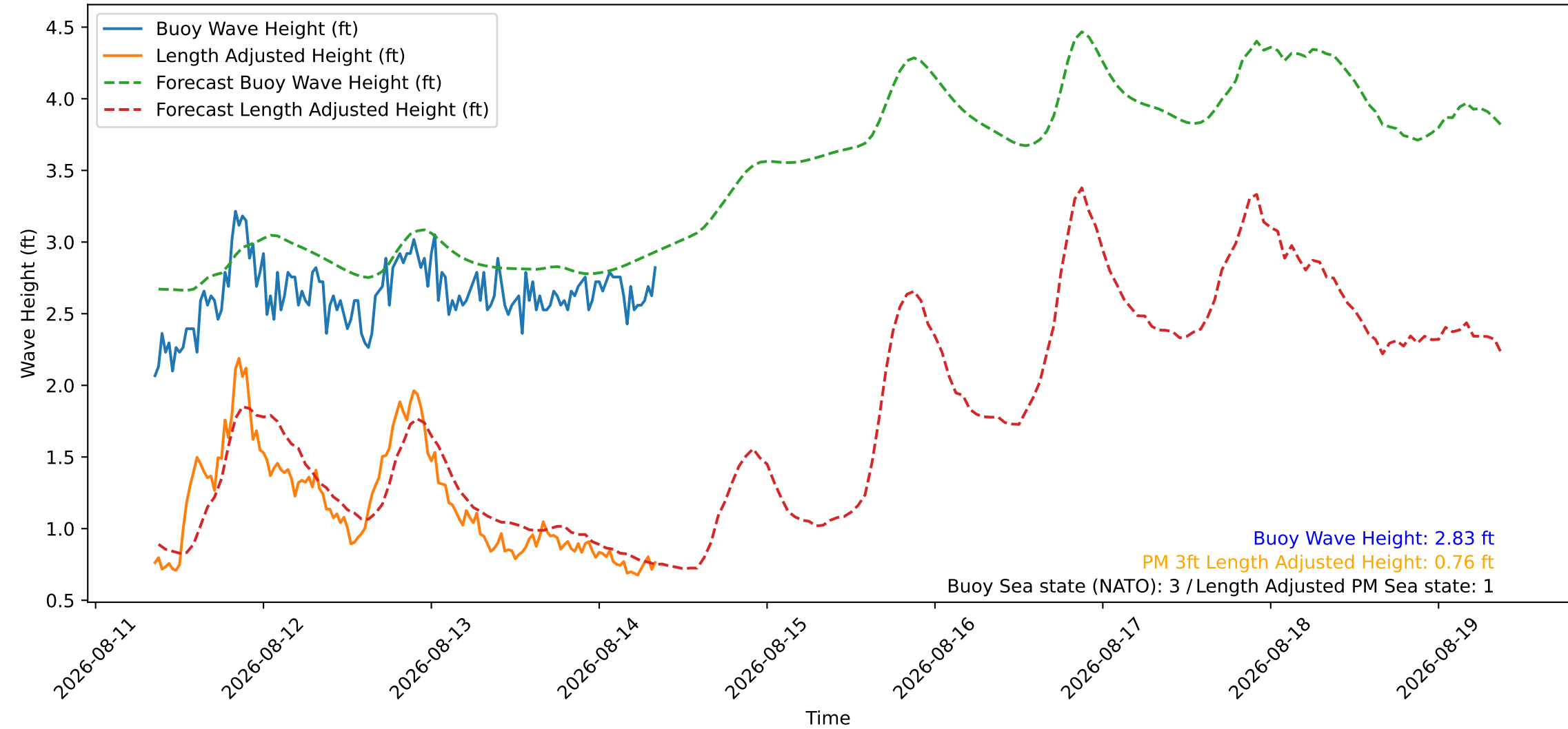
Wave Heights over Time for Green Beach at 2026-08-14 08:41:09
