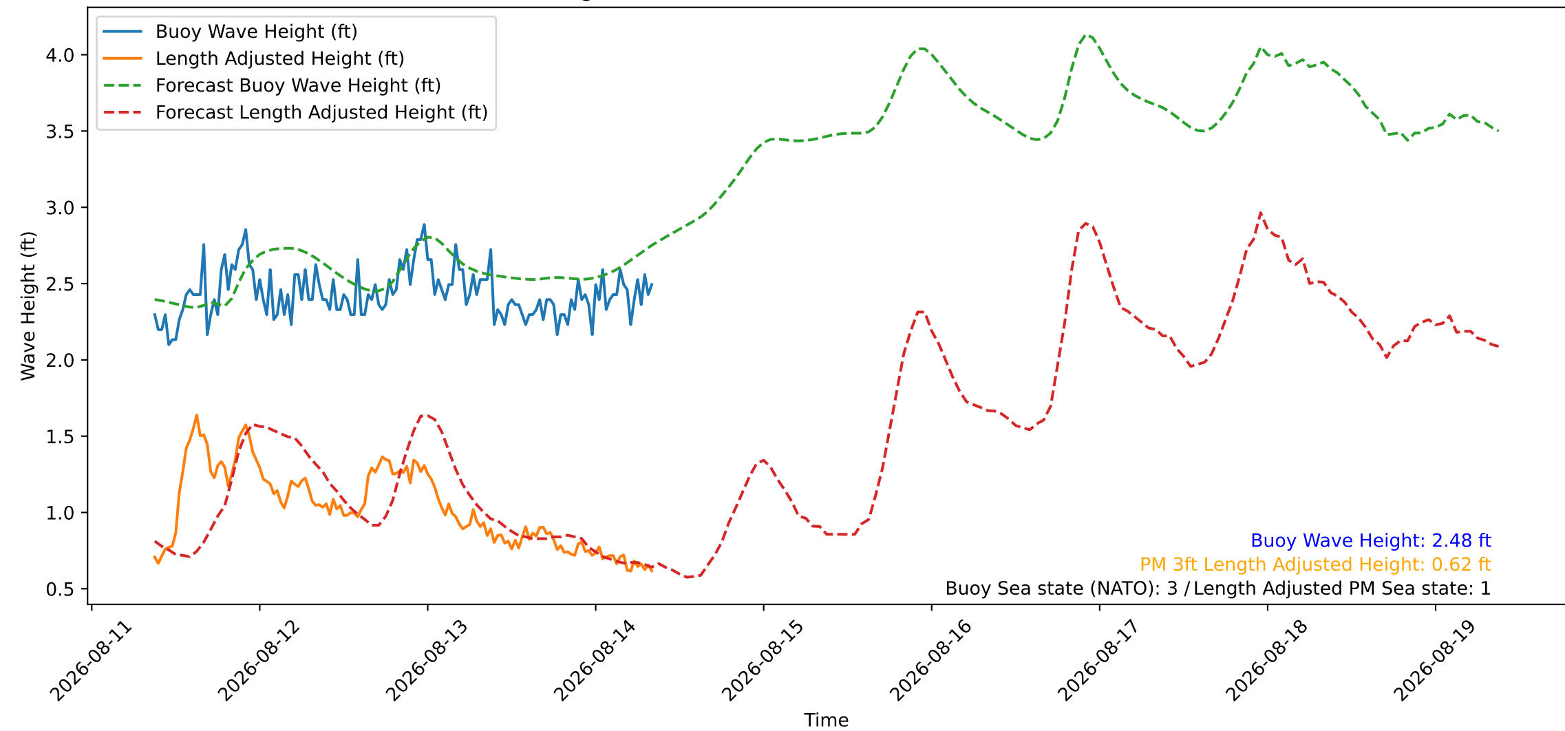
Wave Heights over Time for Red Beach at 2026-08-14 08:40:46
