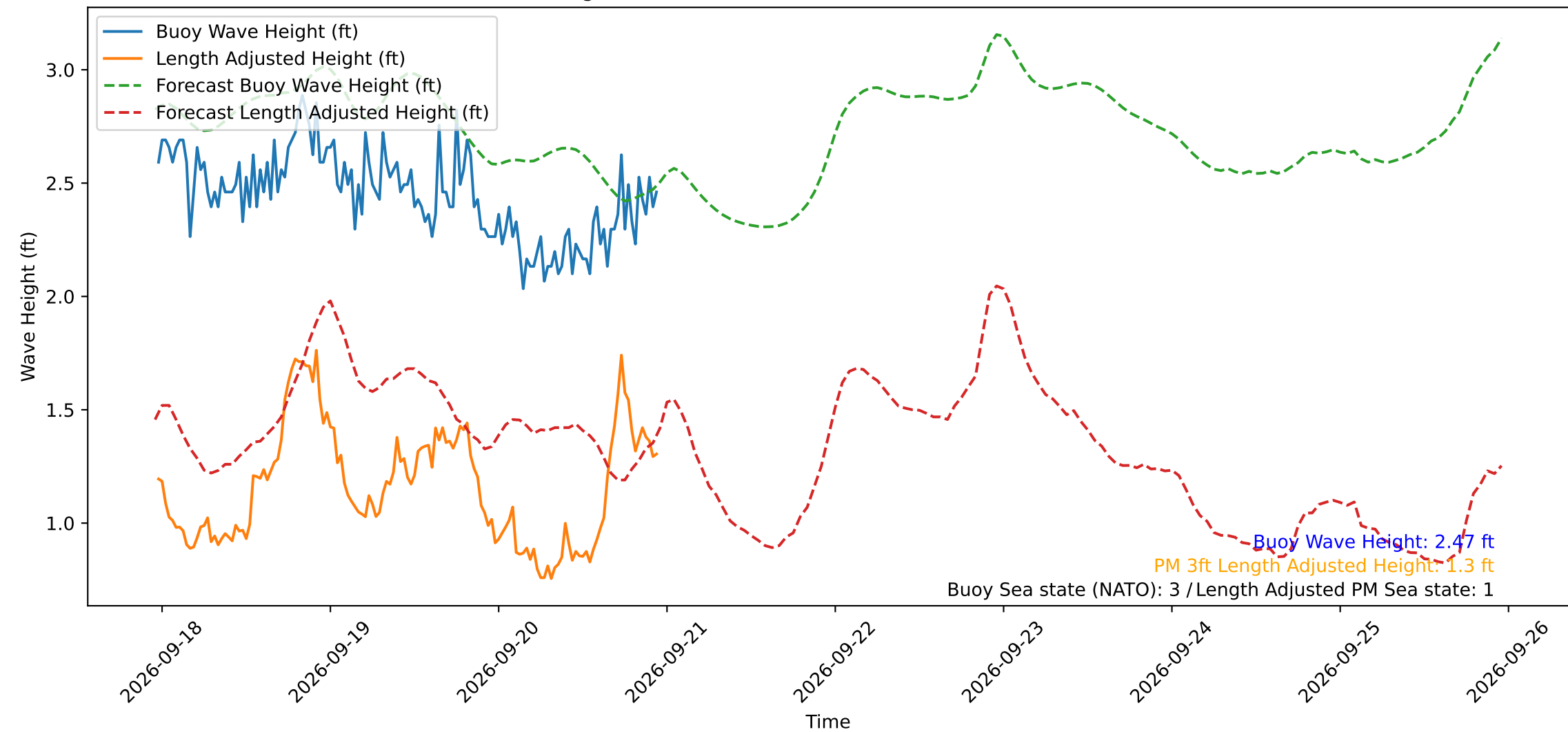
Wave Heights over Time for Red Beach at 2026-09-20 23:10:50
