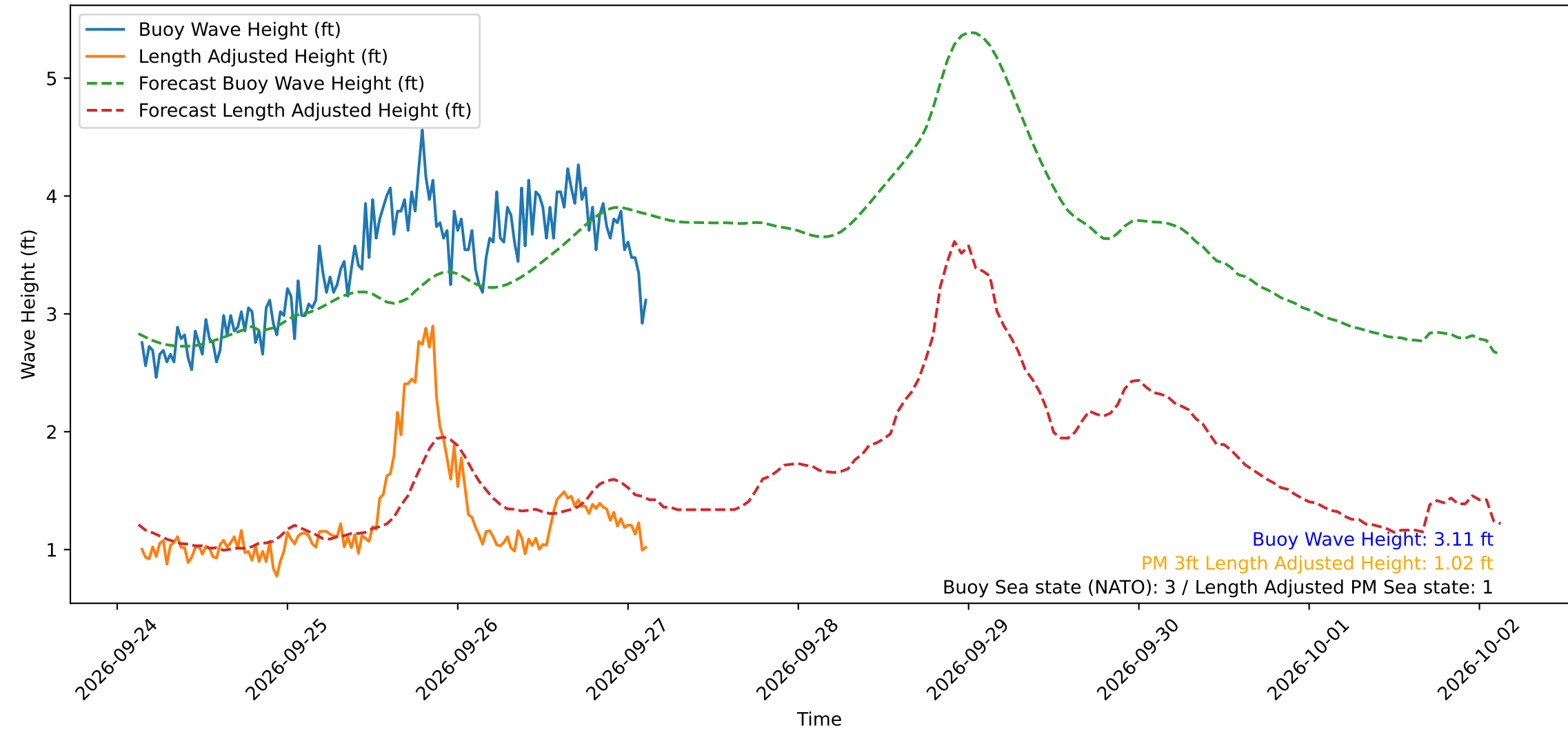
Wave Heights over Time for Green Beach at 2026-09-27 03:11:12
