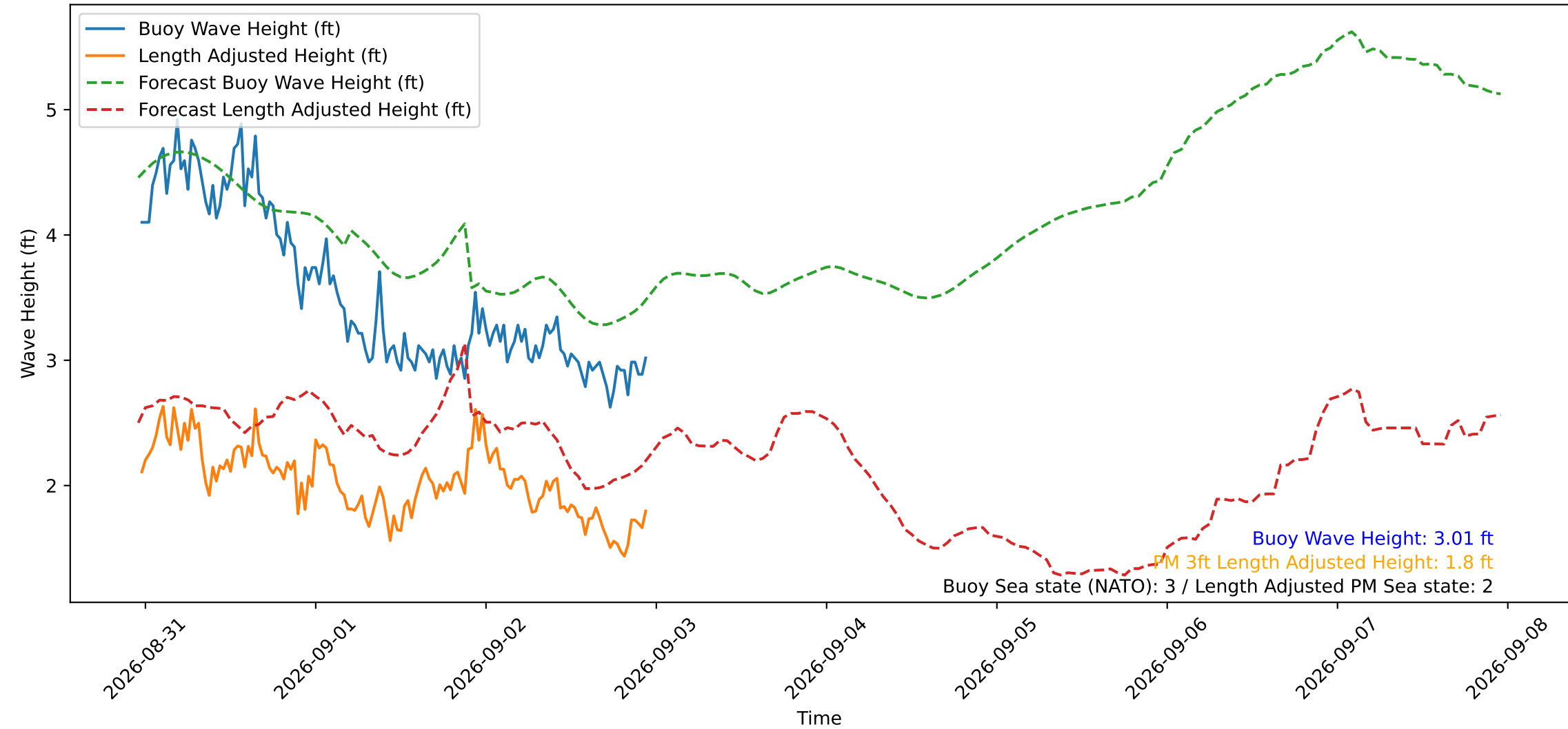
Wave Heights over Time for Oceanside Harbor at 2026-09-02 23:20:29
