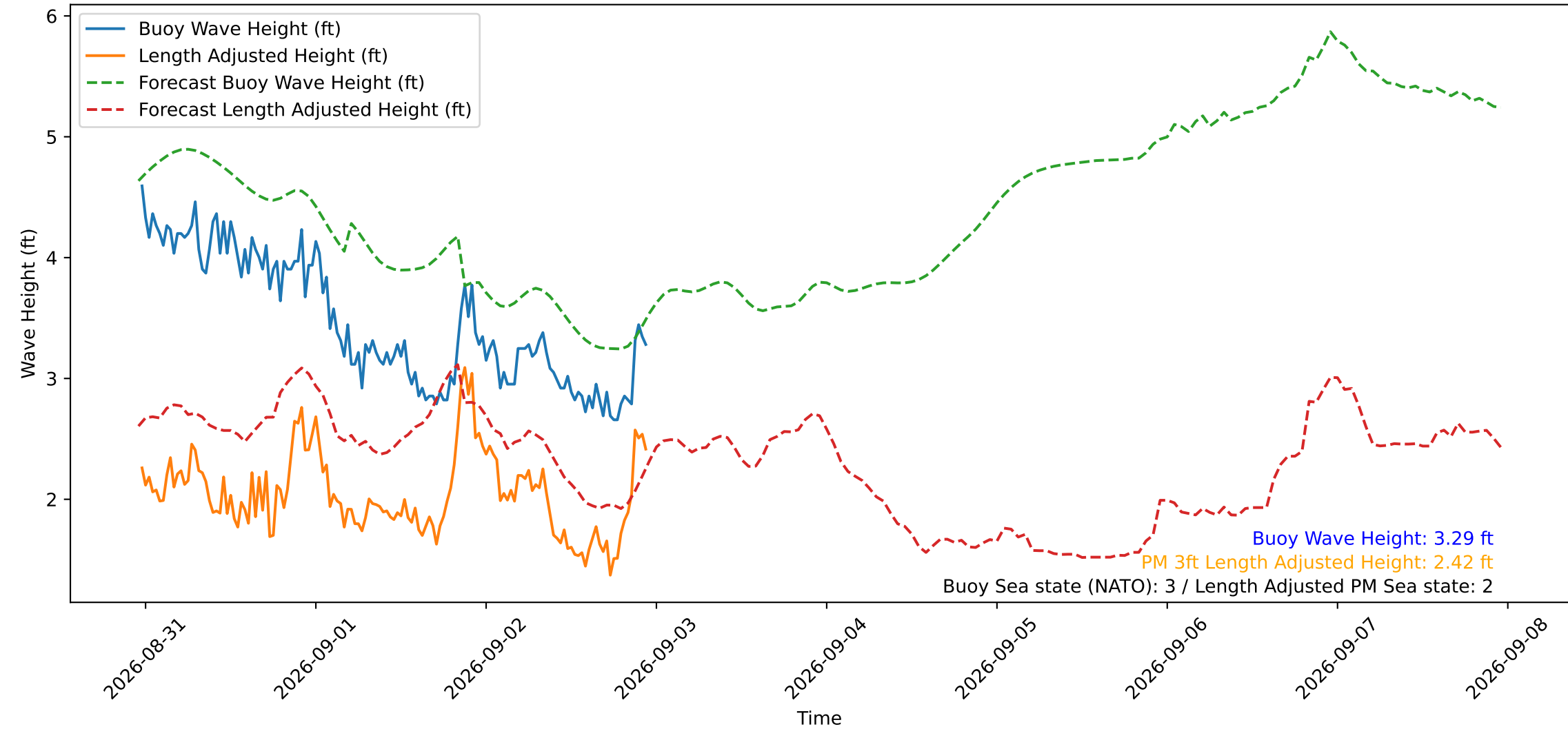
Wave Heights over Time for Green Beach at 2026-09-02 23:21:15
