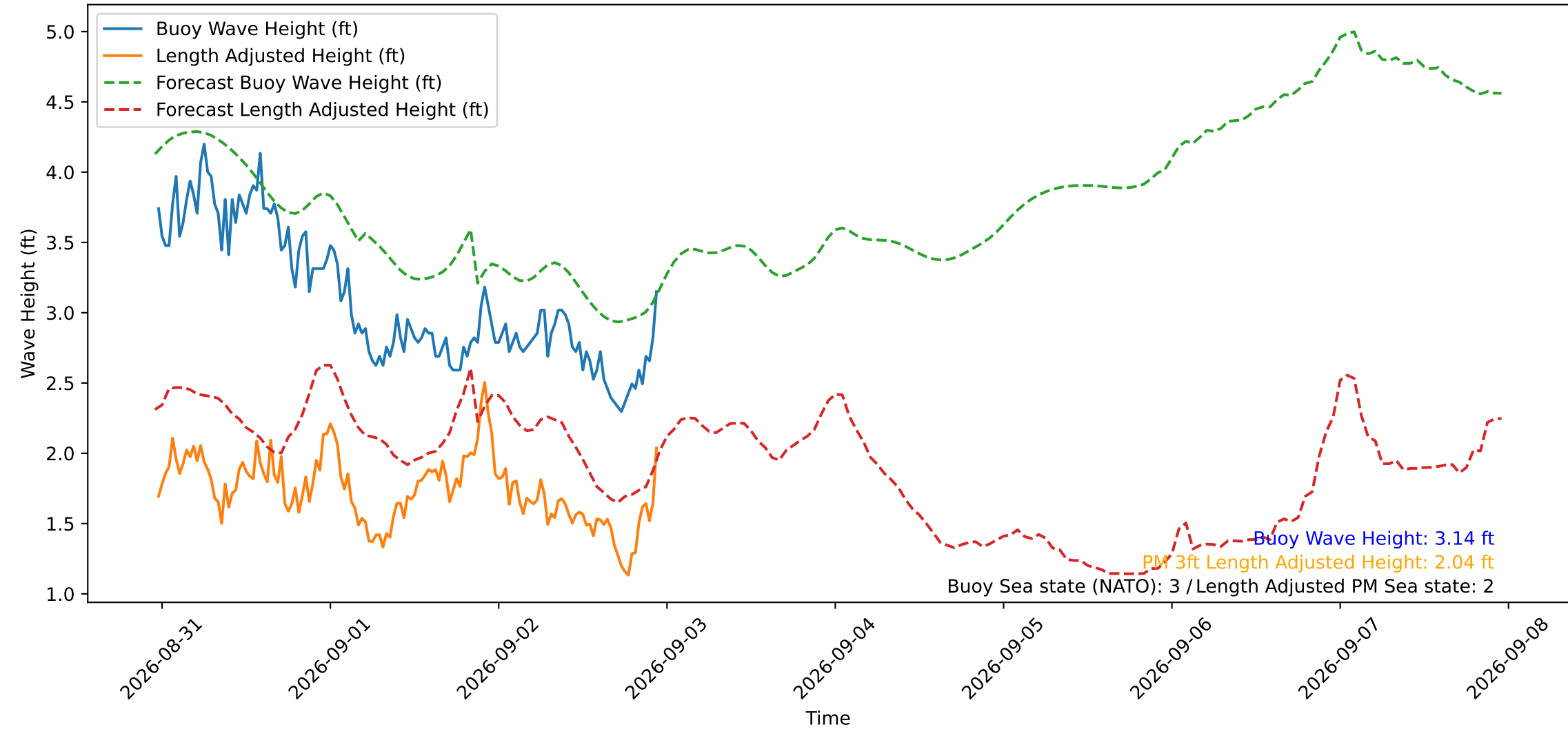
Wave Heights over Time for Red Beach at 2026-09-02 23:20:50
