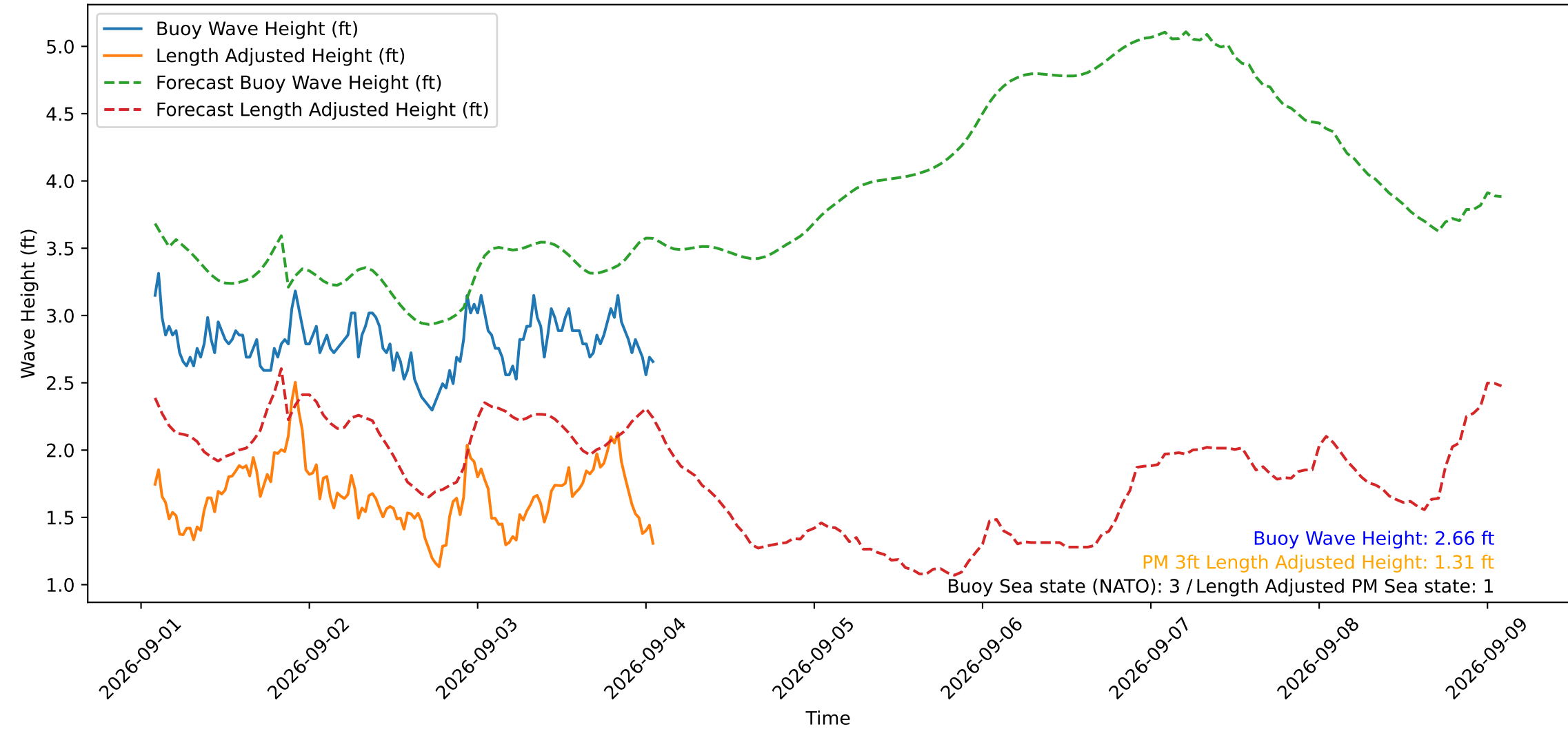
Wave Heights over Time for Red Beach at 2026-09-04 01:50:50
