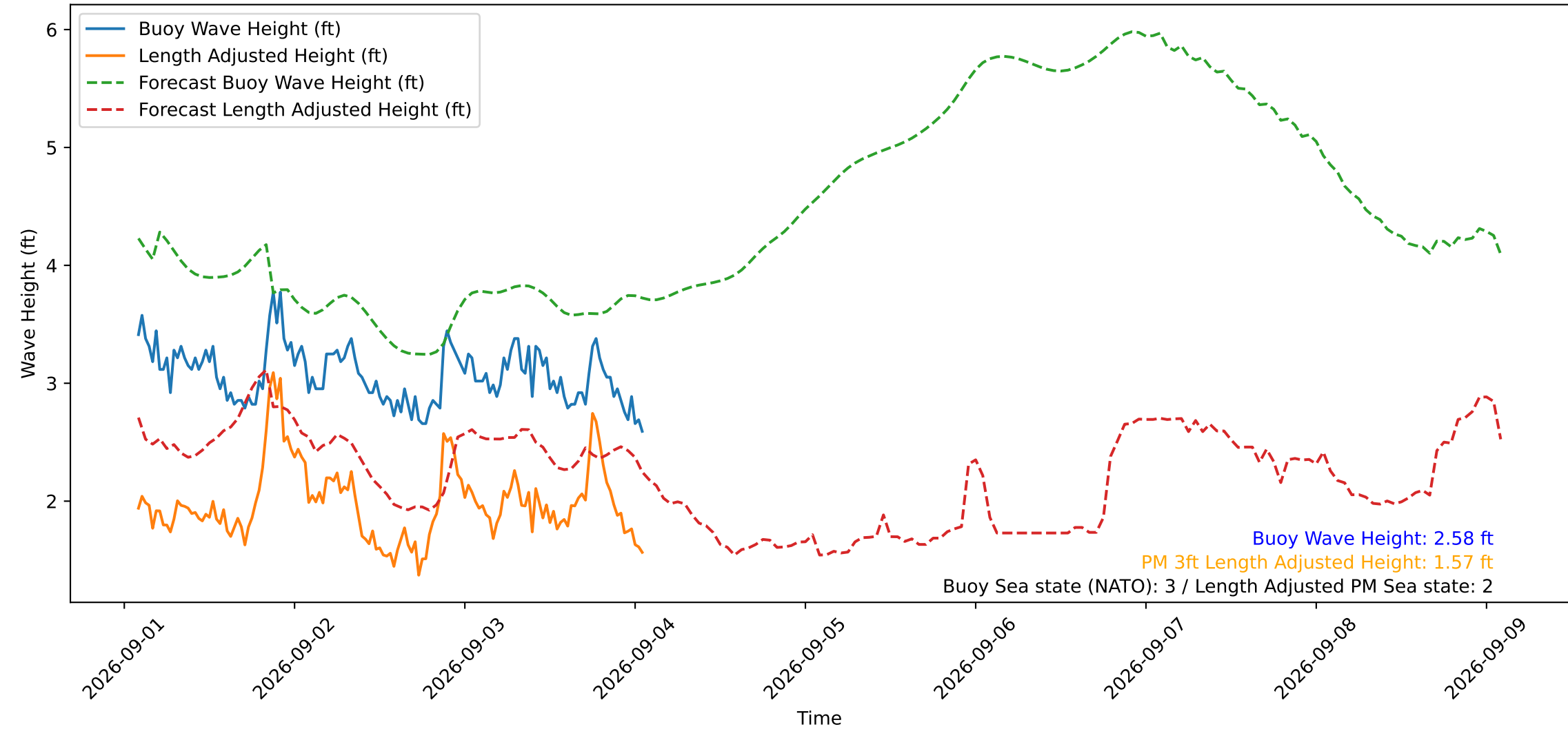
Wave Heights over Time for Green Beach at 2026-09-04 01:51:15
