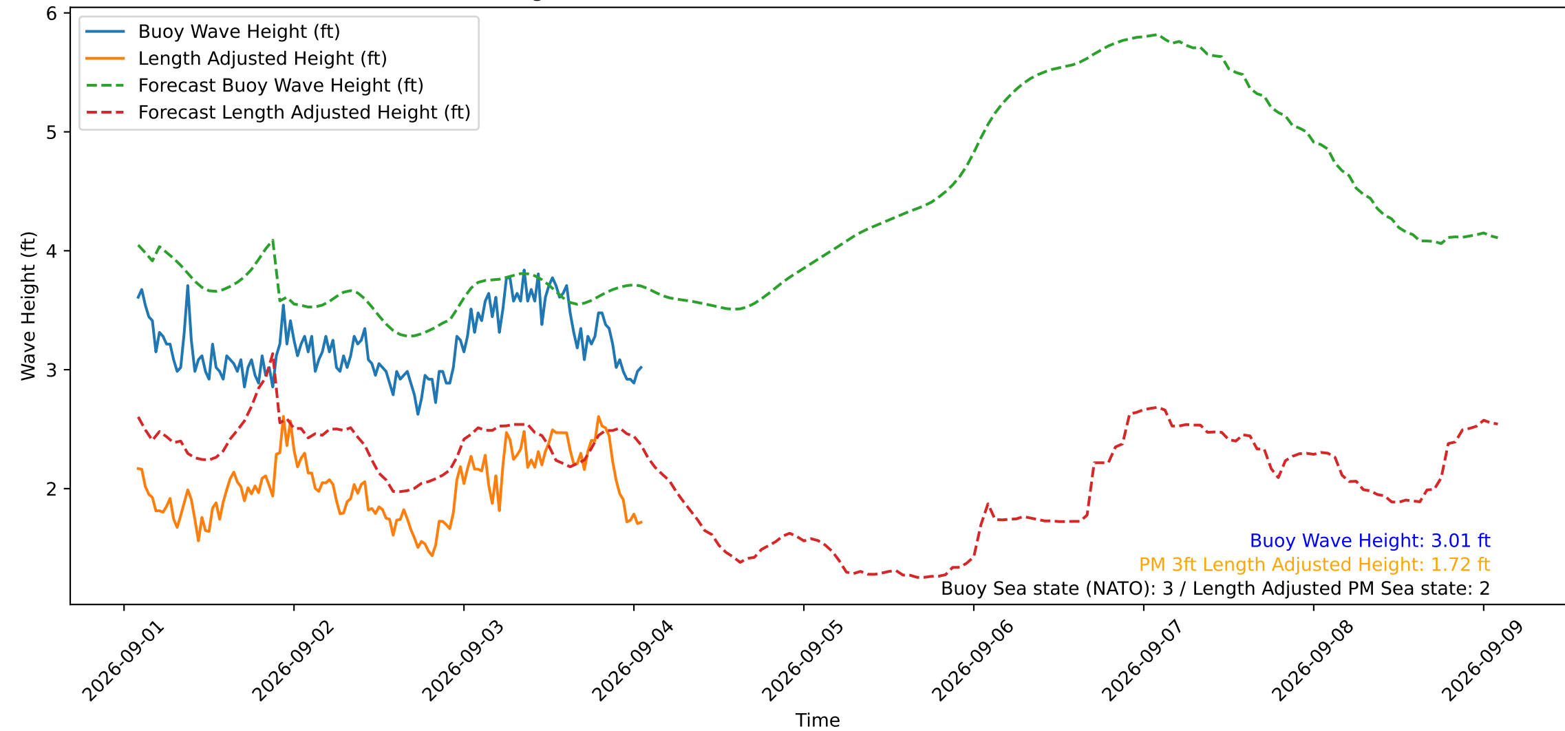
Wave Heights over Time for Oceanside Harbor at 2026-09-04 01:50:29
