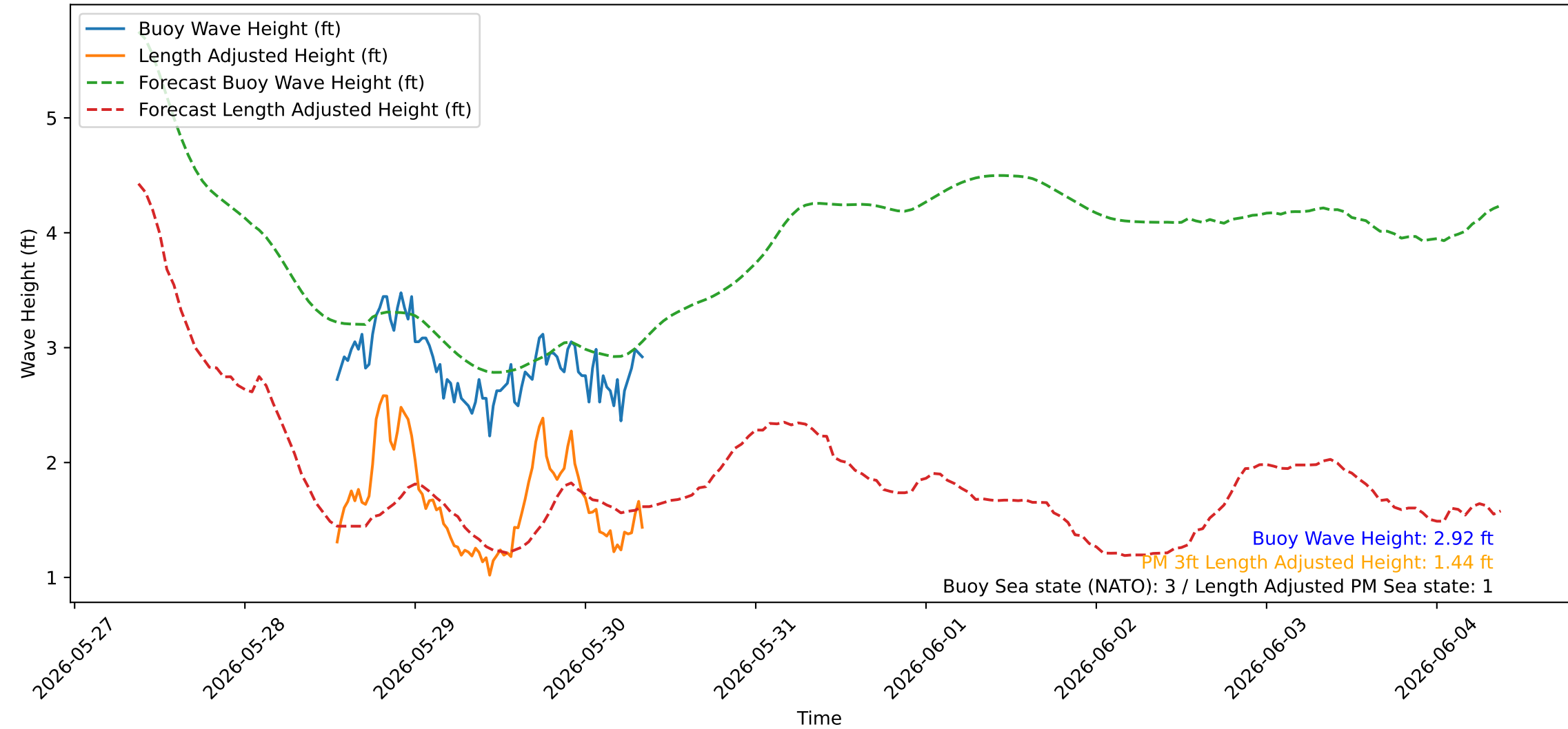
Wave Heights over Time for Oceanside Harbor at 2026-05-30 08:40:23
