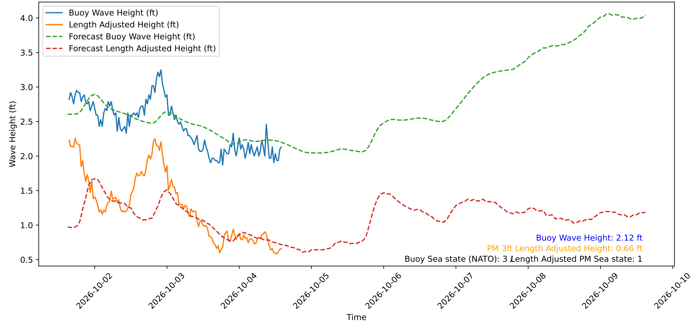
Wave Heights over Time for Red Beach at 2026-10-04 15:00:49
