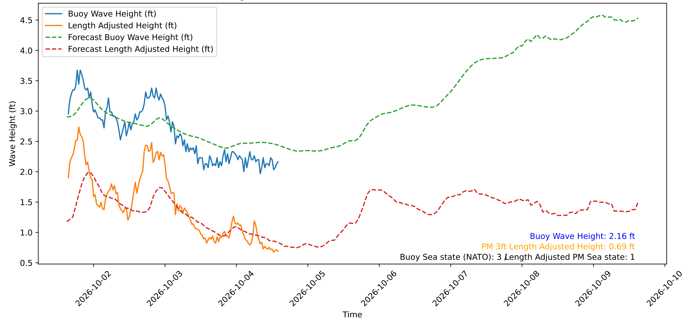
Wave Heights over Time for Green Beach at 2026-10-04 15:01:12
