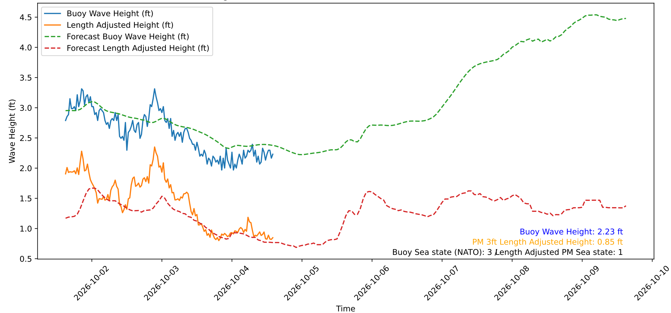
Wave Heights over Time for Oceanside Harbor at 2026-10-04 15:00:30
