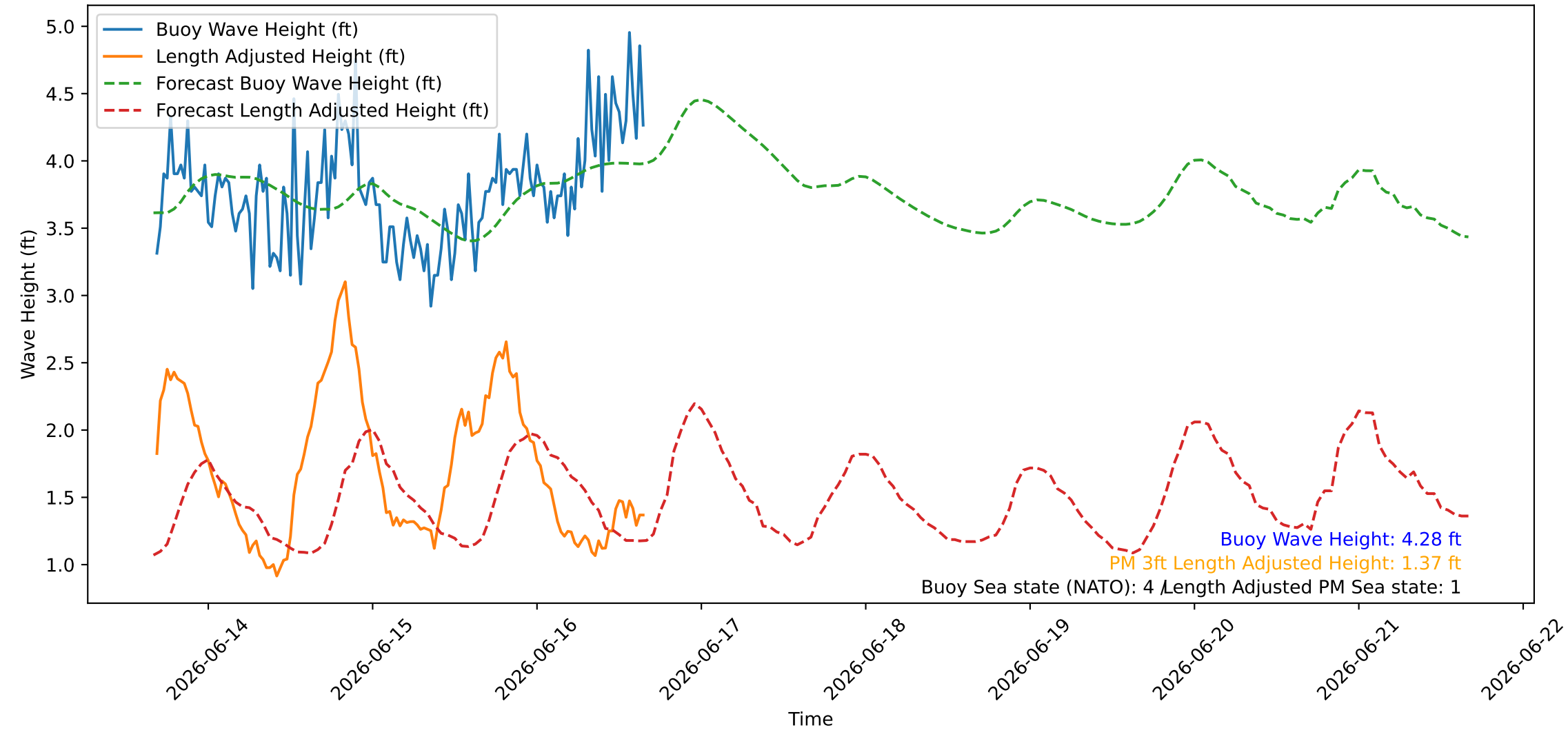
Wave Heights over Time for Red Beach at 2026-06-16 16:10:45
