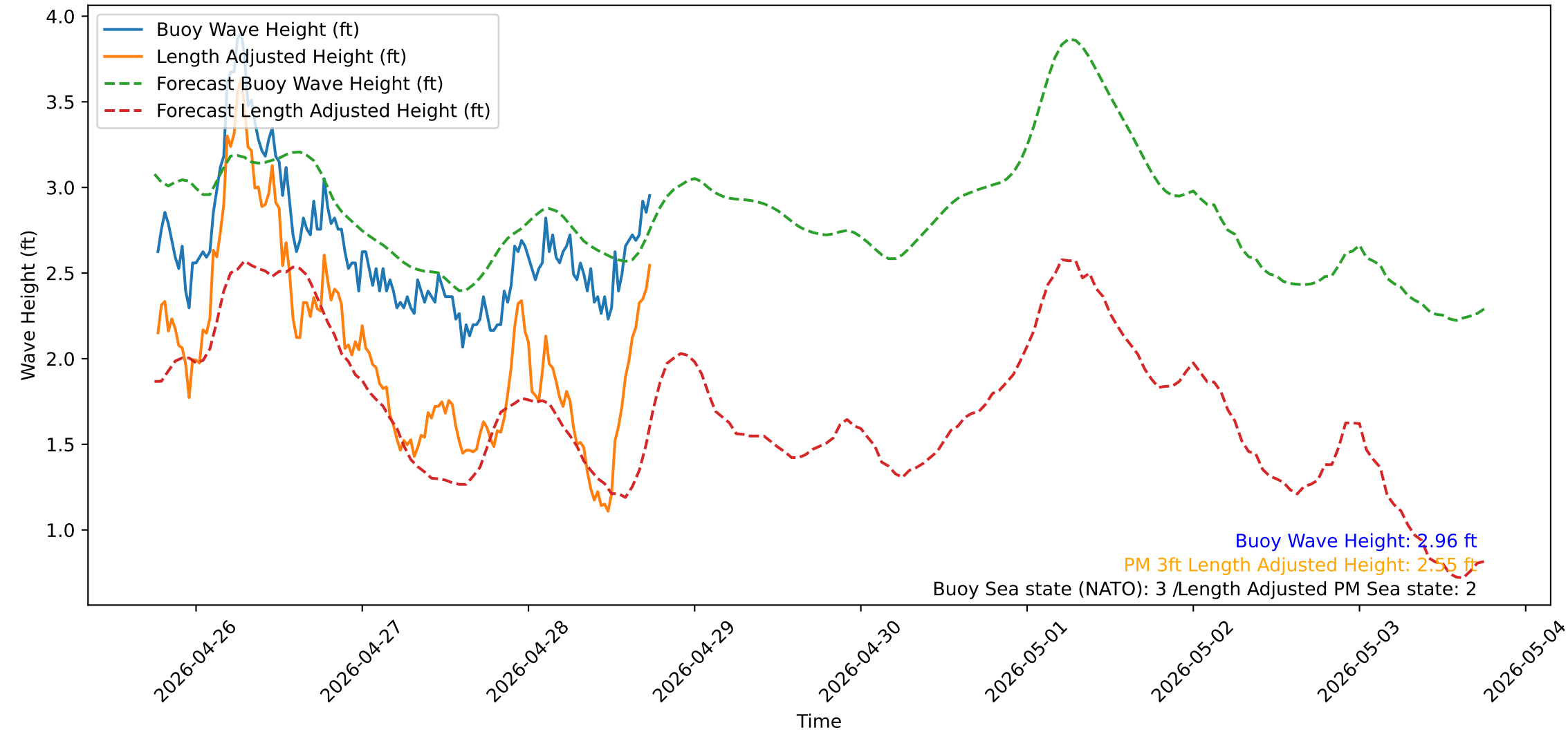
Wave Heights over Time for Oceanside Harbor at 2026-04-28 18:20:30
