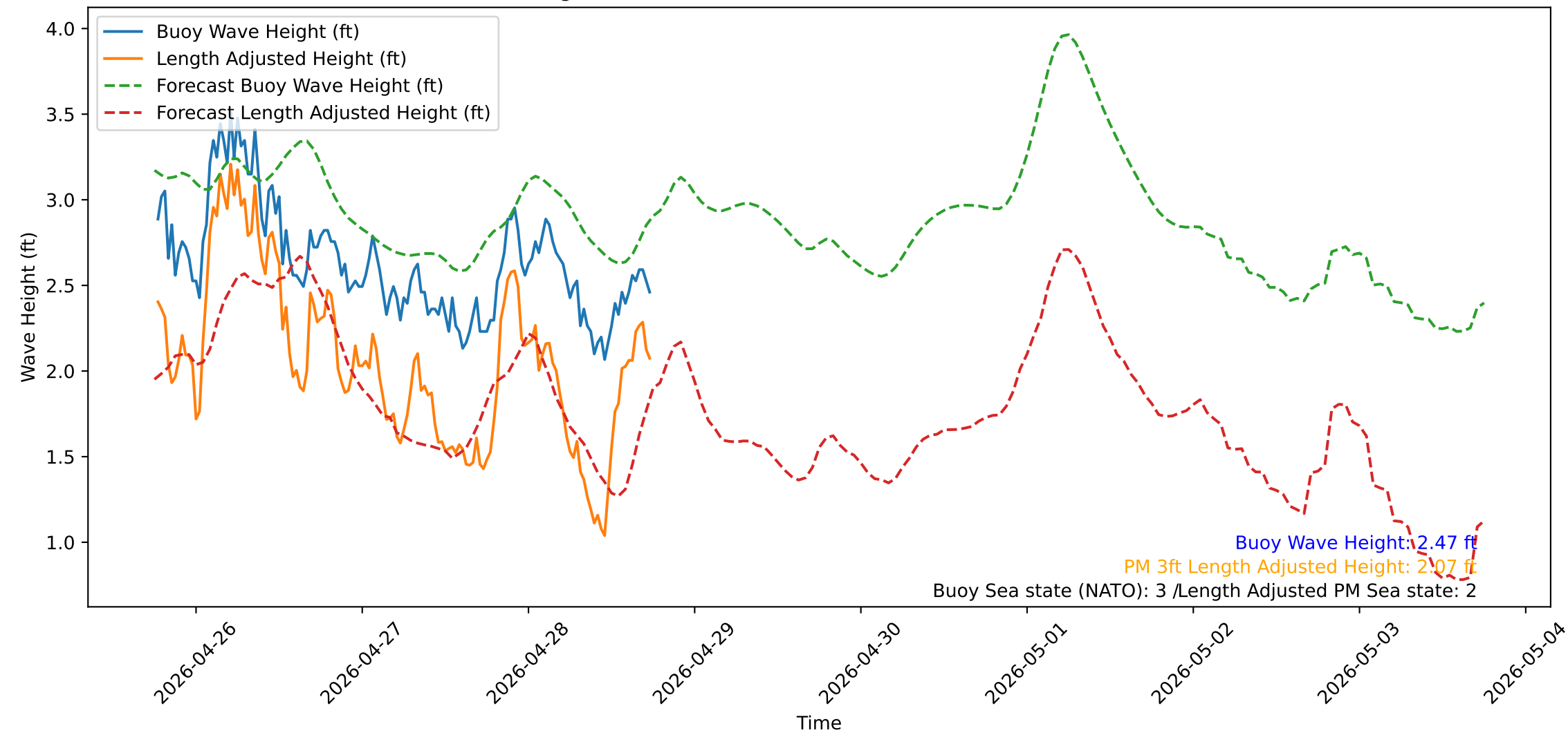
Wave Heights over Time for Green Beach at 2026-04-28 18:21:13
